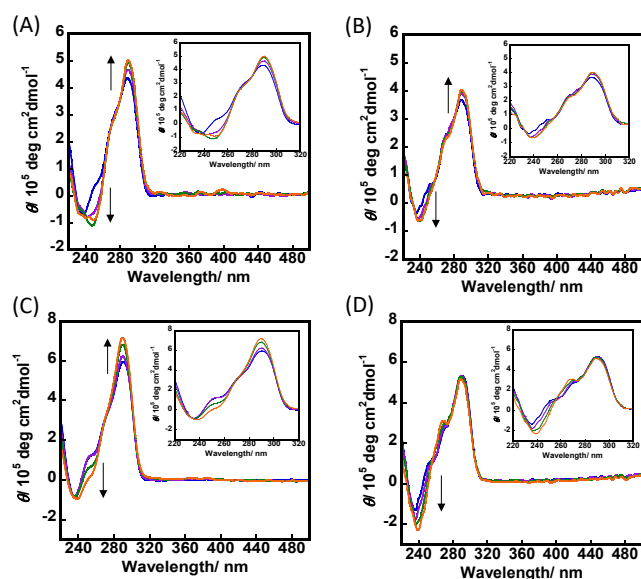
Figure 2. CD spectra analysis. G1 (1.5 \mu\text{M} ) with the presence of varying equivalents of 3 (A), and 5 (B); G2T1 (1.5 \mu\text{M} ) with the presence of 3 (C), and 5 (D). Buffer: 50 mM Tris-HCl (pH 7.4) and 100 mM KCl. Ligand vs. DNA: 0:1 (Blue); 1:1 (Purple); 2:1 (Green); 3:1 (Orange).
