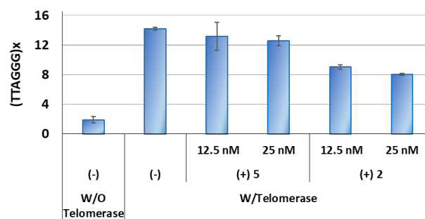
Figure 4. Telomere DNA elongation by telomerase was inhibited by 2 or 5 .
