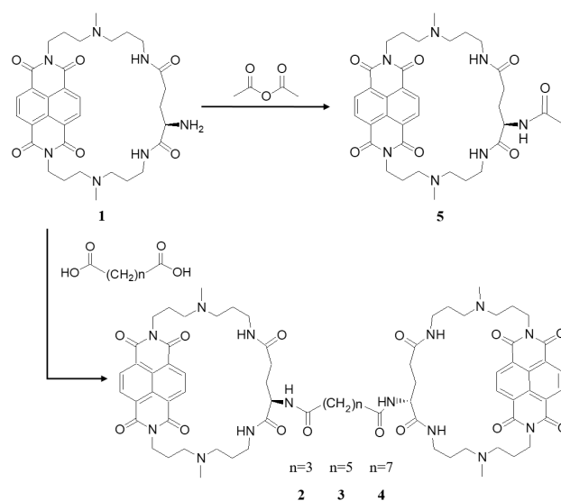
Figure 1. Chemical structures of monomeric cNDI ( 1 ), cNDI-dimers ( 2–4 ) with varied linker chain ( n=3, 5 , or 7 ) and cNDI modified acyl group ( 5 ).
