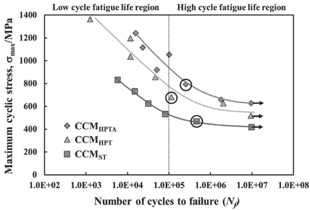
Fig. 4 S-N curves of CCM_{ST} , CCM_{HPT} , and CCM_{HPTA} .
