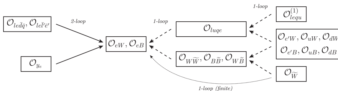
Figure 1. Corrections to the electron EDM (imaginary part of C_{eW,eB} ) induced up to the 2-loop level. The dashed and solid arrows denote mixing at 1-loop and 2-loop order respectively. On the right we list the operators that generate contributions enhanced by a double logarithm (showing the 1-loop mixing patterns that generate it), whereas on the left we list operators giving rise to a single logarithm.
