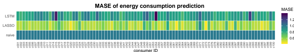
Figure 6. Heat map of MASE scores for the prediction of consumption values per consumer dataset. BLEMevaluateEnergyPreds (github.com/QuantLet/BLEM/tree/master/BLEMevaluateEnergyPreds)
