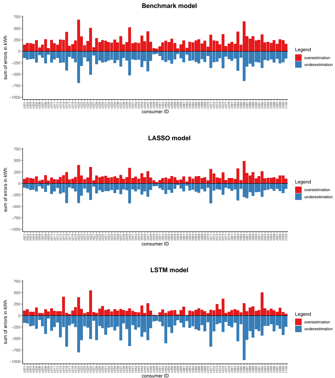
Figure 4. Sum of total over- and underestimation errors of energy consumption per consumer dataset and prediction model. BLEMplotPredErrors (github.com/QuantLet/BLEM/tree/master/BLEMplotPredErrors)
