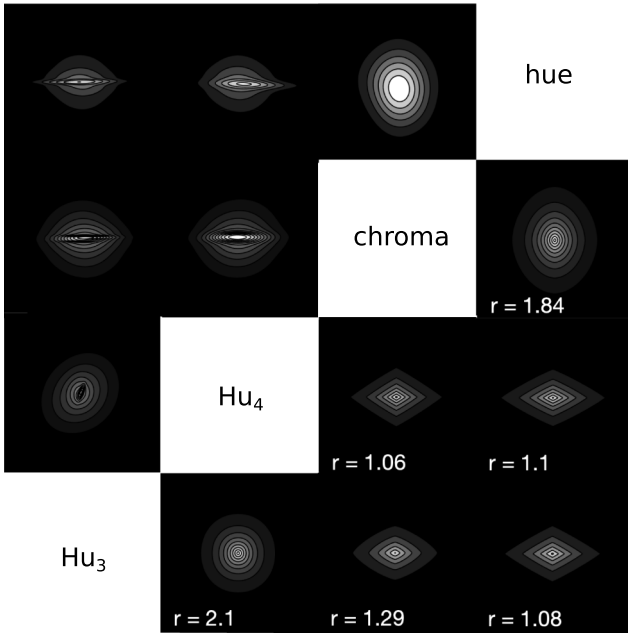
Figure 10 The Effect of Natural Image Statistic Training on the Rational Exclusively Family RESEMBLance Hierarchy’s Predictions for Between-Example Similarity
