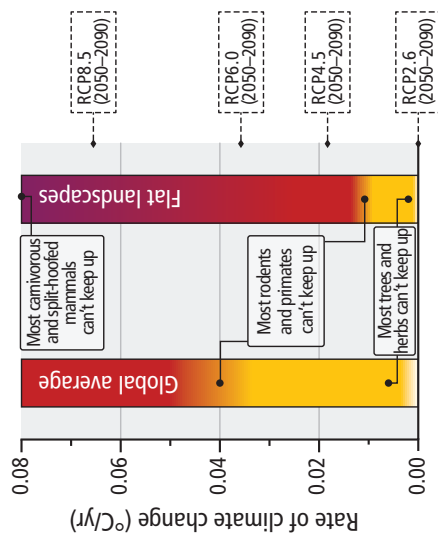
(a) Risk for terrestrial and freshwater species impacted by the rate of warming
