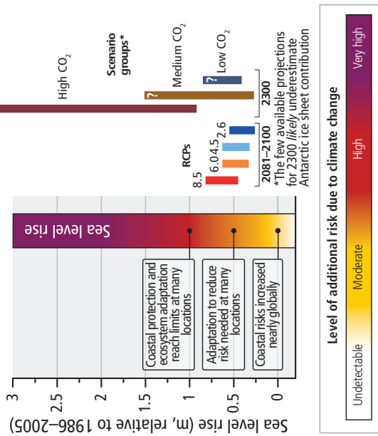
(c) Risk for coastal human and natural systems impacted by sea level rise
