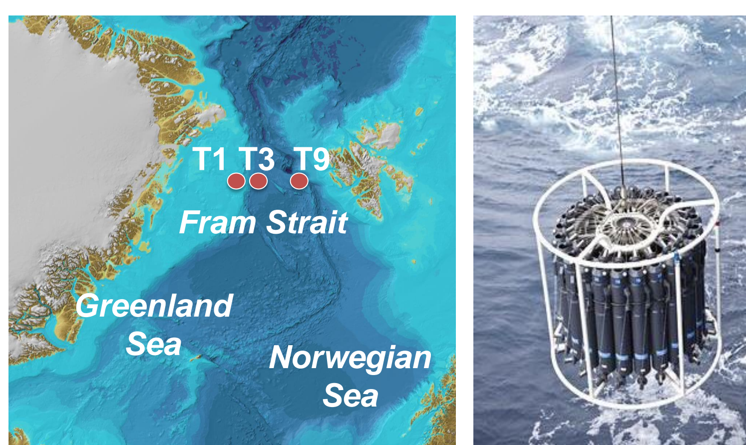
Position of samples. Base of map: http://www.ngdc.noaa.gov/mgg/bathymetry/arctic/
