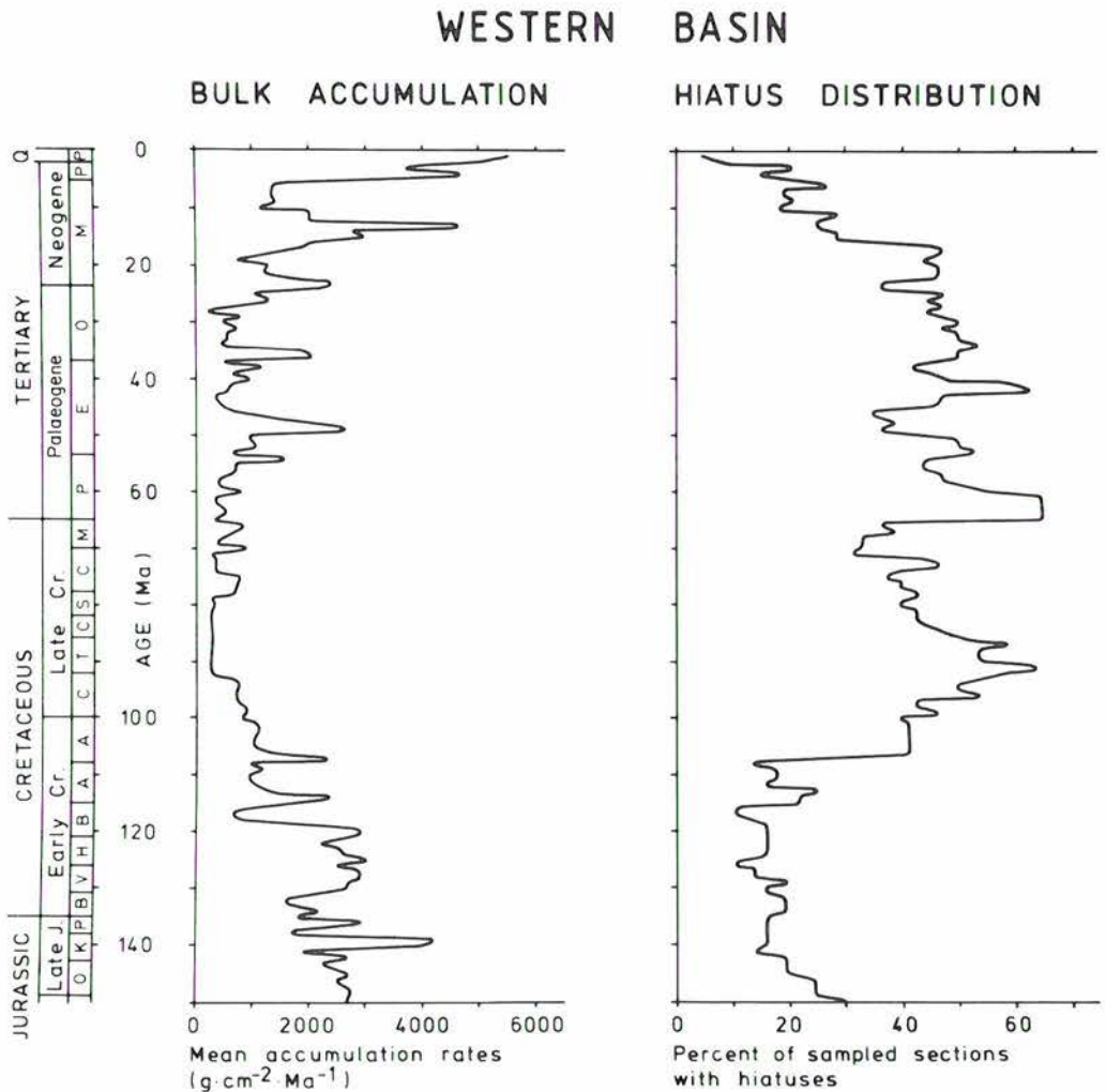
FIG. 7. Average bulk sediment accumulation rates and hiatus distributions versus time in the western sub-basin of the North Atlantic.
