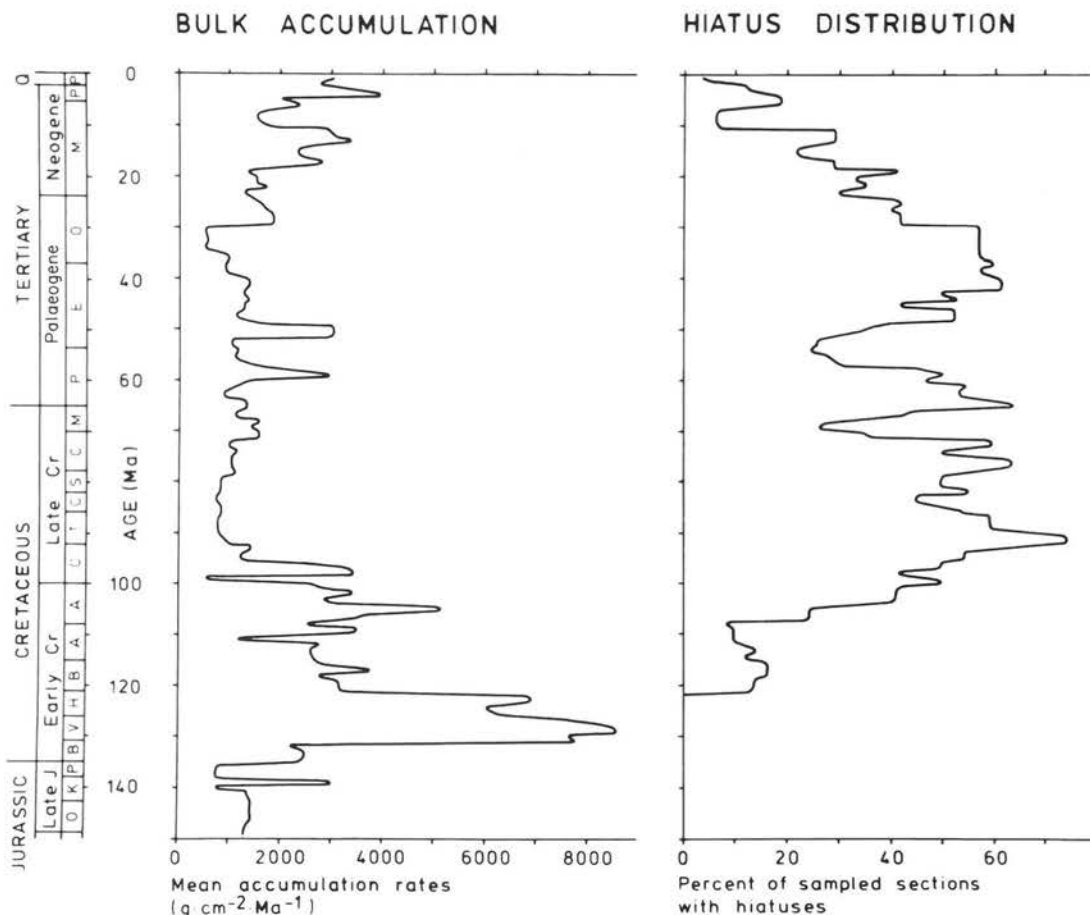
FIG. 8. Average bulk sediment accumulation rates and hiatus distribution versus time in the eastern sub-basin of the North Atlantic.
