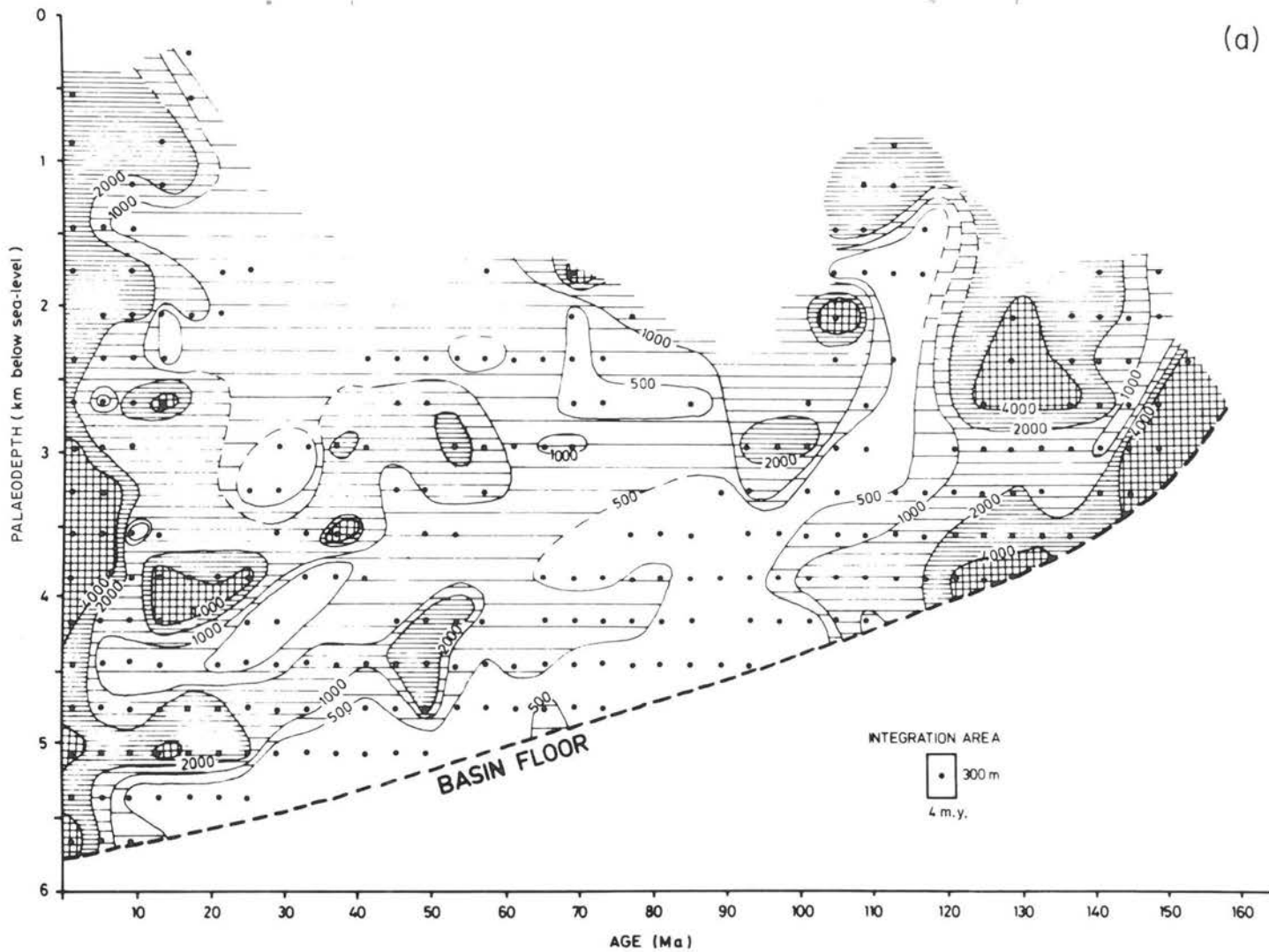
FIG. 5. Accumulation rates ( \text{g cm}^{-2}\text{Ma}^{-1} ) of bulk sediment plotted versus age and palaeodepth for (a) the western, and (b) the eastern basins of the North Atlantic Ocean.
