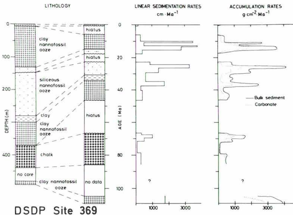
FIG. 3. Graphical example of the authors' data processing: the left column provides the lithostratigraphic information (simplified), as found in the Initial Reports of the Deep-Sea Drilling Project; in the second column lithology is plotted versus age. By correcting linear sedimentation rates for compaction the accumulation rates for every million year time interval have been calculated.
