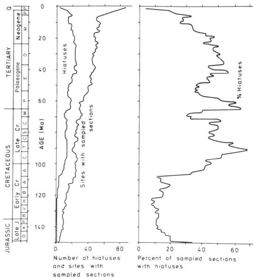
FIG. 6. Distribution of hiatuses in the North Atlantic deep-sea drill sites. Hiatus distributions are given in absolute and relative figures.
