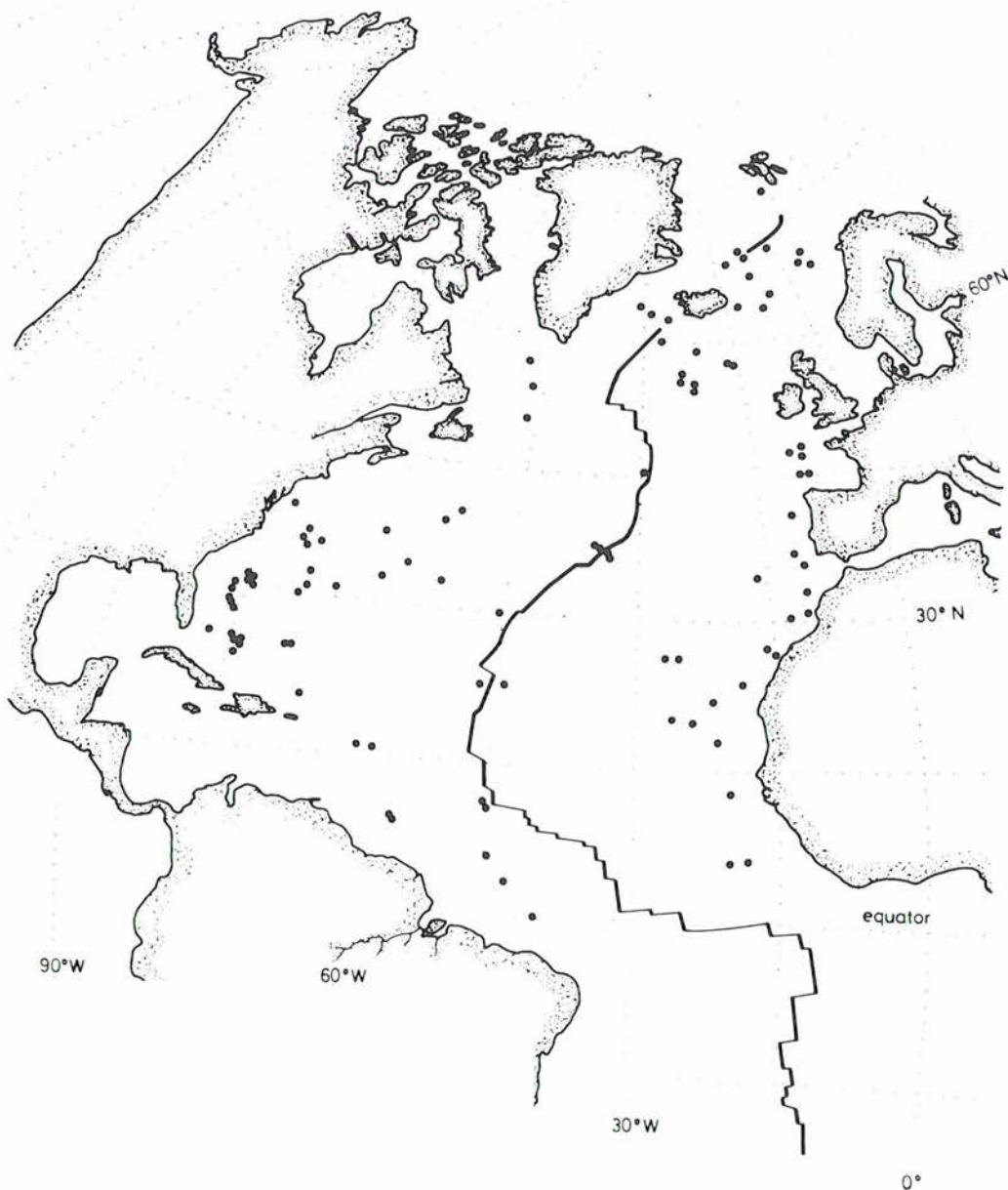
FIG. 1. Distribution of Deep-Sea Drilling Project drill sites analysed for this study.
