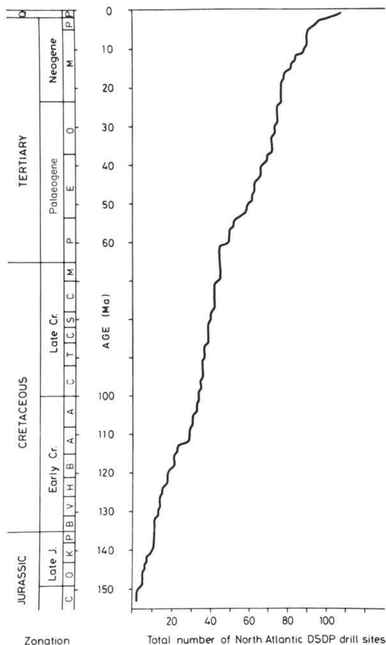
FIG. 2. Temporal coverage of all DSDP sites in the North Atlantic Ocean (including the Norwegian-Greenland Sea). The absolute time-scale (in Ma) is based on available biostratigraphic zonations (van Hinte 1976, 1978; van Couvering & Berggren 1977; Berggren et al. 1978); absolute ages of stratigraphic boundaries as used in this study are indicated in this figure.
