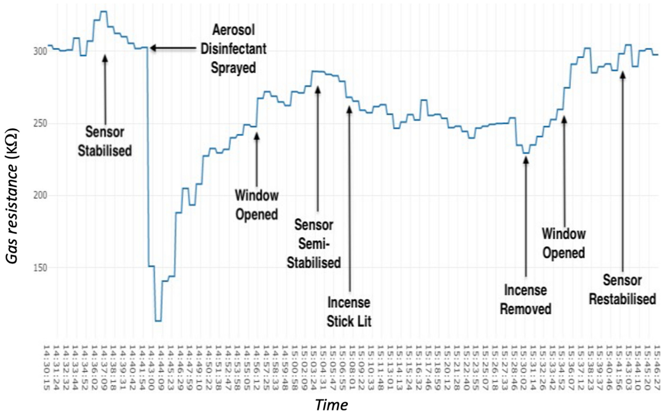
Fig. 6. Controlled experiment: effect of disinfectant and incense (gas resistance against time).
