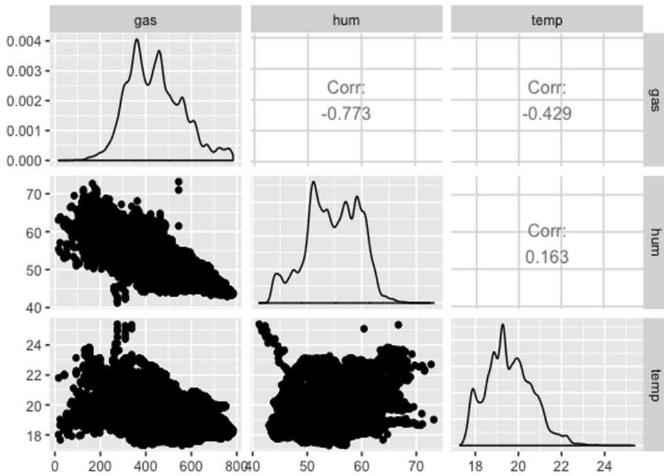
Fig. 12. Indoor air quality kitchen (autumn).
