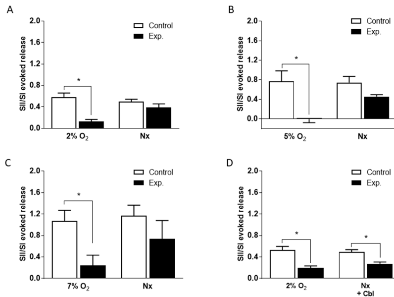
Figure 3. Mean effects of 300 \mu M Cbl on the ratio of the second and first 3 H-CA responses to hypoxia shown in Figure 2. Results were calculated separately for 3 H-CA release during hypoxia and during the subsequent 20 min of normoxia (Nx) during which release fell back to the baseline. (A)–(C) Mean effects of Cbl on the ratio of the second and first responses to hypoxia for 2, 5, and 7% O 2 ; Cbl was present for 10 min before and during the second hypoxic period. (D) Mean effects of Cbl on the ratio of the second and first responses to hypoxia for 2% O 2 ; Cbl was present for 10 min before and during the second hypoxic period, as well as during the subsequent 20 min of normoxia. Asterisks indicate where there was a significant effect of Cbl. Number of replicates for each condition as is indicated in Figure 2.
