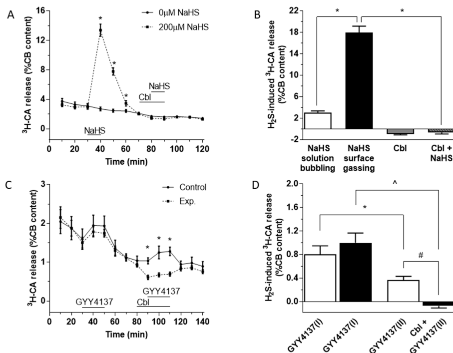
Figure 1. Effect of NaHS and GYY4137 on the release of ^3\text{H} -CA by CB chemoreceptor cells in the presence and absence of Cbl. (A) Time course of catecholamine release elicited by 200 \mu\text{M} NaHS applied for 10 min. A second application of NaHS was in the presence of 300 \mu\text{M} Cbl ( n = 6 and 8, for 0 and 200 \mu\text{M} NaHS, respectively). (B) The black bar shows the magnitude of the release response corresponding to the area under the curve in part A. The empty bar represents the release response obtained for 200 \mu\text{M} NaHS in similar experiments in which the solution rather than the headspace was gassed. The small columns in grey at the right of the figure show that 300 \mu\text{M} Cbl abolished the effect of NaHS, and that when applied alone Cbl caused a modest inhibition of the basal ongoing release of catecholamine (NaHS solution bubbling, n = 2 ; NaHS gassing surface, n = 8 ; Cbl, n = 18 ; Cbl + NaHS, n = 10 ). (C) Effect of GYY4137 on the release of ^3\text{H} -CA in the absence and presence of Cbl. 400 \mu\text{M} GYY4137 was applied for 20 min by itself at 30 and 90 min (continuous line); 400 \mu\text{M} GYY4137 was applied for 20 min by itself at 30 min and then again at 90 min, this time in the presence of 300 \mu\text{M} Cbl, which had been applied at 80 min (dashed line). n = 10 in each condition. (D) The bars show the amplitudes of the two successive responses to GYY4137 (area under the curve) when both responses were evoked in the absence of Cbl (empty bars) and when the second response was elicited in the presence of Cbl. Symbols indicate where there was a significant effect.
