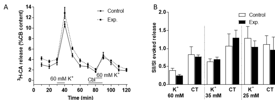
Figure 4. Effects of Cbl on the 3 H-CA release response elicited by three elevated levels of extracellular K + . (A) The continuous line in shows the effects on catecholamine release of successive exposures of CBs (at 30–40 min, SI, and 80–90 min, SII) to 60 mM K + (n = 5 in each condition) under control conditions, whereas the dashed lines illustrate catecholamine release evoked by a similar protocol when 300 \mu M OH-Cbl was present between 70 and 90 min. (B) Bars illustrate the ratio of the second and first responses to high K + in the presence and absence of Cbl during the 10 min of high K + and during the subsequent 20 min period in control Tyrode (CT) solution (K + 5mM) during which catecholamine release remained elevated with 60, 35, and 25 mM (n = 5 in each condition).
