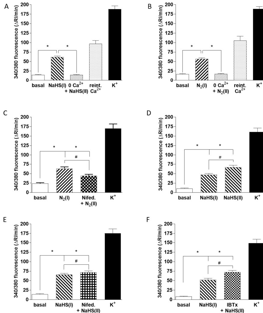
Figure 6. Mechanisms of \text{Ca}^{2+} influx induced by hypoxia and 50 \mu\text{M} NaHS. [\text{Ca}^{2+}]_i was assessed as the F340/F380 fluorescence emission ratio in isolated chemoreceptor cells loaded with fura-2. In all cases the protocols followed the same pattern: a first exposure to hypoxia or NaHS, subsequent application of the experimental condition 0 mM \text{Ca}^{2+} (1 min, A,B ), 2 \mu\text{M} nifedipine (3 min, C and E ), or 100 nM IBTx (1 min, F ) followed by that condition with hypoxia or NaHS and finally high \text{K}^+ to demonstrate that cells were viable. Bars in all panels indicated the running integrals of the fluorescence signals ( \Delta fluorescence/min) obtained during the various conditions. ( A ) Effect of \text{Ca}^{2+} free solution on the \text{Ca}^{2+} signal caused by NaHS ( n = 66 cells). ( B ) Effect of \text{Ca}^{2+} free solution on the \text{Ca}^{2+} signal evoked by hypoxia ( n = 44 cells). In both cases, \text{Ca}^{2+} reintroduction caused a rebound increase in the fluorescence emission ratio. ( C ) Effect of nifedipine on the \text{Ca}^{2+} signal elicited by hypoxia ( n = 24 cells). ( D ) \text{Ca}^{2+} signals evoked by two successive exposures of cells to NaHS under control conditions, data from 51 cells. ( E ) \text{Ca}^{2+} signals evoked by two successive exposures of cells to NaHS—the first under control conditions and the second in the presence of nifedipine ( n = 50 cells). ( F ) \text{Ca}^{2+} signals evoked by two successive exposures of cells to NaHS; the first under control conditions and the second in the presence of IBTx ( n = 47 cells). Symbols connote significant differences between the columns indicated.
