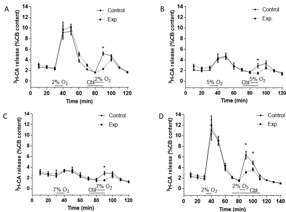
Figure 2. Effects of Cbl on ^3\text{H-CA} release response elicited by different levels of hypoxia. The continuous lines in (A), (B), and (C) show the effects on catecholamine release of successive exposures of CBs (at 40–50 min, SI, and 80–90 min, SII) to 2% \text{O}_2 (A, n = 12 in each group), 5% \text{O}_2 (B, n = 5 in each group), and 7% \text{O}_2 (C, n = 5 in each group) under control conditions, whereas the dashed lines illustrate catecholamine release evoked by a similar protocol when 300 \mu\text{M} Cbl was present between 70 and 90 min. (D). Protocol similar to panels A except that Cbl was present both during and after the second hypoxic challenge (from 70 to 110 min), n = 8 and 12, control and experimental group, respectively. Asterisks connote time points where there were significant differences between the amplitudes of ^3\text{H-CA} release observed in CBs which were exposed or not exposed to Cbl.
