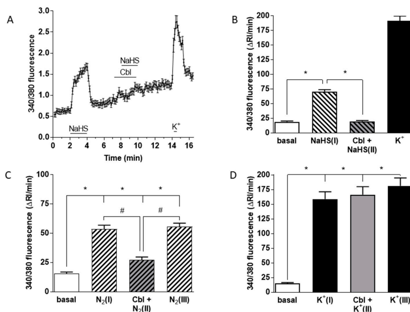
Figure 5. Effects of Cbl on the intracellular Ca 2+ responses elicited by 50 μM NaHS, hypoxia, and high external K + . [Ca 2+ ] i was assessed as the F340/F380 fluorescence emission ratio in isolated chemoreceptor cells loaded with fura-2. (A) Mean +/− SEM 340/380 fluorescence ratio (calculated every 8 s) from 74 cells stimulated with NaHS in the absence and presence of 300 μM Cbl. The response to high K + at the end demonstrates cell viability. The fast Ca 2+ transient in response to high K + at the end of experiments demonstrates that cell was viable. (B) Mean running integrals of the basal and stimulated fluorescence signals (Δ fluorescence/min) obtained from the 74 chemoreceptor cells recorded as in (A). (C) Mean running integrals of the fluorescence signals obtained in 43 cells recorded following the sequence depicted in the figure consisting of the application of three identical hypoxic stimuli (perfusion with 5% CO 2 /95% N 2 ) except that the middle hypoxic challenge was applied in the presence of 300 μM Cbl. (D) Mean values obtained in 44 cells in a similar ‘sandwich’ style experiment using high (35 mM) external K + as the stimulus. Symbols connote significant differences between the columns indicated.
