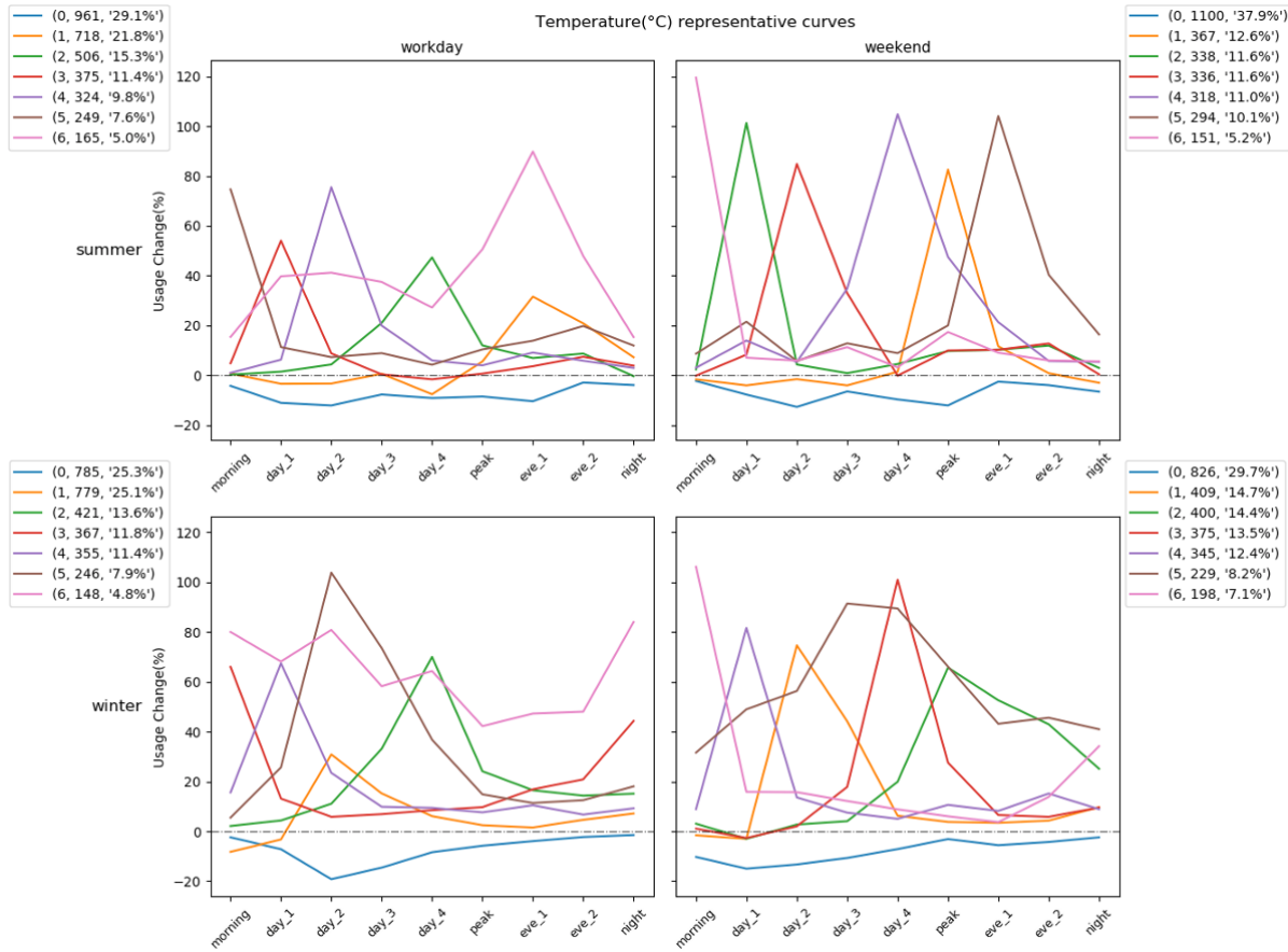
Fig. 3 Temperature sensitivity
