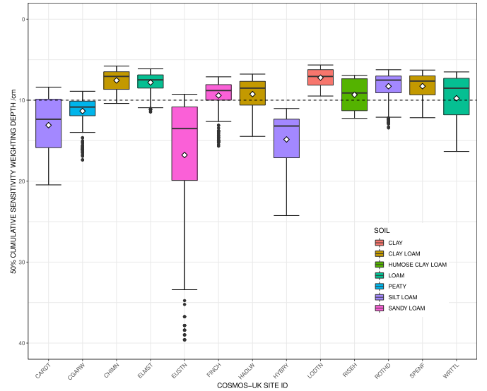
Fig. 3. Boxplot representing the variation in the 50% cumulative sensitivity depth d_{50} (weighted by radius) during 2018 at the COSMOS-UK sites used in this study. The whiskers define the extremes of the data, the thick bars the median, and the box ends represent the first and third quartile values. The mean for each site is plotted as the white diamond. The box colors represent the site soil classification for the surface layer.
