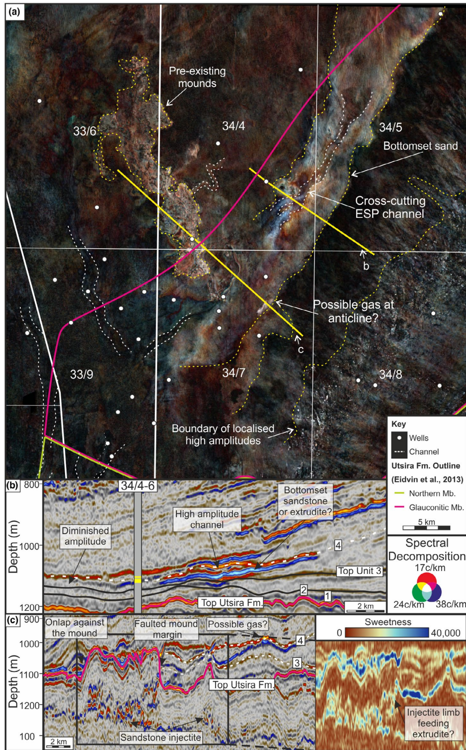
FIGURE 12 Sandstone connectivity between the ESP and NM systems. (a) Frequency decomposition of the Top Unit 4 surface, showing the bottomset sandstones from the NM clinoforms being cross-cut by channels from the ESP, promoting connectivity. (b) Seismic dip section to show the bottomset sandstone in Unit 4, being cross-cut by the possibly sand-filled channel from the ESP. (c) Seismic dip section highlighting the interaction of the sandstone with the mounds (possibly faulted margins) and sand injectite limb. Inset shows the sweetness of Unit 4 sandstone which is possibly sourced from the underlying injectite. Sweetness colour bar from Crameri (2021). Location of 'a' shown in Figure 5
