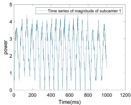
Figure 6: Original CSI stream on a subcarrier
