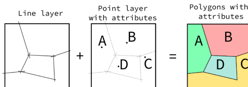
Figure A2.1: Generation of a consistent polygonal layer by polygonize operation, this can be performed by any GIS and is suggested as a good practice in geological map generation. A line layer is used for tracing the contacts between the different units and a point layer is also needed to define attributes for the polygons.
