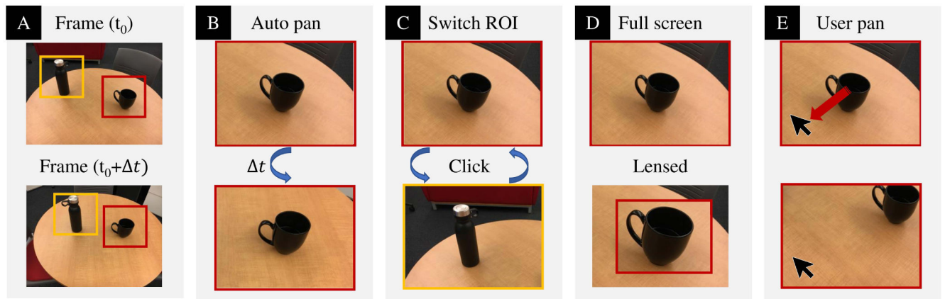
Figure 4: Interface design space for SViM magnifier. (A) shows two frames of a video with two salient ROIs enclosed by red and yellow squares; the top and bottom frames have time stamps t_0 t_0 + t respectively. (B) shows assistive panning following the ROIs through time by automatically panning the viewport to the ROIs. Specifically, observe that assistive panning has tracked the ROI enclosed in red square through time ranging from t_0 through t_0 + t and panned the viewport to this ROI at t_0 + t . (C) shows switching between ROIs with mouse clicks - the ROI in the red square is switched to the ROI in the yellow square. (D) shows the display modes, the full screen mode (on top) populates the entire screen to show magnified content whereas in the lensed mode (bottom) the ROI is magnified (such as the one in the red square) overlaying the rest of the content unmagnified. (E) shows that the user moves the mouse to pan to any location.
