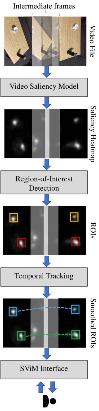
Figure 2: The SViM video magnification pipeline. The process begins with a sequence of RGB frames. Video saliency model predicts saliency in the form of a heatmap. Next, the ROI detector produces a set of bounding boxes identifying ROIs. This is followed by temporal tracking, which smooths the trajectory of ROIs across the frames. The result of this process is then passed to the SViM interface, which displays the magnified ROIs to the user in the magnifier viewport.
