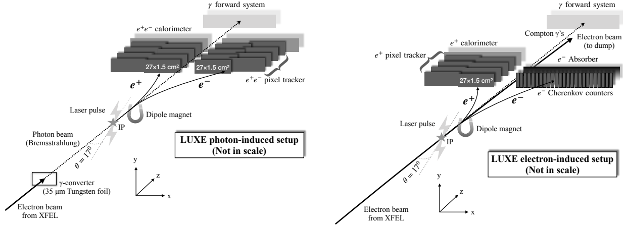
Figure 23. Schematic of the detector system to measure e^+e^- pairs produced at the IP for the (left) \gamma_B -laser and (right) e^- -laser setup. In both cases, the electrons and positrons are separated by a dipole magnet. In the \gamma_B -laser setup, electrons and positrons are measured in a detector system consisting of tracking planes and calorimeters, where the electron and positron detector systems are identical. In the e^- -laser setup, electrons and positrons are measured in a detector system consisting of tracking planes and a calorimeter for the positrons and Cherenkov counters for the electrons. Photons continue to the forward system, which is discussed in Section 5.2.3.
