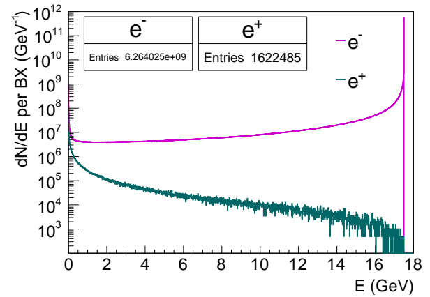
Figure 20. Energy spectra of electrons and positrons observed in the simulation with a tungsten target of 35 \mu\text{m} ( 1\%X_0 ) thickness for one bunch crossing. The electron spectrum also includes electrons from the beam which did not interact with the converter.
