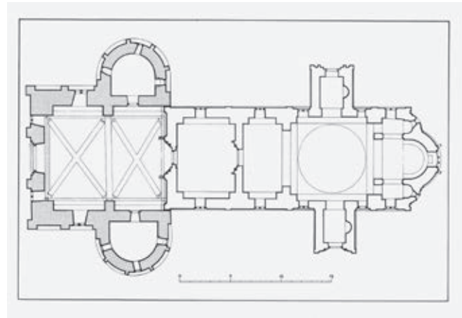
Fig. 154. Studenica monastery, Church of the Mother of God, ground plan
