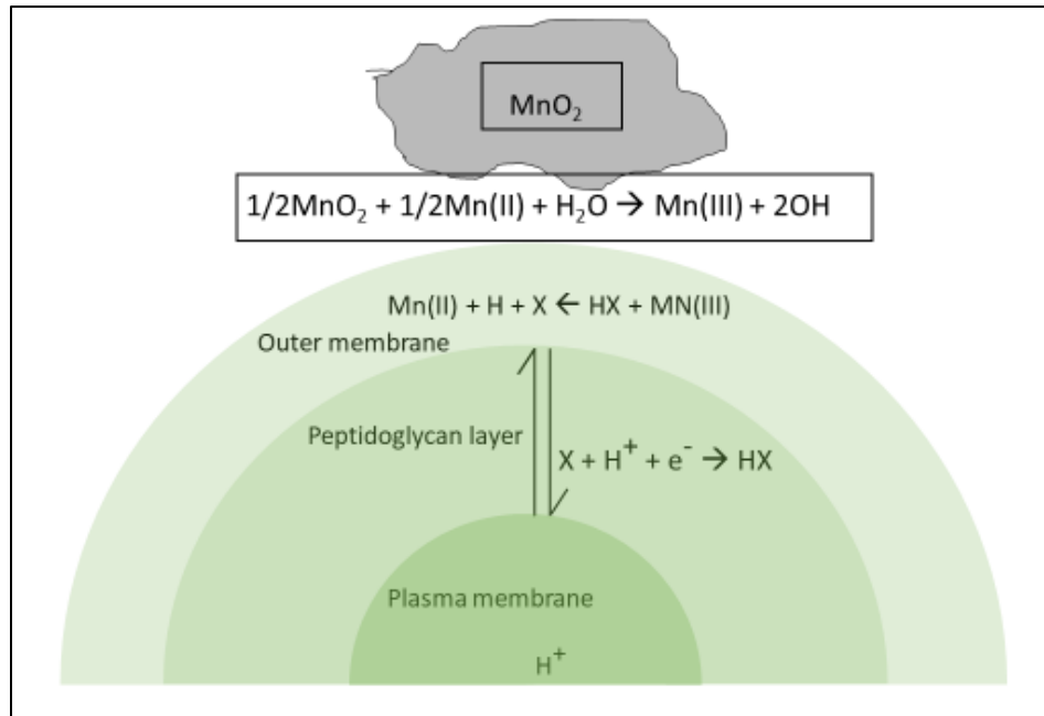
Figure 2. A model explaining the transfer of electrons across the interface between a bacterial cell surface and MnO 2 . Source: https://doi.org/10.1016/j.chemosphere.2016.04.028 after [26].
