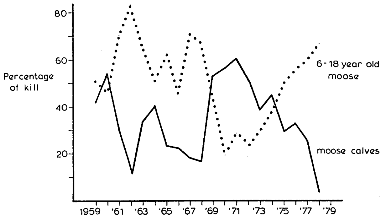
Figure 3. Annual proportion of calves and 6-18 year-old moose among wolf-kills.
