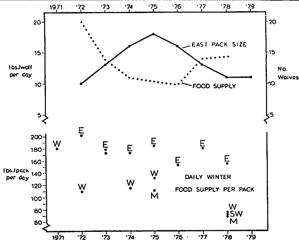
Figure 8. Upper graph: East Pack size and food availability per wolf, 1972-79. Lower graph: Predation rate as indicated by food availability per pack. E=East Pack, W=West Pack, M=Middle Pack, SW=Southwest Pack.
