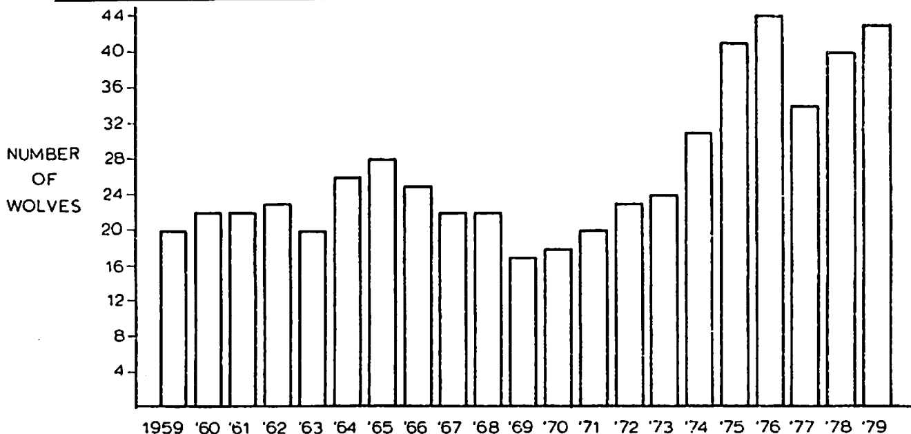
Figure 5. Isle Royale wolf population levels in midwinter, 1959-79.
