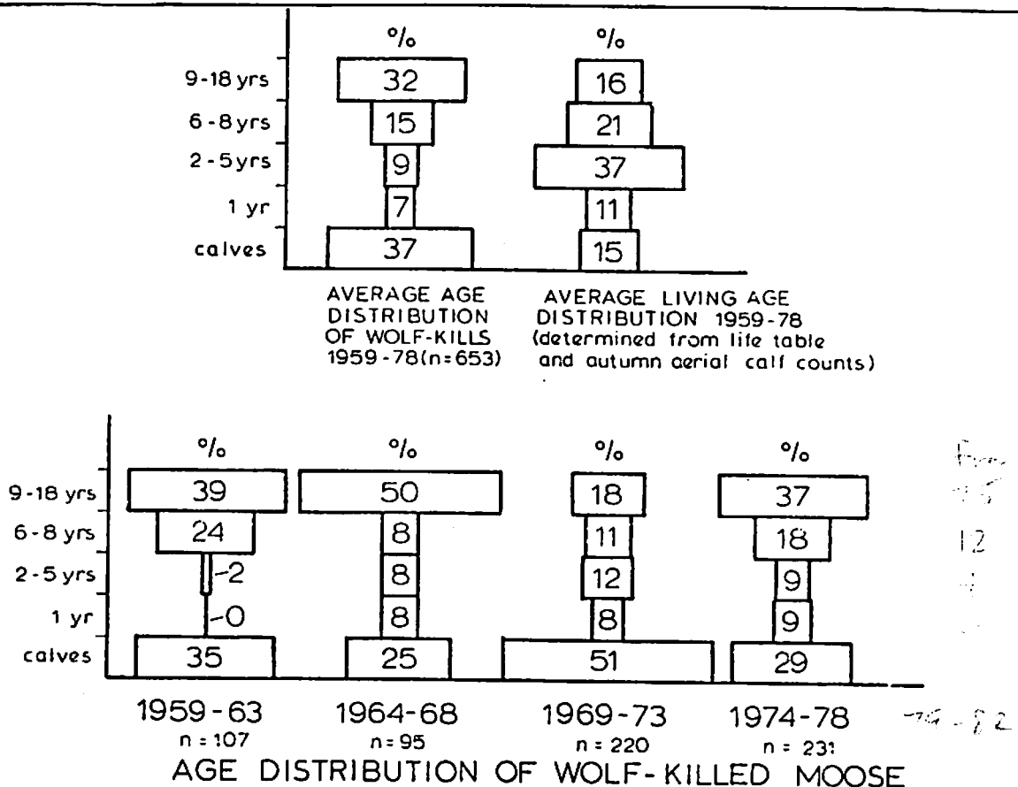
Figure 4. Upper graph: Long-term average age distribution of wolf-killed moose compared to living age distribution. Lower graph: Age distribution of wolf-killed moose sorted by five-year intervals.
