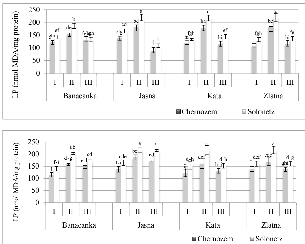
Figure 4. The LP intensity in the leaves (top) and roots (bottom) of selected genotypes of oilseed rape grown on chernozem and solonetz in various development stages.
