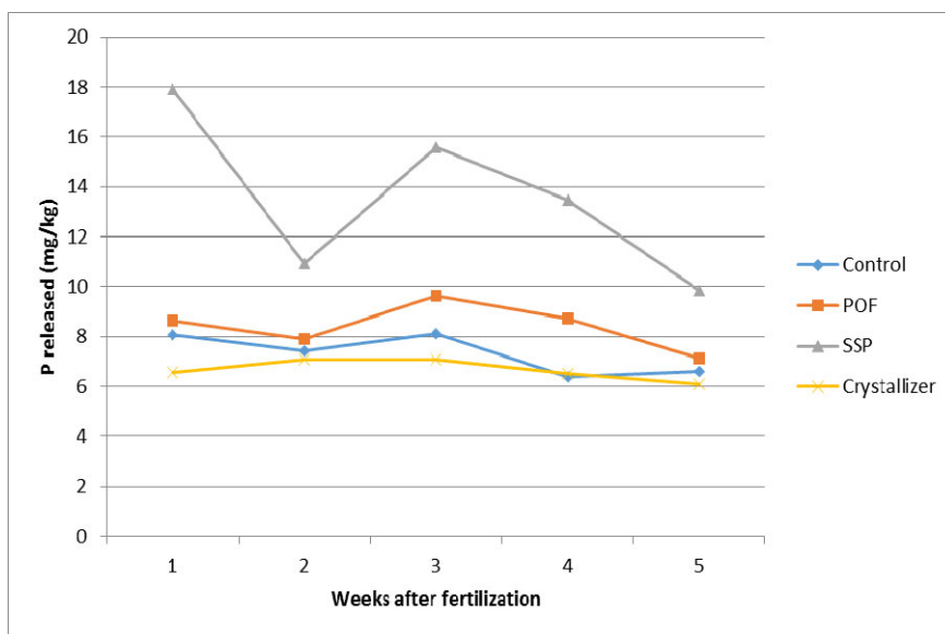
Figure 1 - Kinetics of phosphorus release in the soil used
