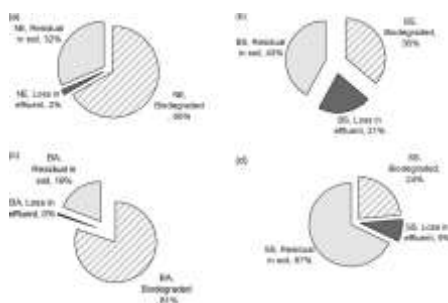
Figure 2 Biodegradation of petroleum hydrocarbons in a soil polluted with 10300 \text{ mg kg}^{-1} THP in for different treatments: bioaugmentation (BA), biostimulation with biosurfactants (BS), nutrients addition (NE) and a control (SS) (Liu et al., 2008)
