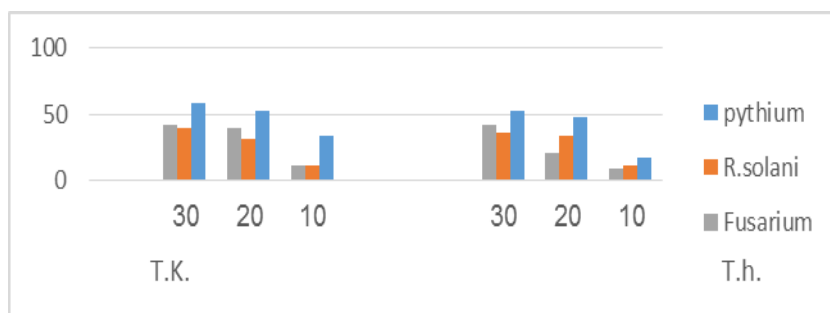
Fig. 4 The inhibition of the pathogenic fungi in a different concentrations of filtrates types of fungus T.harzianum and T.Koningii
