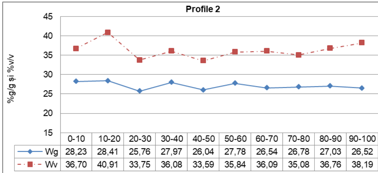
Figure 4 The gravimetric and volumetric values of field capacity on cambic colluvic Chernozems
