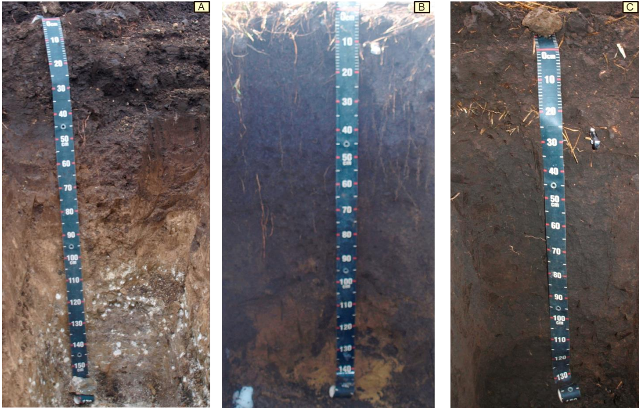
Figure 2. Soil profiles in the eastern slope of the Ursului Valley (A: profile 1 - Cambic Chernozems; B: profile 2 - Colluvic cambic Chernozems; C: profile 3 - Gleyic colluvic Chernozems)
