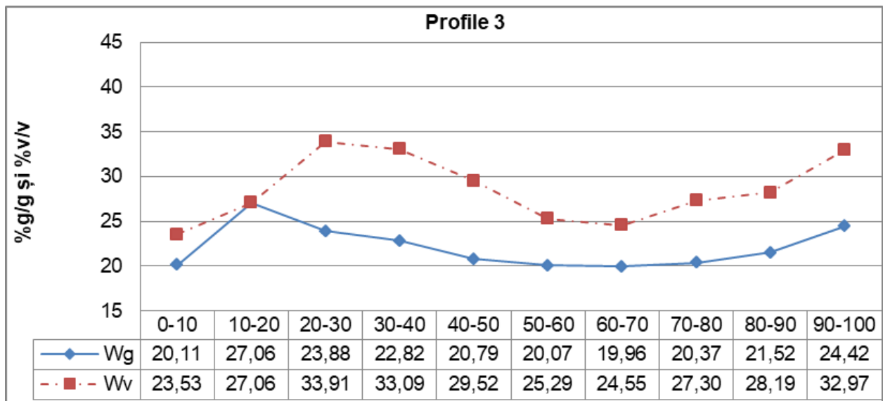
Figure 5 The gravimetric and volumetric values of field capacity on the gleyic-colluvic Chernozems
