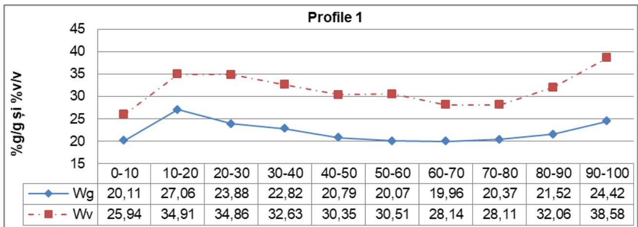
Figure 3 The gravimetric and volumetric values of filed capacity from cambic Chernozems
