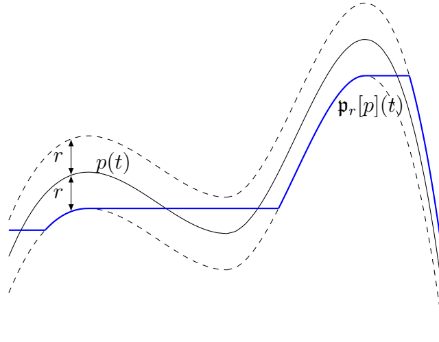
Figure 2: Application of the Play operator \mathfrak{p} on given function p .
