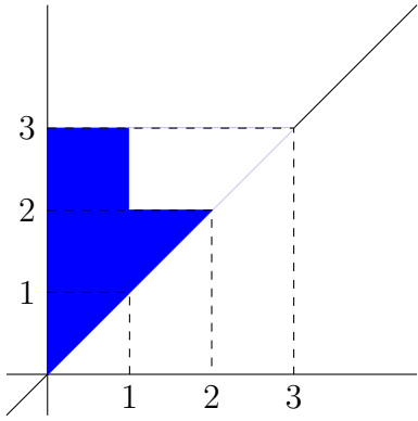
Figure 5: G_0[p](t_3) .
