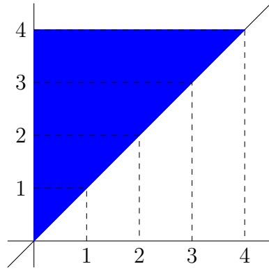
Figure 6: G_0[p](t_4) .
