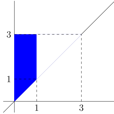
Figure 4: G_0[p](t_2) .
