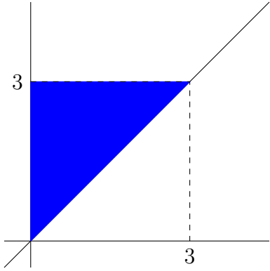
Figure 3: G_0[p](t_1) .
