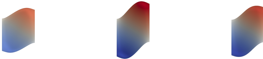
Figure 7: p(t = 0.175) .
