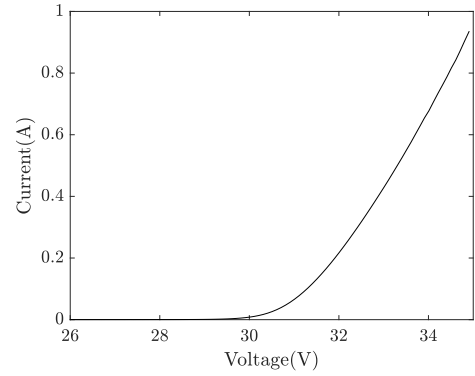
Fig. 2: Measured V-I curve of the LED panel.
