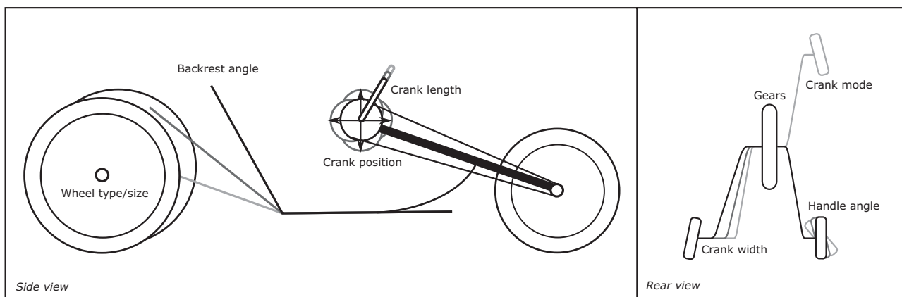
Figure 3. Overview of potential adjustments/configurations of a fixed frame handcycle.
