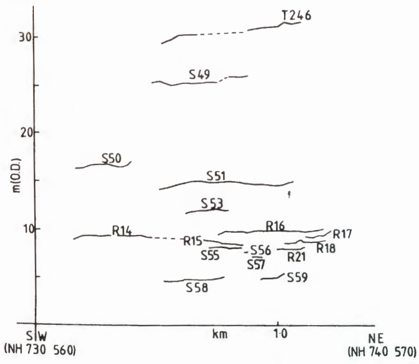
FIGURE 38 The Fortrose area.
