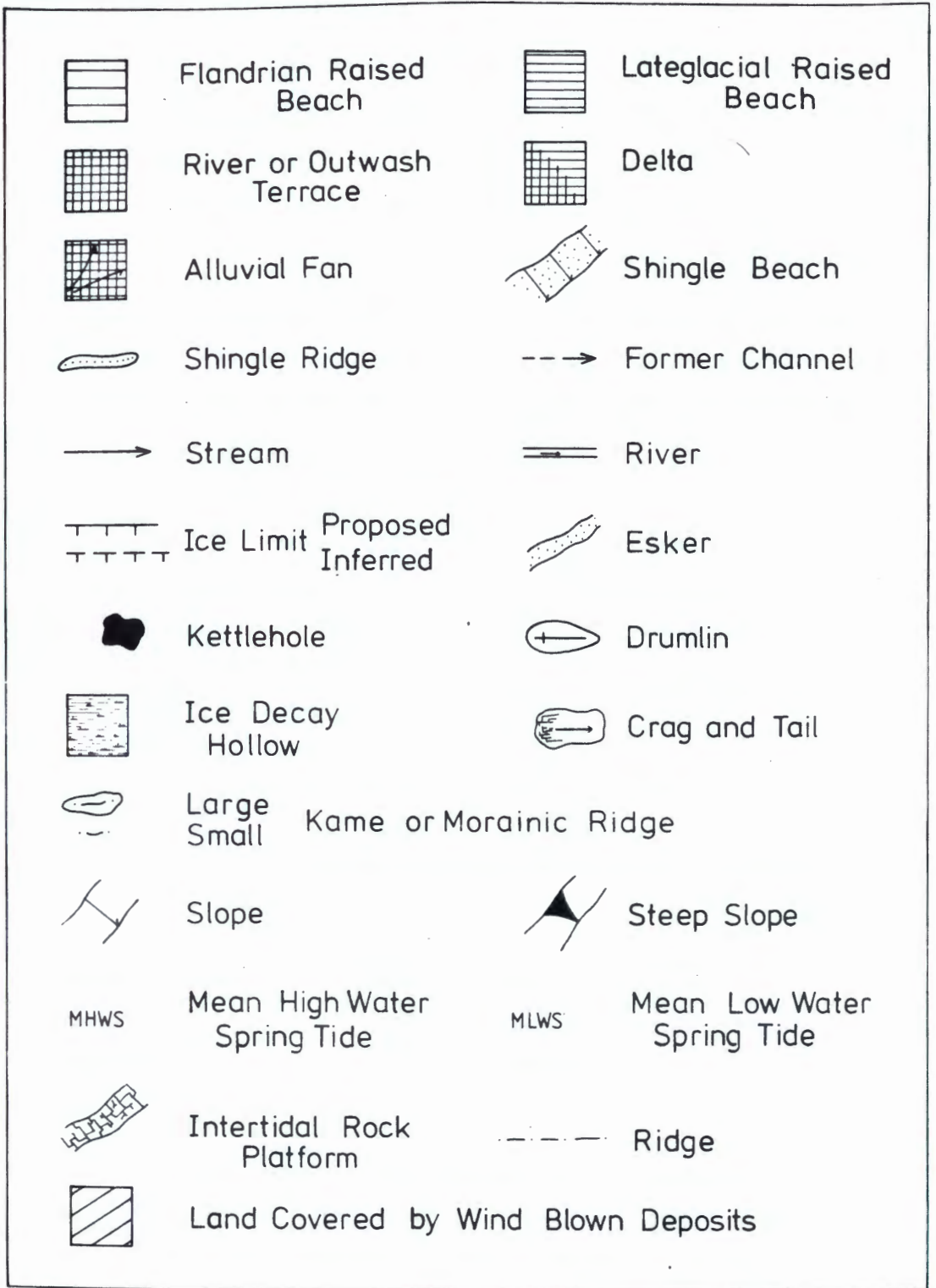
FIGURE 16 The morphological map symbols used in the thesis.
