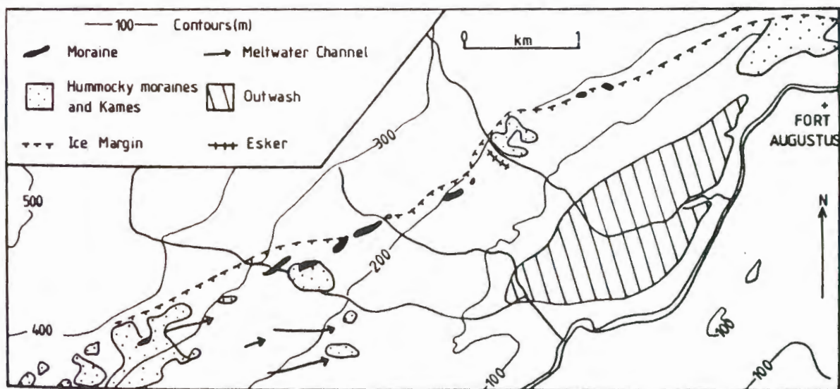
FIGURE 41 The Loch Lomond Stadal ice limit identified at Fort Augustus by Sissons (1979c).
