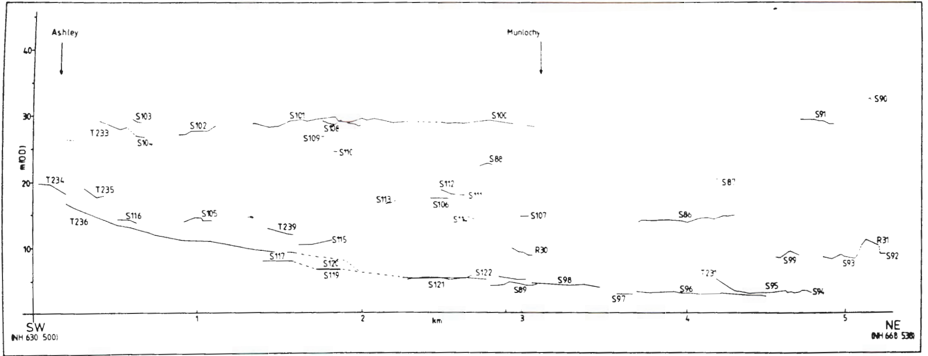
FIGURE 37 Altitude data for the Munloch Bay and Munloch Valley areas.
