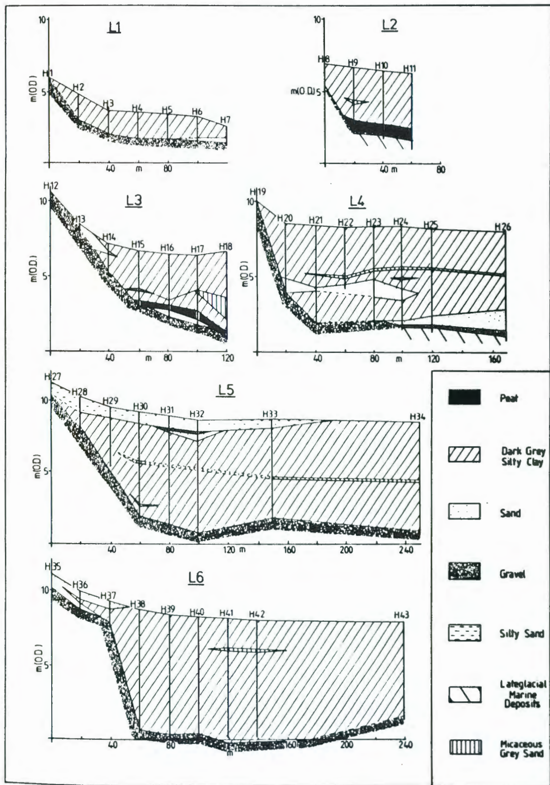
FIGURE 71 Sections drawn up along the transect lines to reveal the depth of the 'buried gravel layer'.
