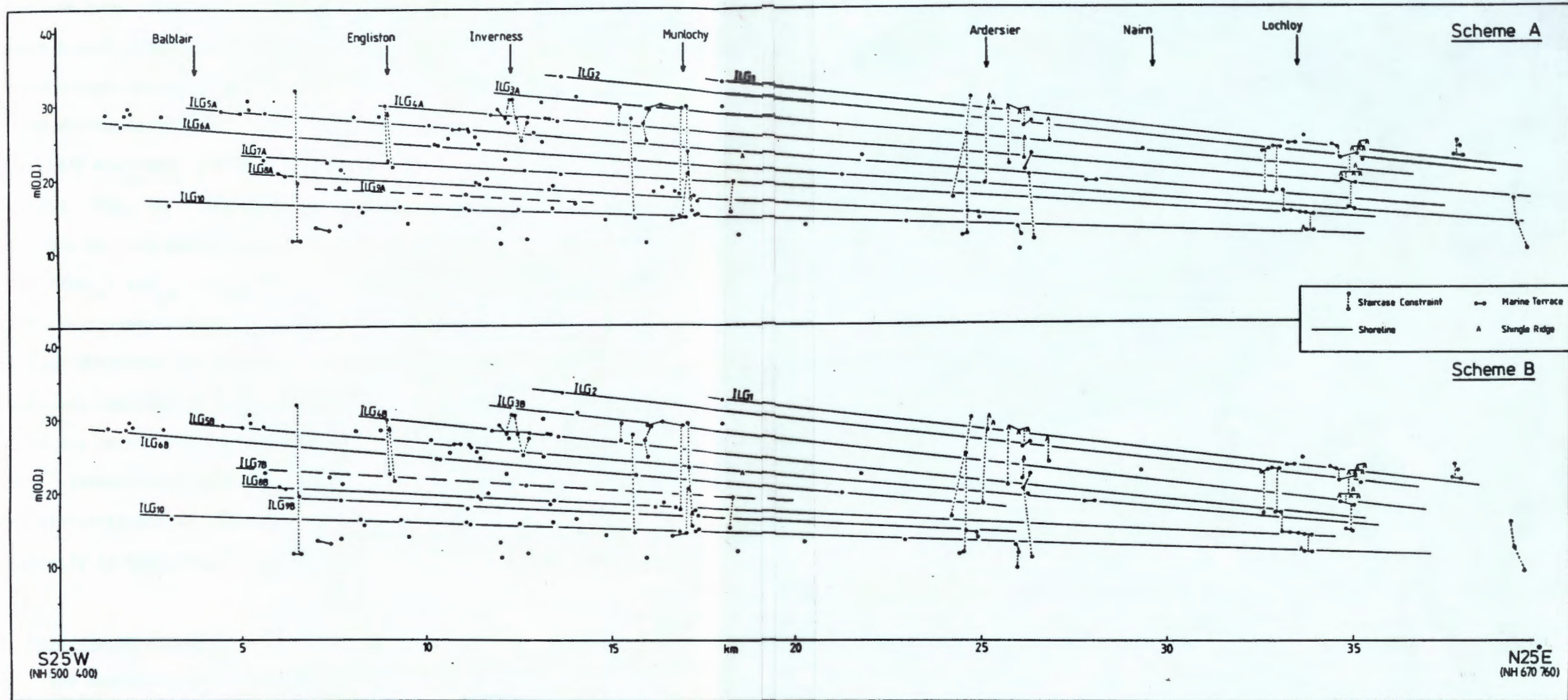
FIGURE 75 Height-distance diagram aligned along the plane of projection S25° W-N25° E to show the two possible schemes of correlation of the Lateglacial shoreline fragments in the inner Moray Firth area.
