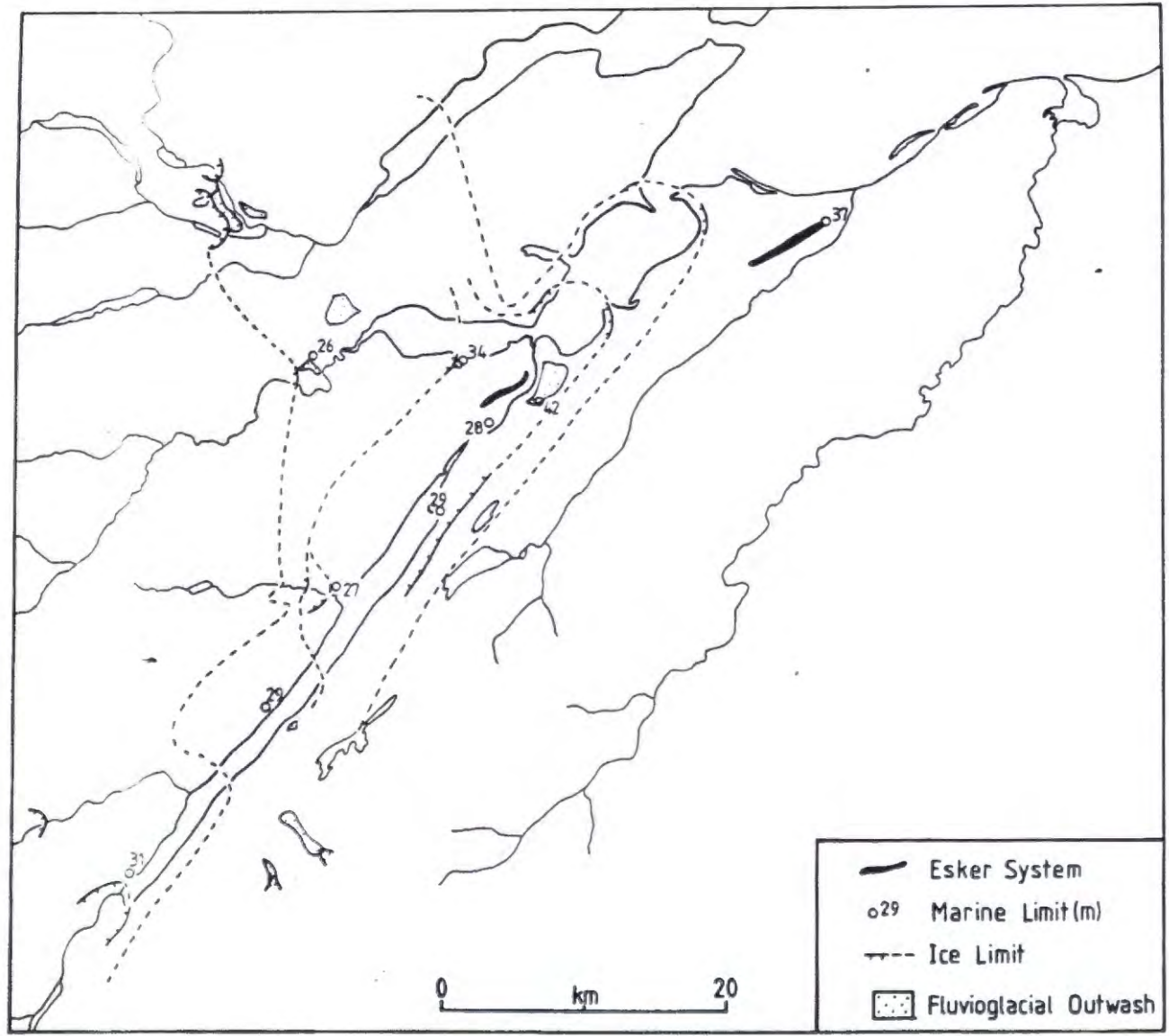
FIGURE 14 Late Devensian ice limits in the inner Moray Firth area as proposed by Syngé (1977a) and Syngé and Smith (1980).
