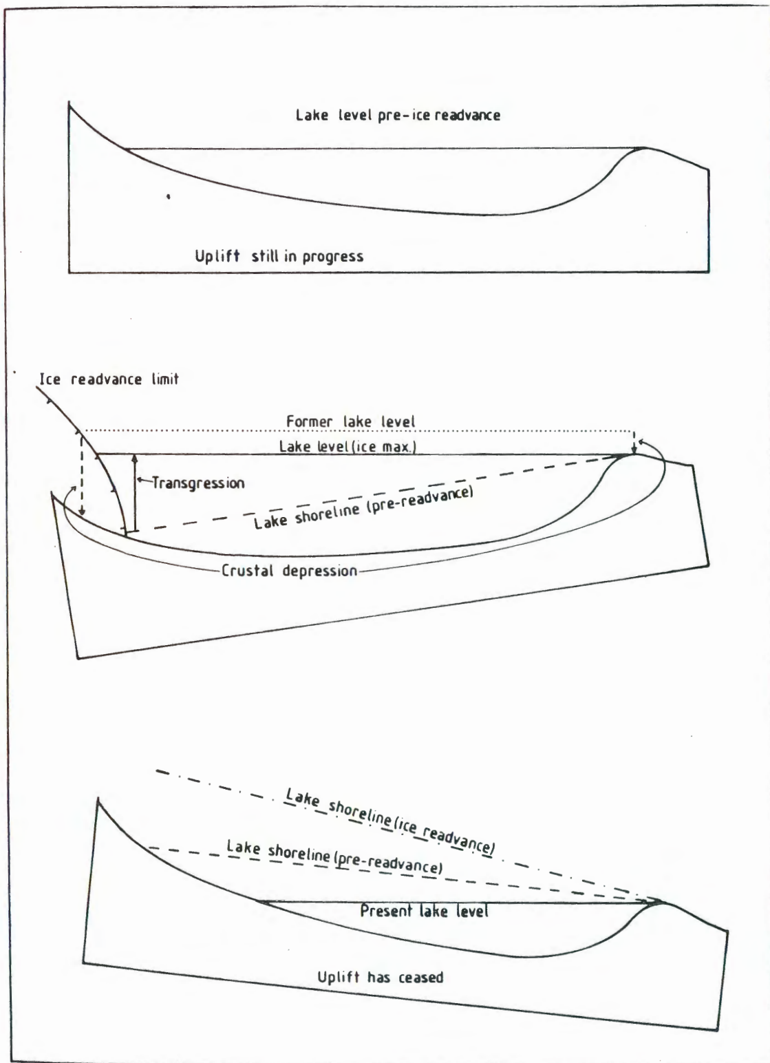
FIGURE 52 An idealised diagram to indicate the possible sequence of lacustrine shorelines which are formed during glacio-isostatic redepression of the crust and during the subsequent period of uplift.
