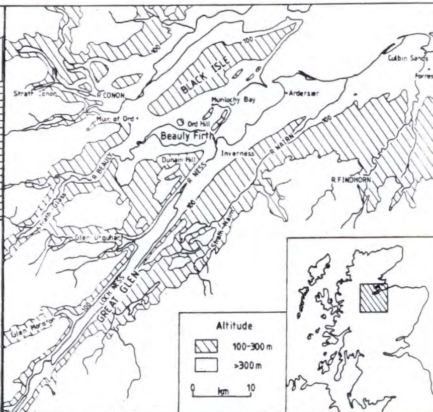
FIGURE 3 Topography of the inner Moray Firth area.
