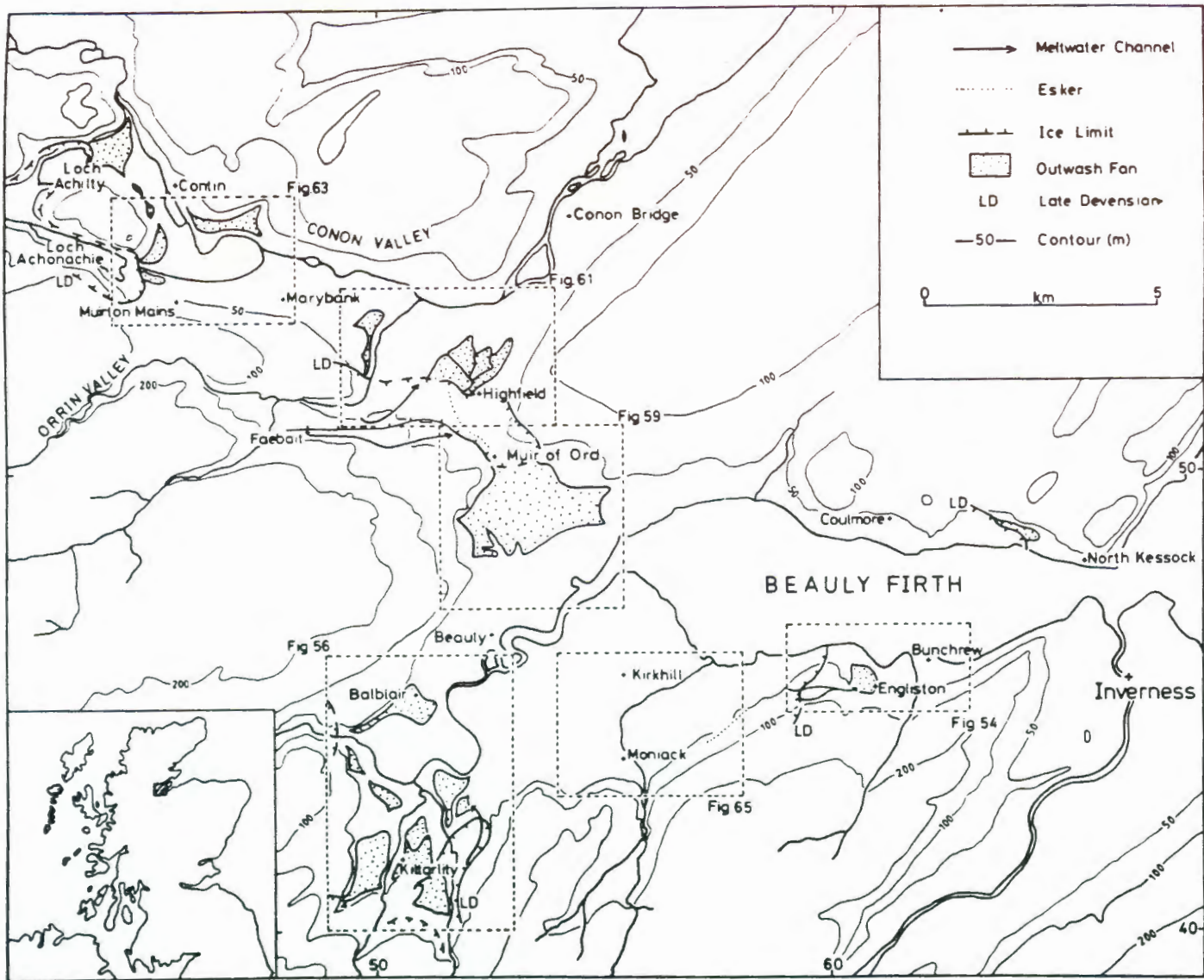
FIGURE 53 The Beaully Firth region.
