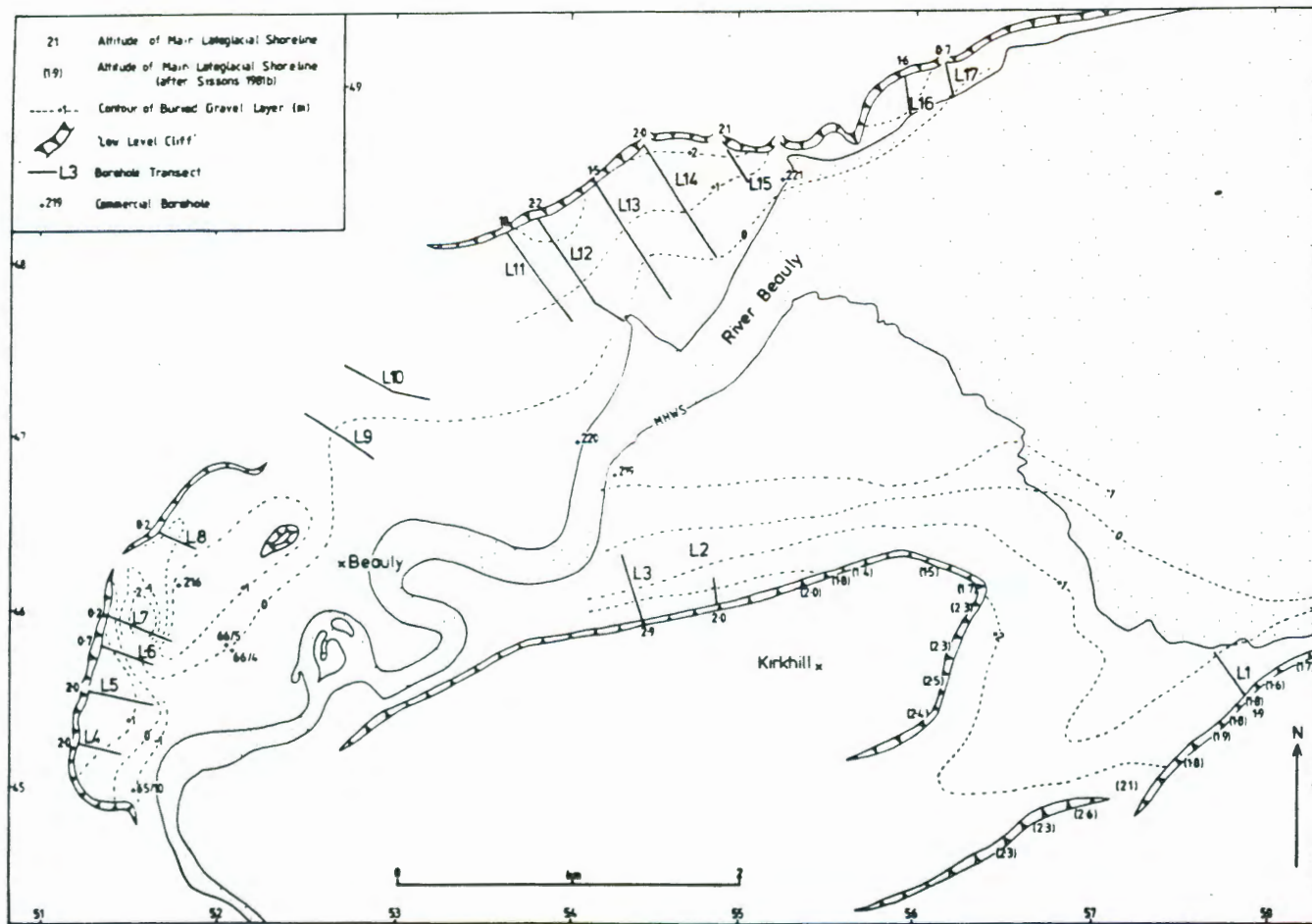
FIGURE 69 The location of the borehole transects at the head of the Beaully Firth, the altitude of the buried gravel layer and the inferred altitude of the Main Lateglacial shoreline (modified from Sissons, 1981b).
