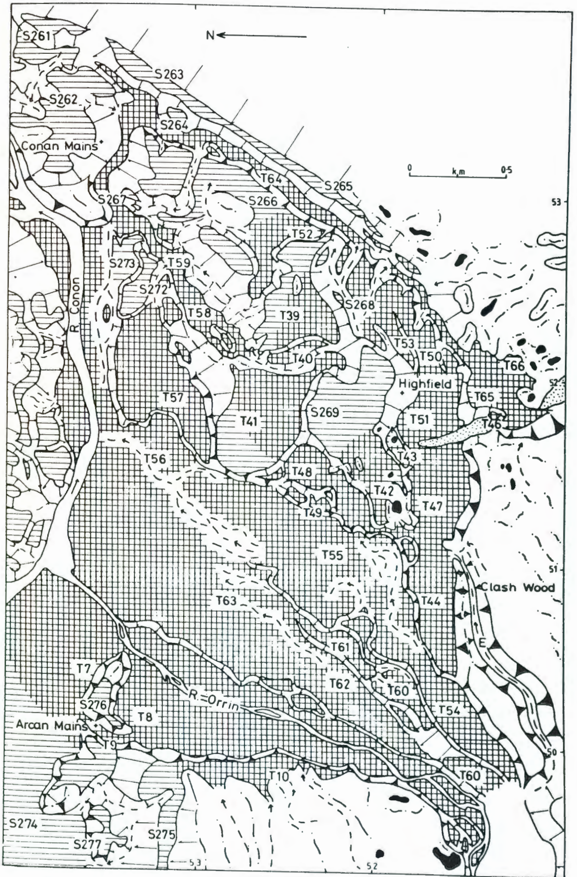
FIGURE 61 The Highfield area.
