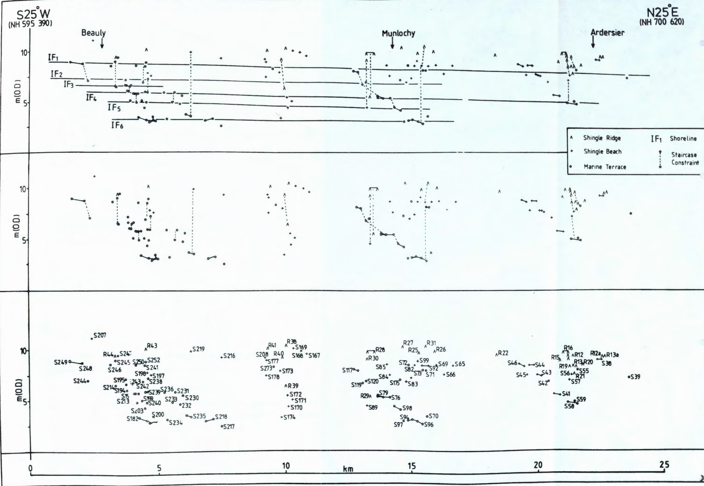
FIGURE 82a. Height-distance diagram aligned along the plane of projection S25 W-N25 E to show the location and coelevation of Flandrian marine shoreline fragments in the inner Moray Firth area.
