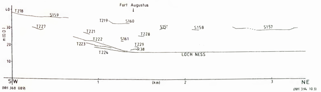
FIGURE 42 The Fort Augustus area.
