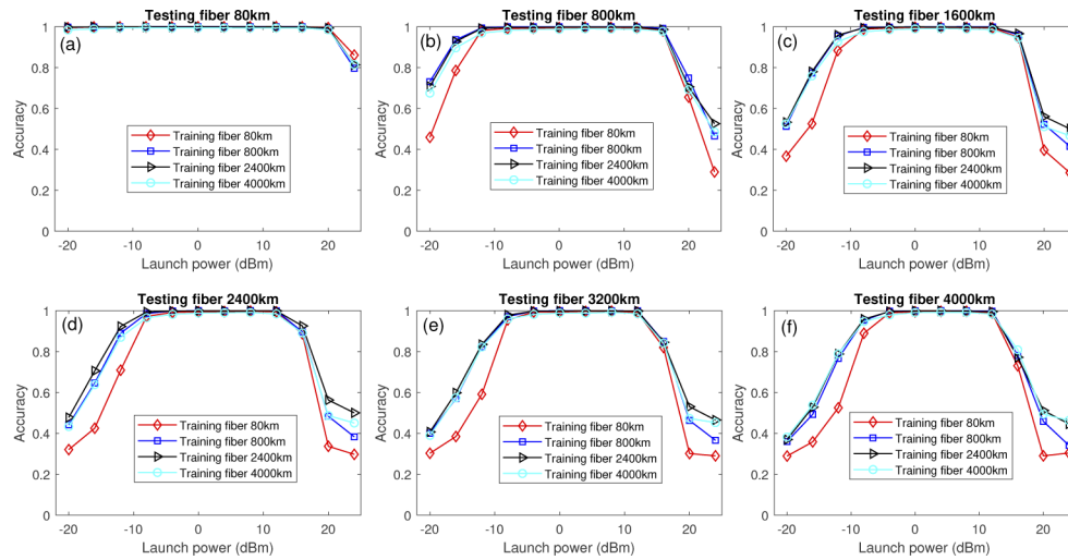
Fig. 6. Classifier accuracy under different training and testing fiber transmission distances. Classifiers are trained with fiber distances at 80 km, 800 km, 2400km and 4000 km. TSPSC is fixed at 1000. Training data covers launch power ranging from -20 dBm to 24 dBm. (a) Testing fiber distance at 80 km. (b) Testing fiber distance at 800 km. (c) Testing fiber distance at 1600 km. (d) Testing fiber distance at 2400 km. (e) Testing fiber distance at 3200 km. (f) Testing fiber distance at 4000 km.
