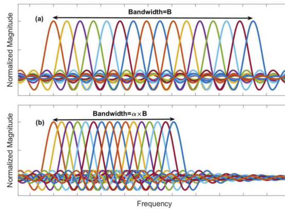
Fig. 2. Sub-carrier packing illustration. (a) OFDM. (b) SEFDM. The parameter \alpha indicates bandwidth compression factor.
