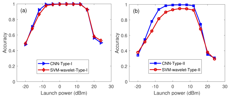
Fig. 16. Comparisons between deep learning CNN classification and machine learning SVM-wavelet classification. Type-I signal patterns: OFDM, SEFDM ( \alpha=0.9, 0.8, 0.7 ). Type-II signal patterns: OFDM, SEFDM ( \alpha=0.95, 0.9, 0.85, 0.8, 0.75, 0.7 ).
