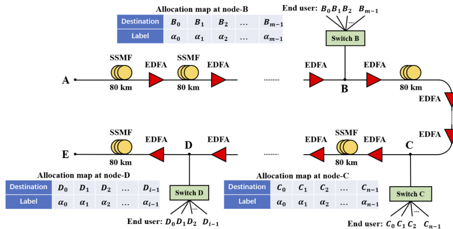
Fig. 1. Application scenario for the spectral compression labelling signal distribution in private optical networks. The parameter \alpha , ranging from 0 to 1, indicates the spectral compression ratio for the multi-carrier signals.
