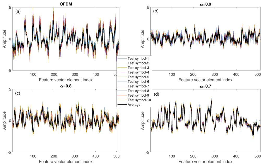
Fig. 15. Flatten feature vectors illustration after the convolutional layer in NN7.
