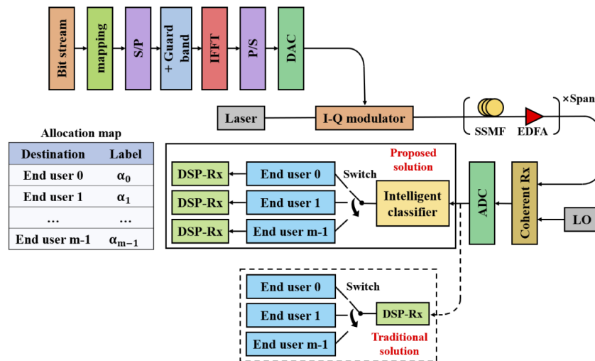
Fig. 4. Simulation model of a long-haul optical fiber transmission system. Proposed edge node intelligent receiver architecture and traditional edge node receiver architecture. The intelligent classifier will be explained in detail in the following sections.
