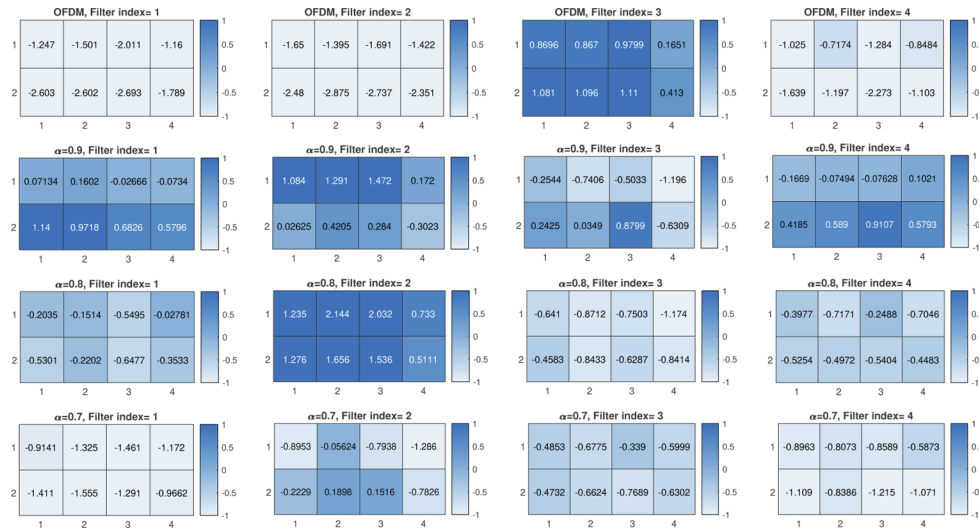
Fig. 14. Feature maps illustration after the convolutional layer in NN7.
