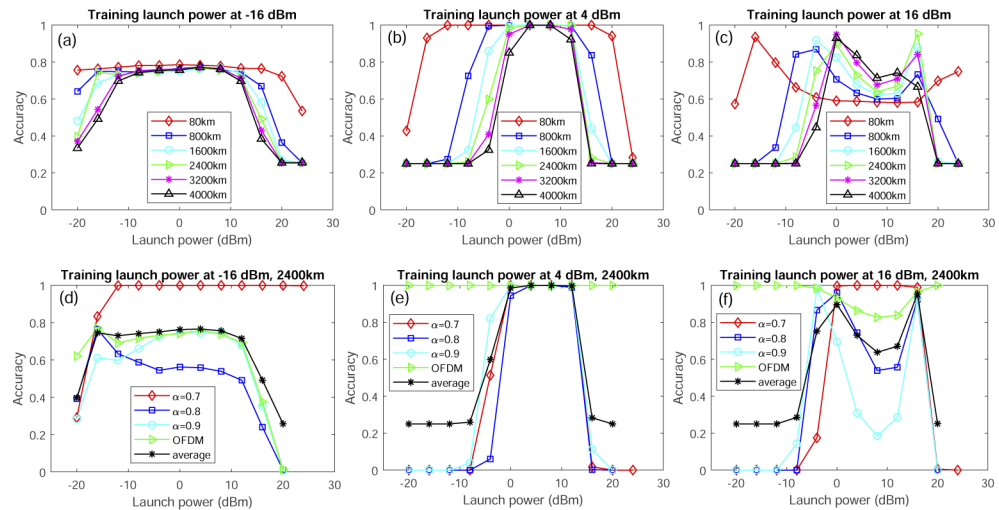
Fig. 8. Classifier accuracy under different training launch power effects. Three launch power candidates are -16 dBm, 4 dBm and 16 dBm. Training fiber distance is fixed to 2400 km. TSPSC is fixed at 1000. (a) Training launch power at -16 dBm for different testing fiber lengths. (b) Training launch power at 4 dBm for different testing fiber lengths. (c) Training launch power at 16 dBm for different testing fiber lengths. (d) Training launch power at -16 dBm for specific signals. (e) Training launch power at 4 dBm for specific signals. (f) Training launch power at 16 dBm for specific signals.
