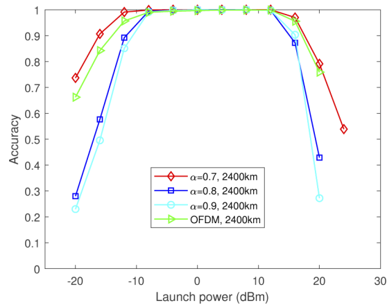
Fig. 10. Classification accuracy for each signal class ( \alpha ) testing at 2400 km fiber transmission distance.
