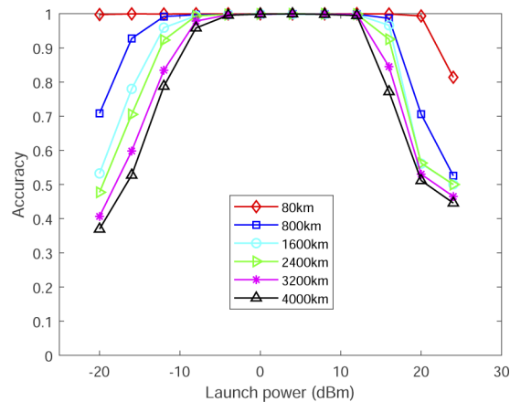
Fig. 9. Classification accuracy under different fiber transmission distances using the optimally and universally trained signal classifier.
