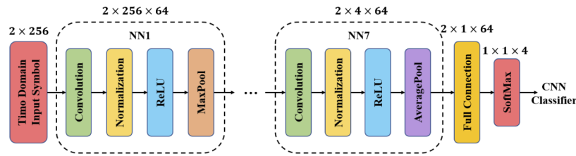
Fig. 5. CNN signal classifier architecture.
