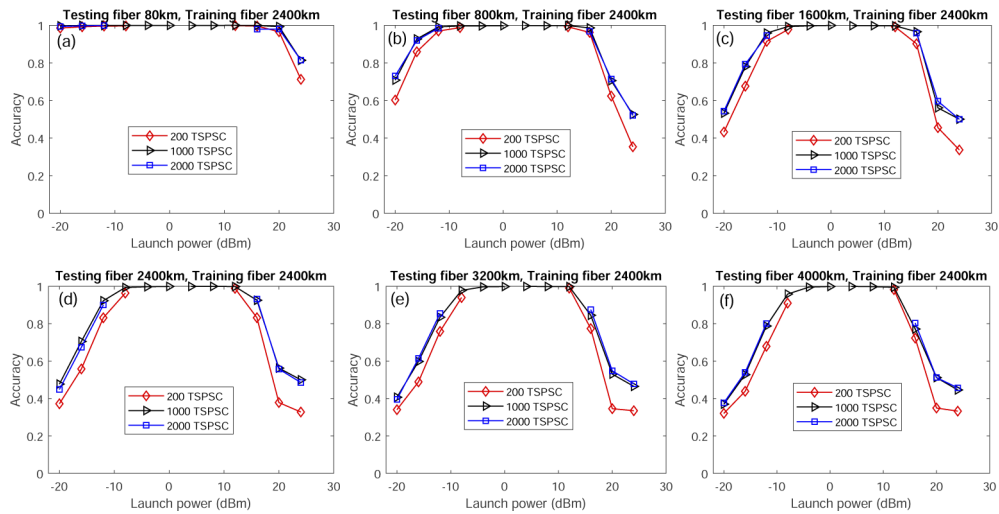
Fig. 7. Classifier accuracy under different training dataset sizes. TSPSC=200, 1000, 2000 are tested. Training fiber distance is fixed to 2400 km. Training data covers launch power ranging from -20 dBm to 24 dBm. (a) Testing fiber distance at 80 km. (b) Testing fiber distance at 800 km. (c) Testing fiber distance at 1600 km. (d) Testing fiber distance at 2400 km. (e) Testing fiber distance at 3200 km. (f) Testing fiber distance at 4000 km.
