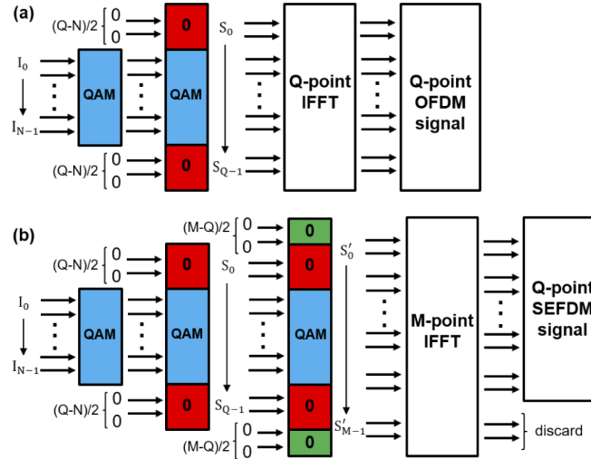
Fig. 3. Signal generation block diagram. (a) OFDM. (b) SEFDM.
