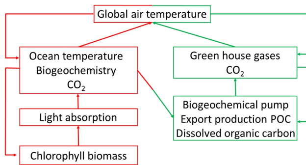
Figure 3. Schematic representation of the different links between the climate variables we analyze. The global atmospheric temperature is impacted by a biogeophysical mechanism (left, red color) and a biogeochemical mechanism (right, green color). Phytoplankton light absorption impacts directly sea surface temperature, biogeochemical properties and atmospheric \text{CO}_2 concentration, leading indirectly to changes in chlorophyll biomass and global atmospheric temperature. Increasing ecosystem complexity affects directly the export production of particulate organic carbon and thus the biogeochemical pump. As a consequence, atmospheric \text{CO}_2 concentrations and therefore global atmospheric temperature can be altered.
