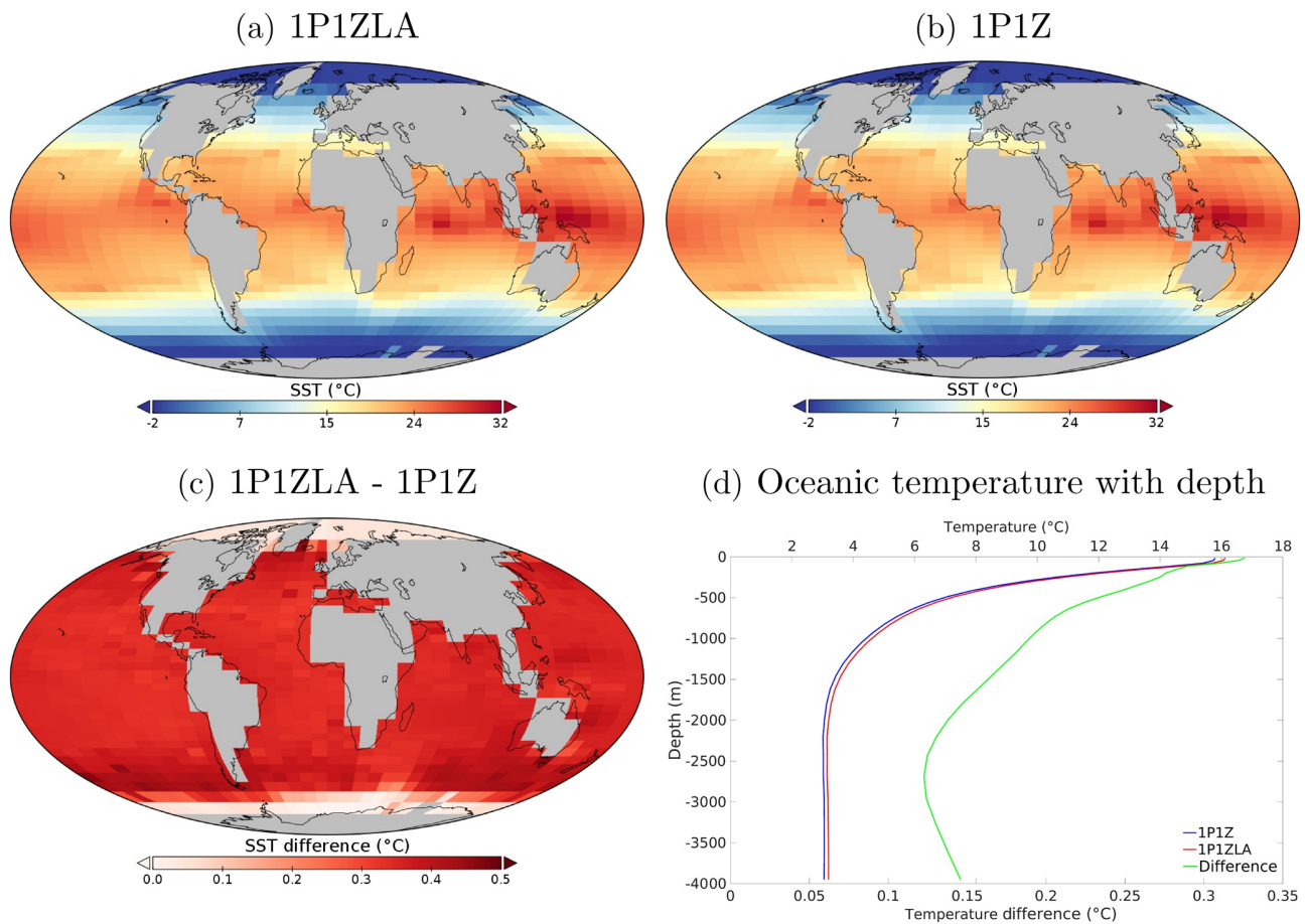
Figure 8. Sea surface temperature ( ^{\circ}\text{C} ) for the simulations (a) 1P1ZLA and (b) 1P1Z. Blue colors indicate low while red colors represent high ocean temperatures. (c) Differences of sea surface temperature between the two simulations. White color indicates small and orange/brown colors represent large differences. Note that the differences between the model simulations are always positives. (d) Variation of the oceanic temperature with depth. The red line corresponds to the model run with phytoplankton light absorption. The blue line represents the model run without. The green line represents the difference between the model simulation with and without phytoplankton light absorption.
