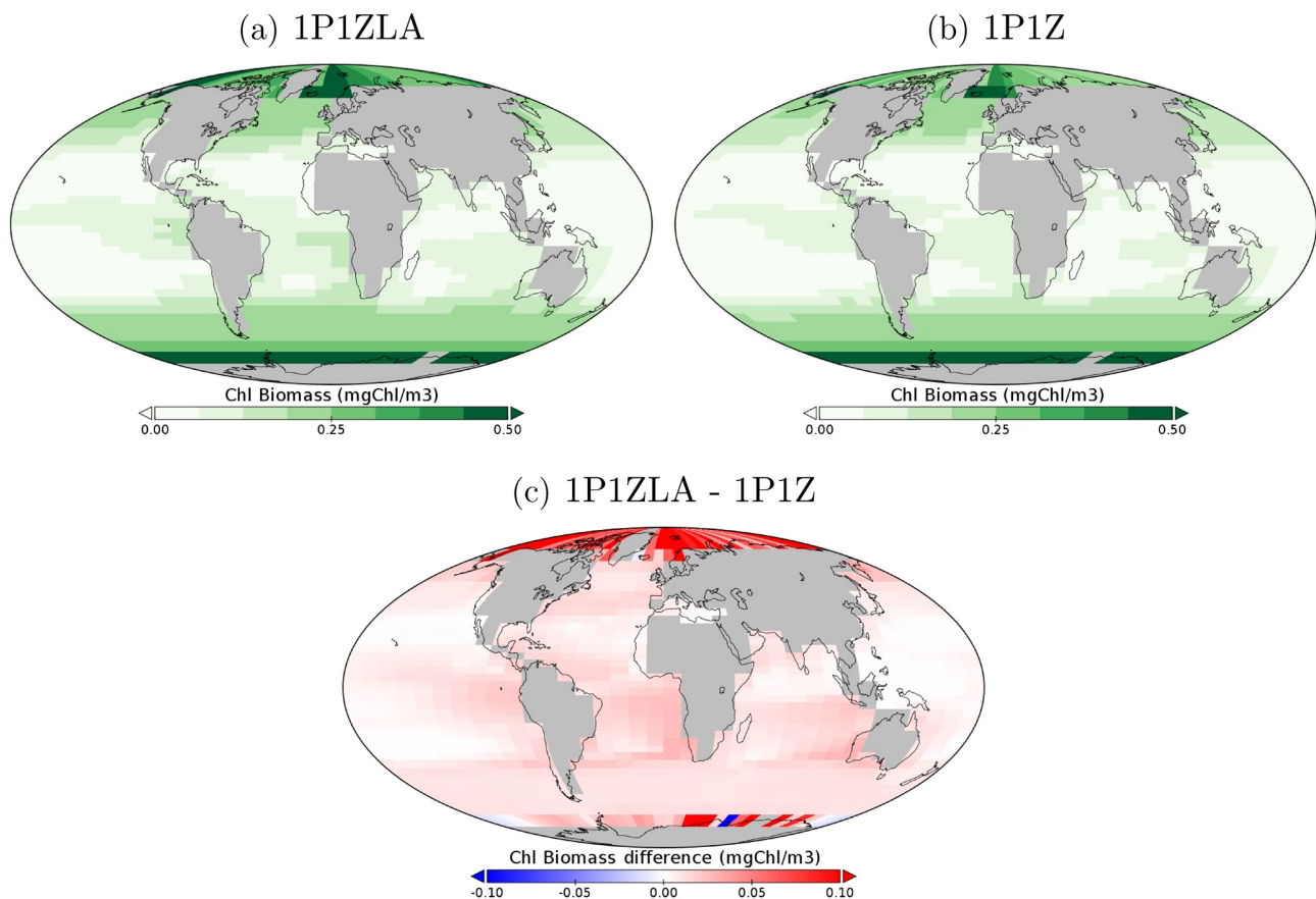
Figure 4. Chlorophyll biomass ( \text{mgChl/m}^3 ) for the model runs (a) 1P1ZLA and (b) 1P1Z. (c) Chlorophyll biomass difference between the two simulations; blue colors indicate lower while red colors indicate higher chlorophyll concentrations in the model run with light absorption.
