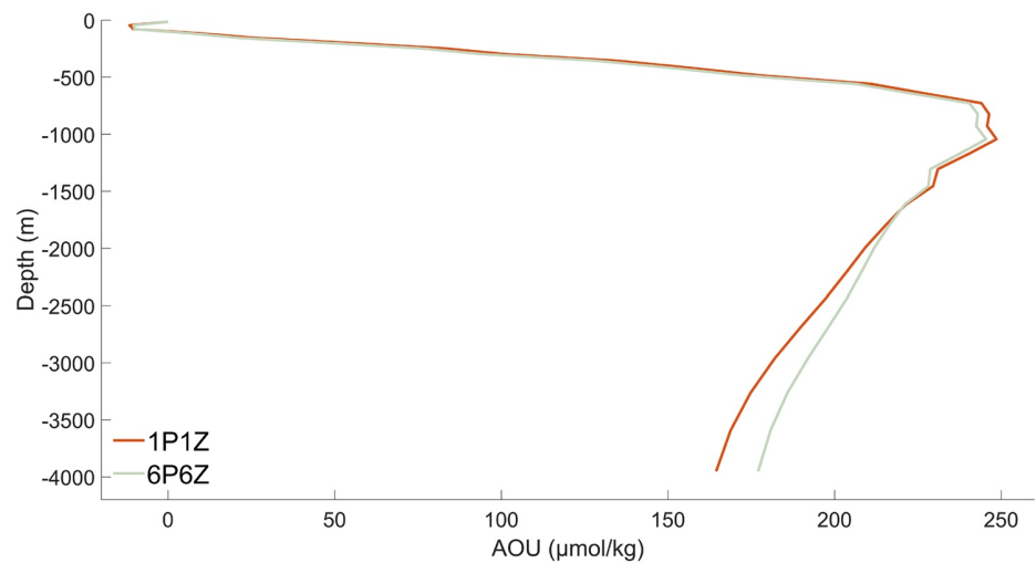
Figure 6. Vertical profile of Apparent Oxygen Utilization ( \mu\text{mol}/\text{kg} ) for the different simulations. The red curve represents the vertical profile of the simulation 1P1Z. The gray curve represents the vertical profile of the simulation 6P6Z.
