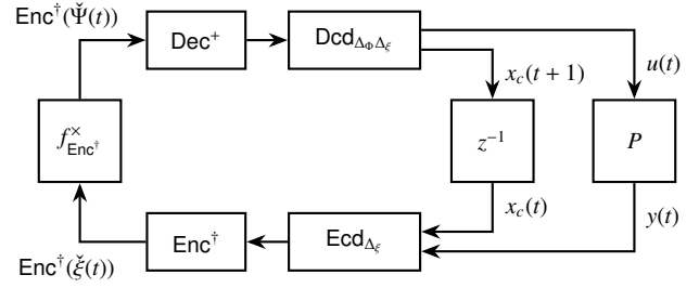
Fig. 2 Block diagram of encrypted control system.
