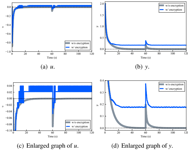
Fig. 5 Control performance of the encrypted control system using dynamic quantizer with ElGamal encryption.
