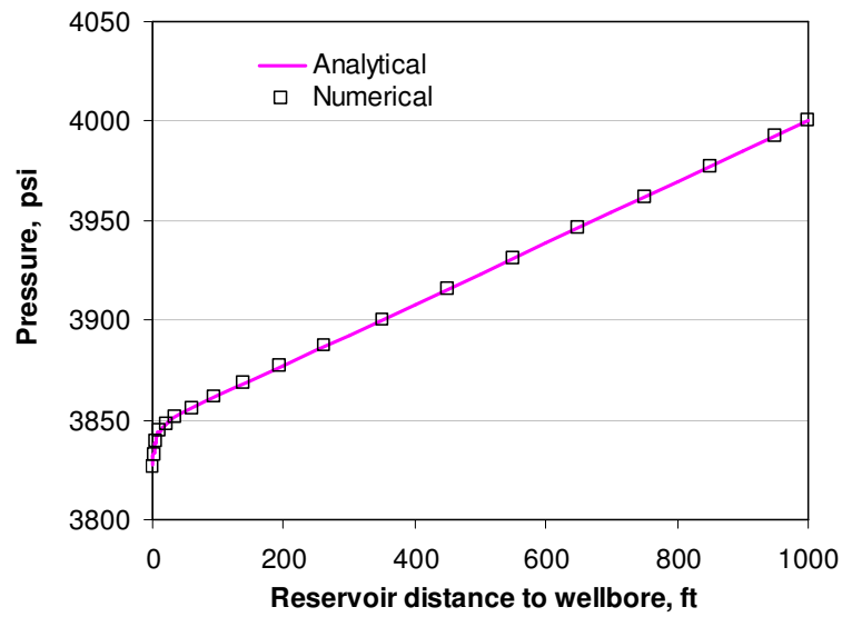
Fig. 2.6 Reservoir pressure distribution
