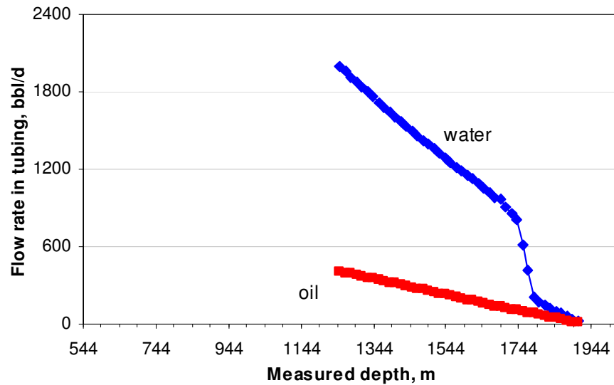
Fig. 5.15 Inverted flow rate profiles of oil and water
