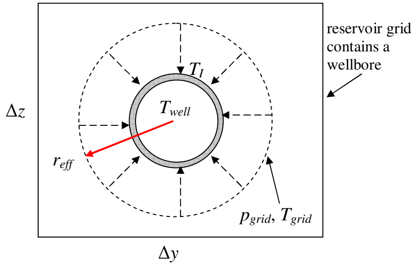
Fig. 2.2 Integrated temperature behavior between reservoir grid and wellbore
