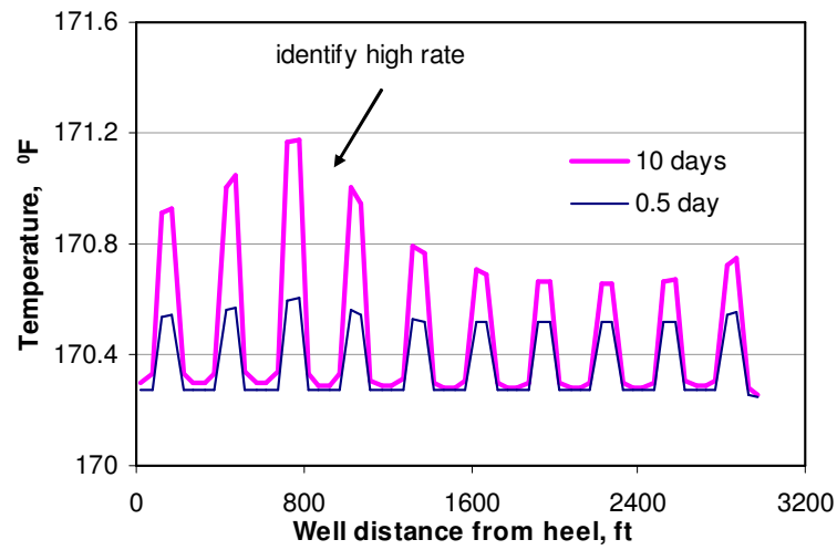
Fig. 5.45 Use temperature to identify inflow rate distribution
