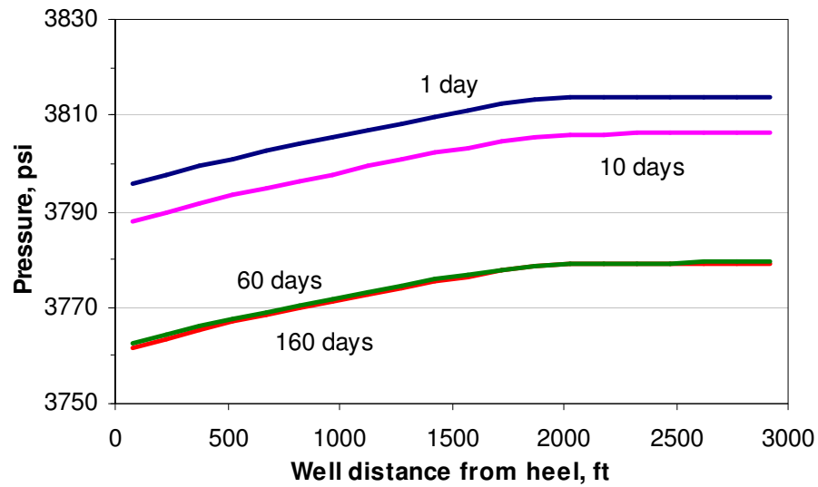
Fig. 4.6 Pressure distribution in wellbore
