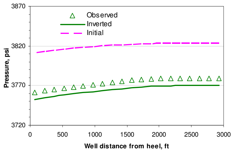
Fig. 4.19 Matched pressure data from L-M method, 2-value initial
