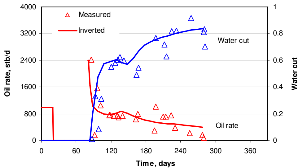
Fig. 5.14 Inverted production history follows the trend of measurement
