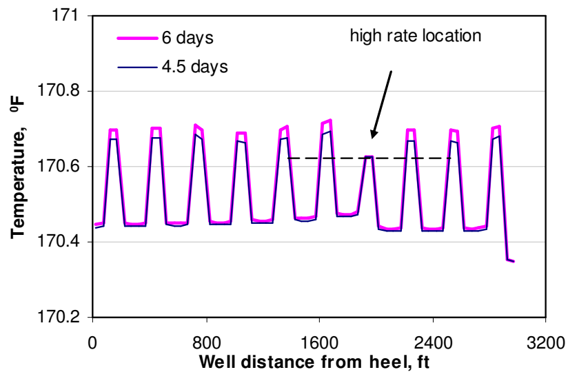
Fig. 5.29 Temperature achieves design at first adjustment
