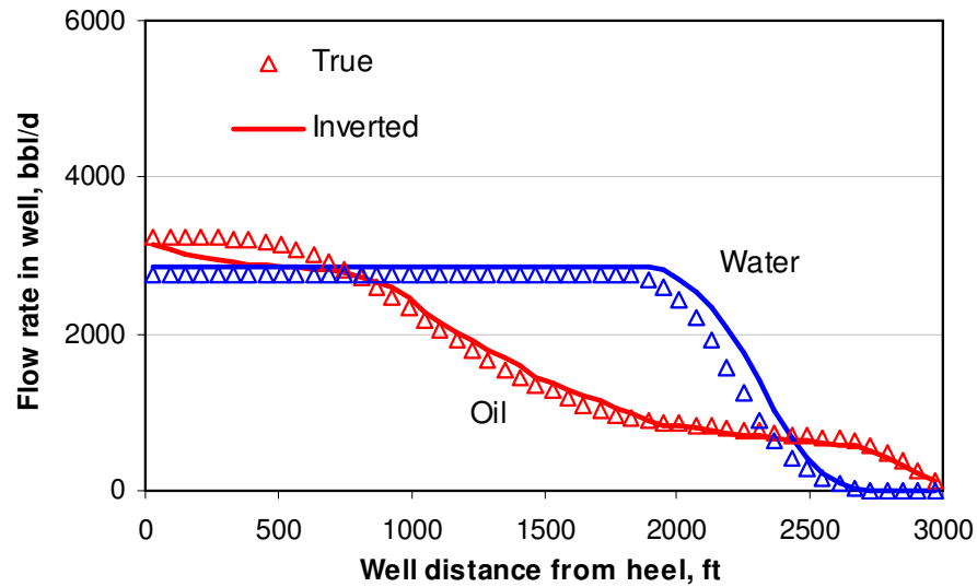
Fig. 5.58 Inverted flow rate profiles in tubing for oil and water
