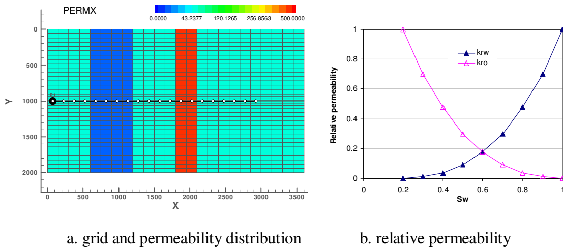
Fig. 4.2 Reservoir permeability distribution and relative permeability curve
