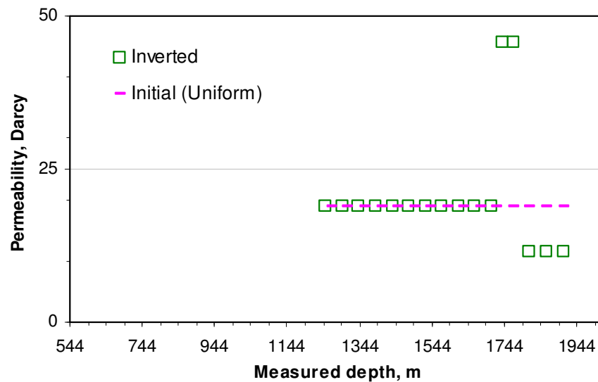
Fig. 5.13 Inverted permeability distribution of heavy oil well example
