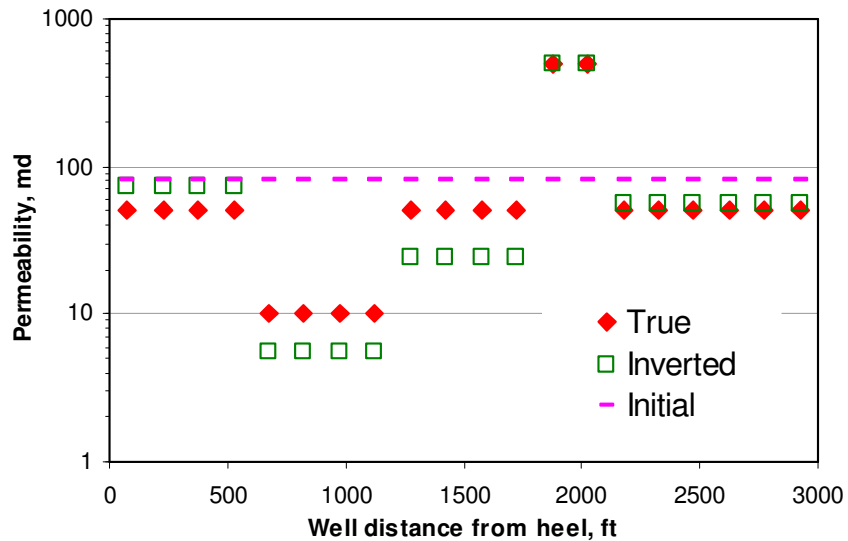
Fig. 4.26 Inverted permeability distribution from MCMC method
