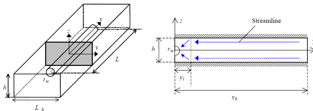
Fig. 2.5 Linear-radial flow geometry (Furui et al., 2003)
