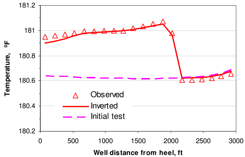
Fig. 4.23 Matched temperature data from MCMC method
