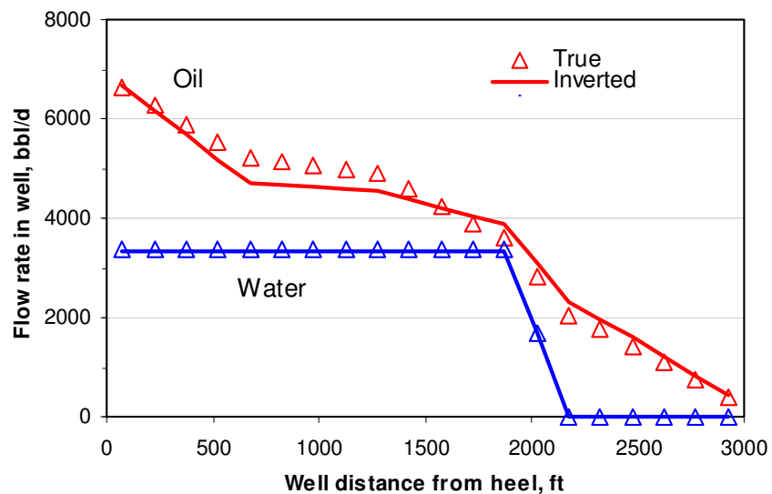
Fig. 4.25 Inverted oil and water flow rate profiles from MCMC method
