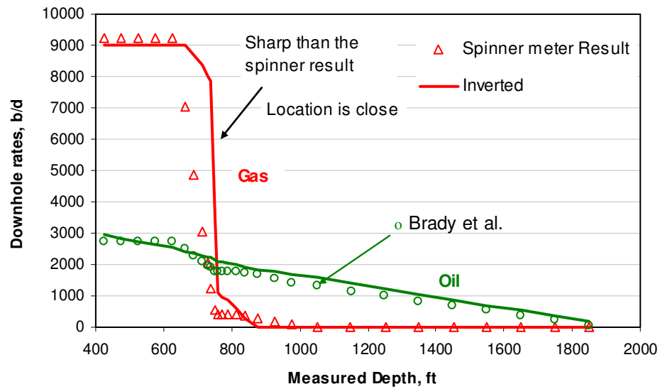
Fig. 5.3 Model interpretation result vs. spinner measurement
