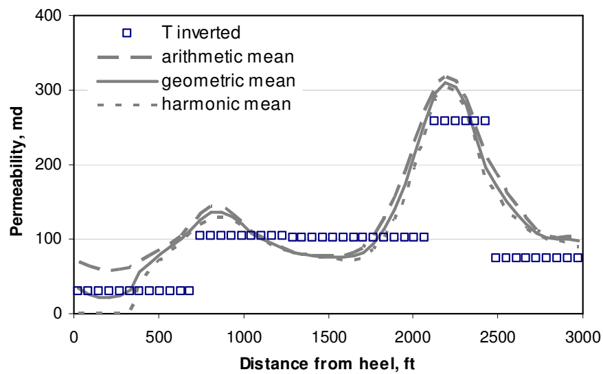
Fig. 4.37 Temperature inverted perm value vs. true perm average at y direction
