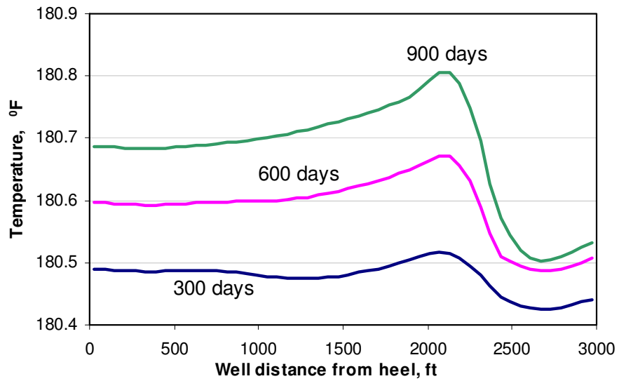
Fig. 4.31 Wellbore temperature distribution
