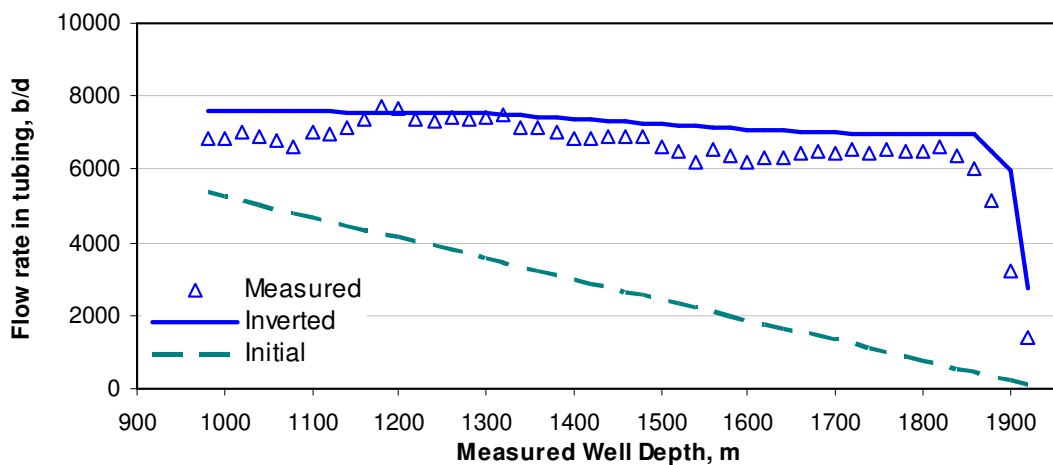
Fig. 5.11 Model interpretation compared with production logging measurement, water
