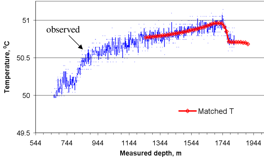
Fig. 5.12 Match measured DTS temperature data
