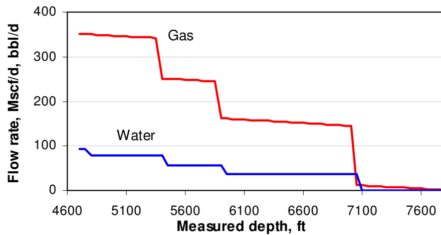
Fig. 5.19 Inverted flow rate distributions of gas and water
