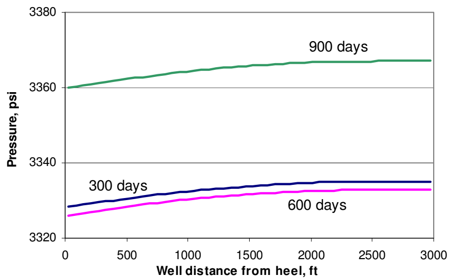
Fig. 4.32 Wellbore pressure distribution
