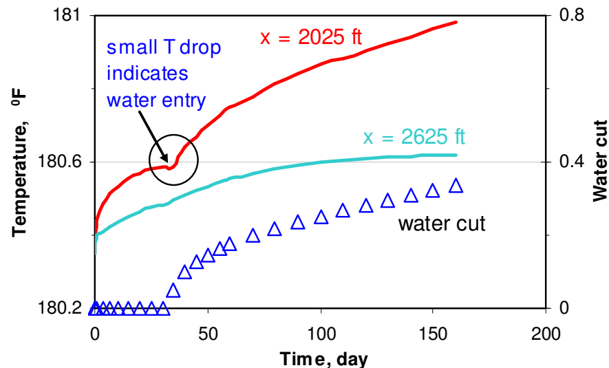
Fig. 4.8 Water cut history and transient temperature at two locations
