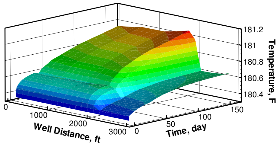
Fig. 4.9 Transient wellbore temperature distribution
