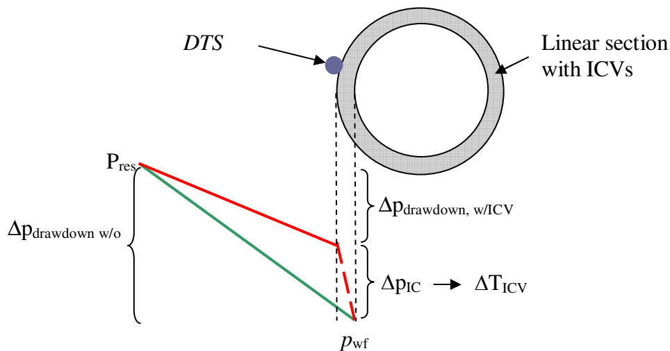
Fig. 5.22 ICV effect on pressure distribution and temperature in our model
