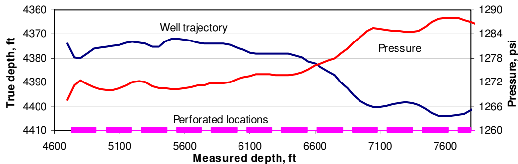
Fig. 5.17 Measured pressure, well trajectory and perforated locations
