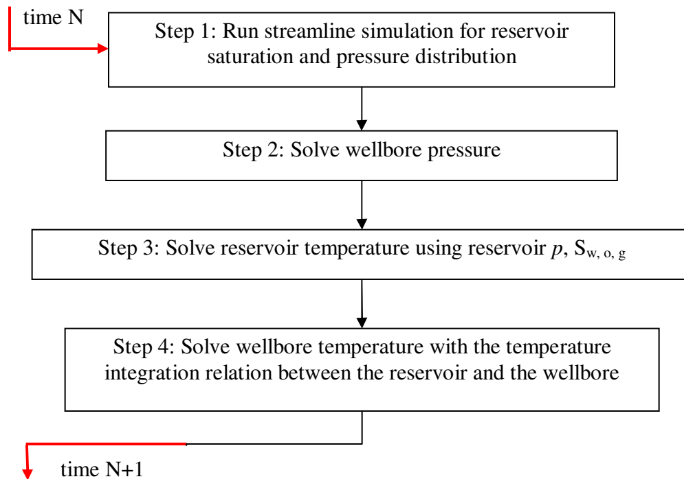
Fig. 2.4 Calculation procedure of forward model
