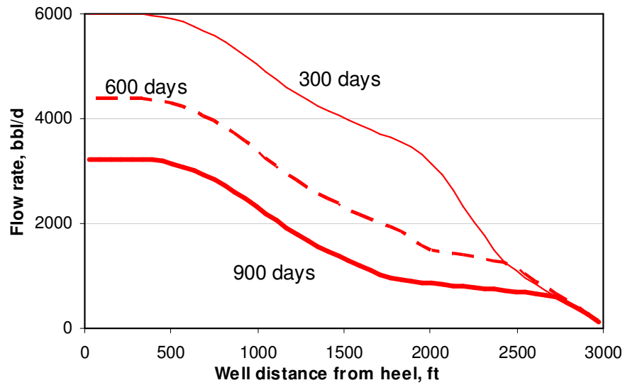
Fig. 4.29 Oil flow rate profiles in tubing
