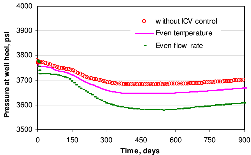
Fig. 5.34 Pressure at heel vs. time at three conditions
