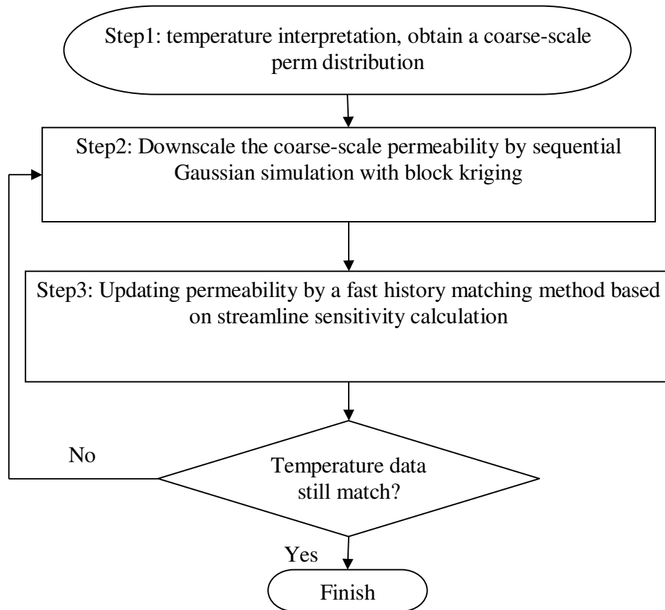
Fig. 5.51 Integrated approach for incorporating temperature data into history matching
