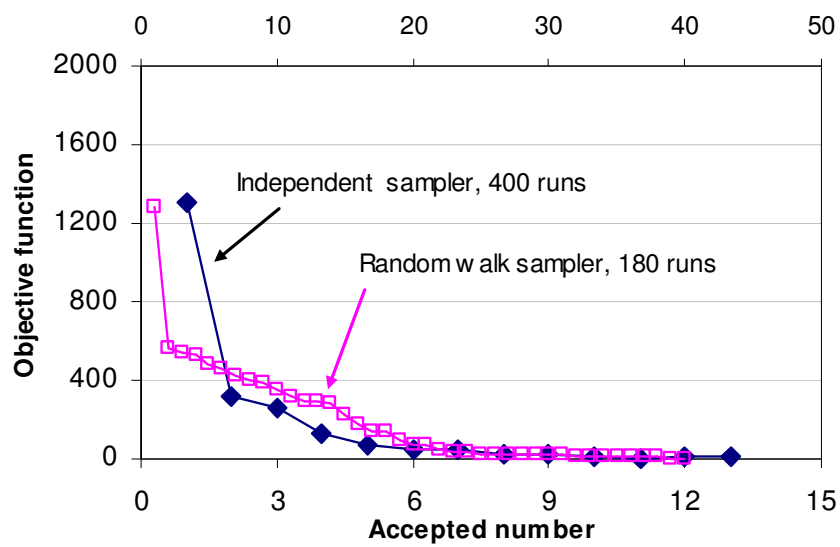
Fig. 4.22 Objective function converges
