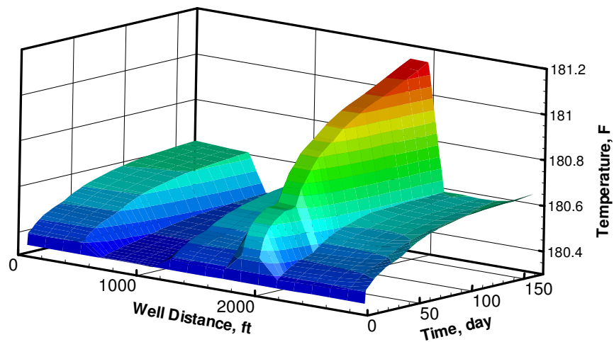
Fig. 4.10 Transient arriving temperature distribution
