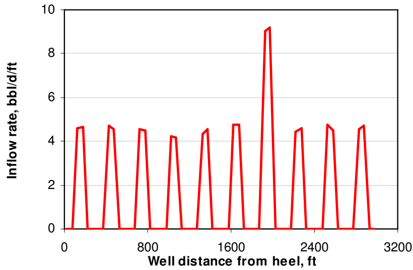
Fig. 5.30 Inflow rate distribution at first adjustment
