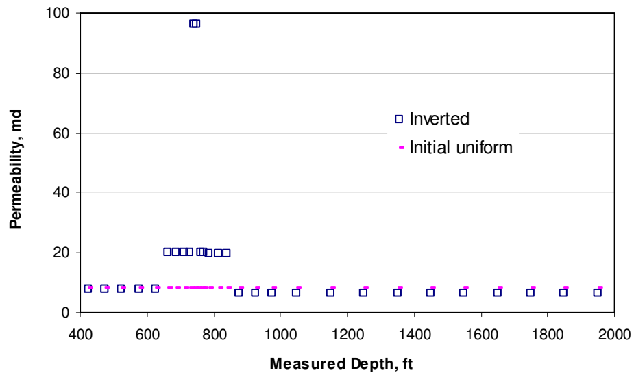
Fig. 5.4 Inverted permeability distribution of gas entry oil well example
