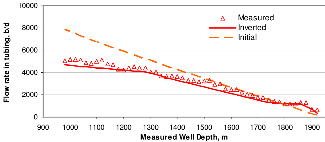
Fig. 5.10 Model interpretation compared with production logging measurement, oil
