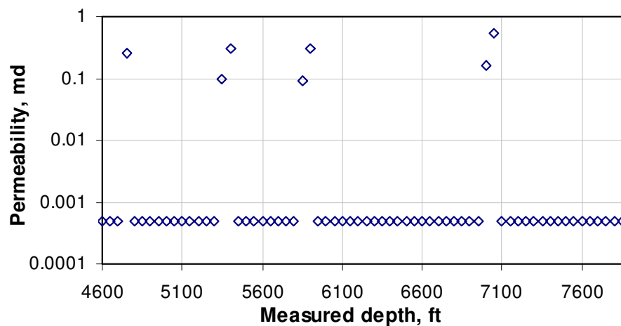
Fig. 5.20 Inverted permeability distribution of water entry gas well example
