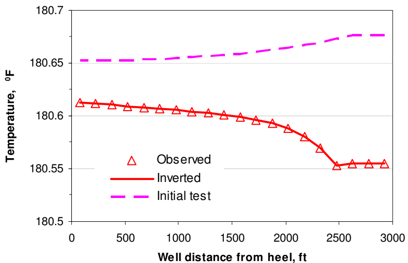
Fig. 3.3 Observed and inverted temperature data at 60 days
