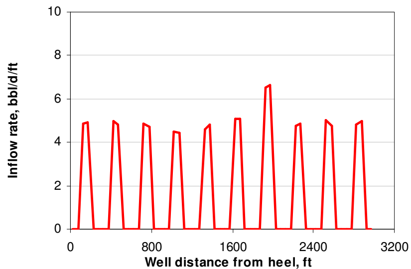
Fig. 5.32 Inflow rate is closed to evenly distribute
