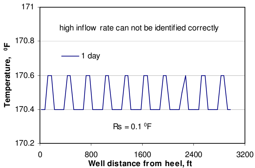
Fig. 5.38 Unable to identify high inflow sections at 1 day, R_s = 0.1 °F
