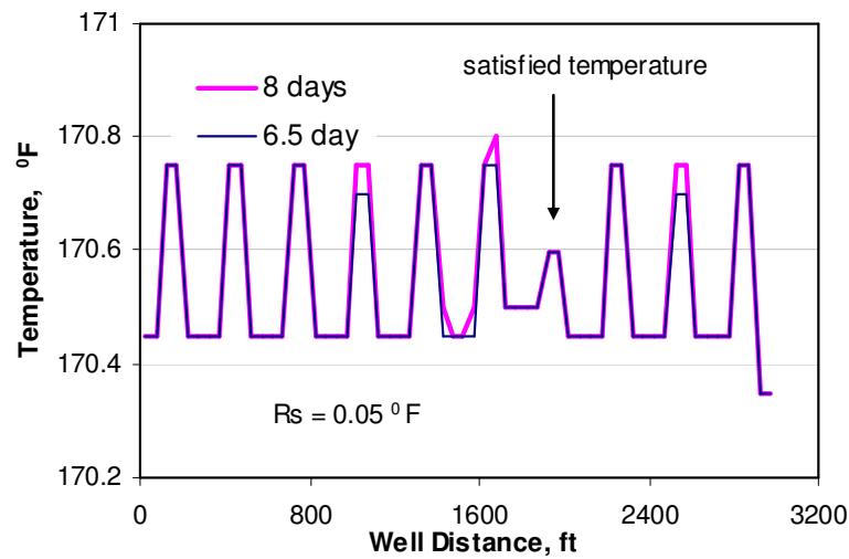
Fig. 5.36 Temperature achieves design, R_s = 0.05 °F
