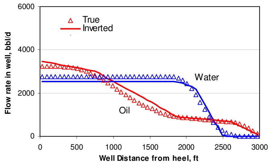
Fig. 4.36 Inverted water and oil flow rate profiles of water injection example
