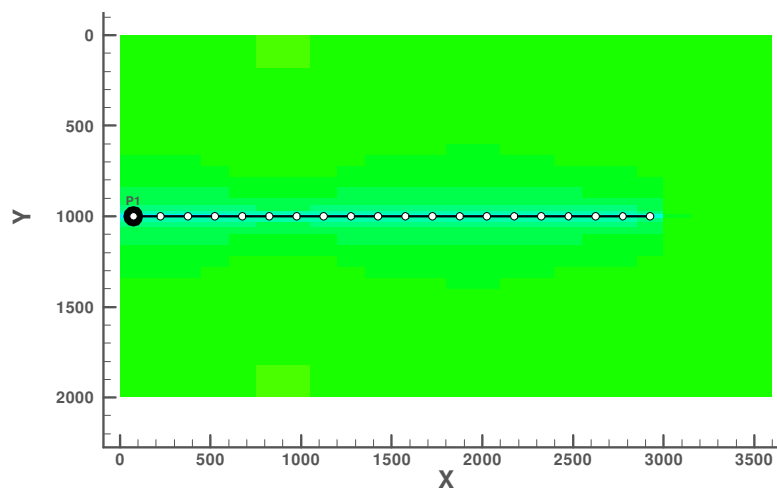
Fig. 4.11 Top view of reservoir and wellbore
