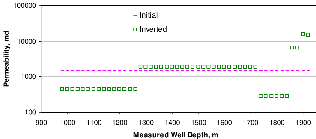
Fig. 5.9 Inverted permeability distribution of water entry oil well example
