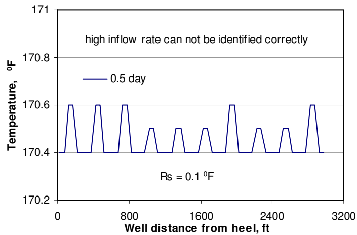
Fig. 5.37 Unable to identify high inflow sections at 0.5 day, R_s = 0.1 °F
