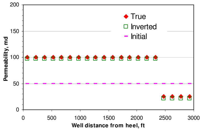
Fig. 3.5 Inverted permeability distribution of validation case
