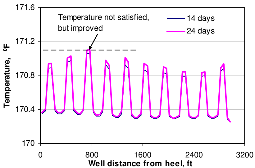
Fig. 5.48 Temperature after ICV operation
