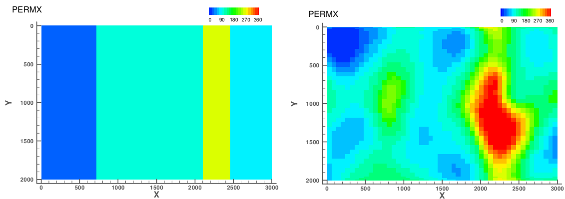
Fig. 4.35 Temperature inverted perm vs. true perm, contour
