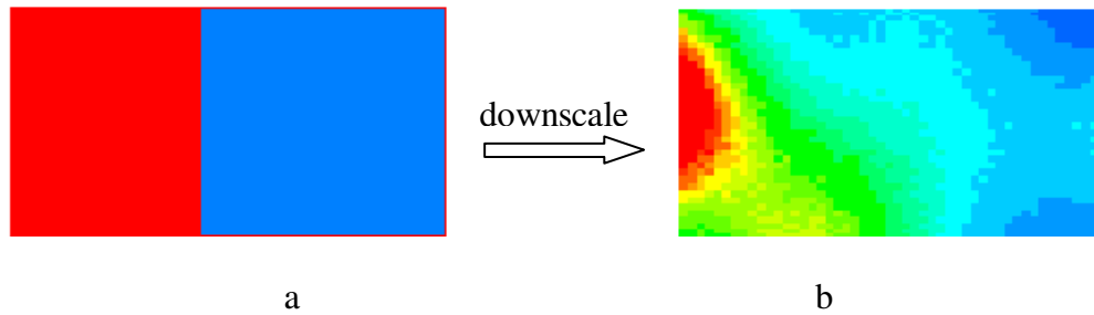
Fig. 5.52 Downscaling of the temperature inverted coarse-scale permeability
