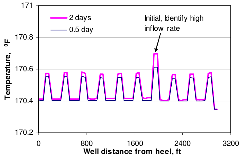
Fig. 5.25 Use temperature to identify high inflow rate before operating ICVs
