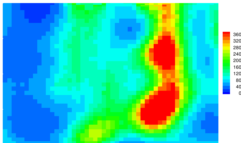
Fig. 5.55 A sample of generated permeability fields from the integrated approach
