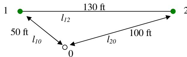
Fig. 5.53 Simple example for kriging estimation
