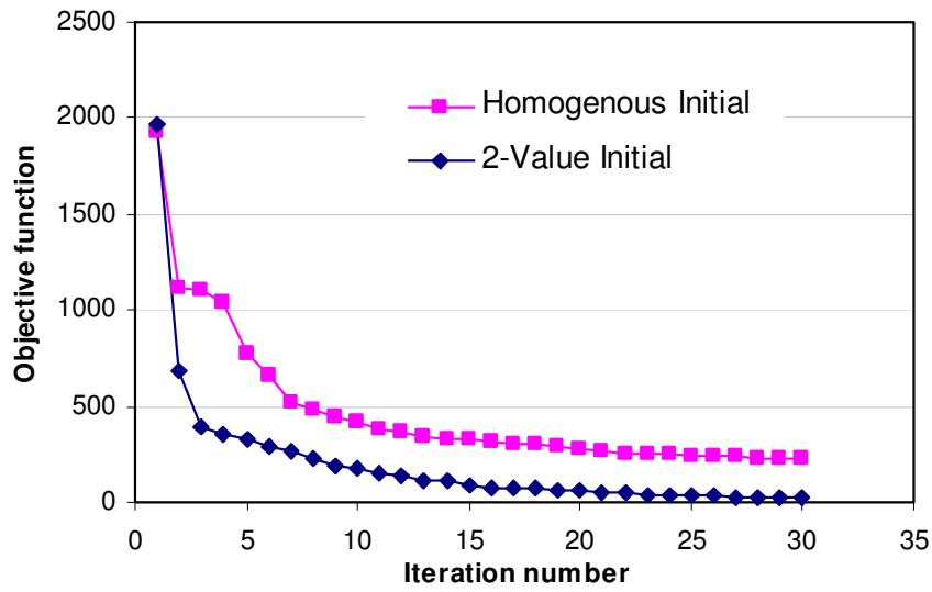
Fig. 4.13 Objective function vs. iteration number at two initial conditions
