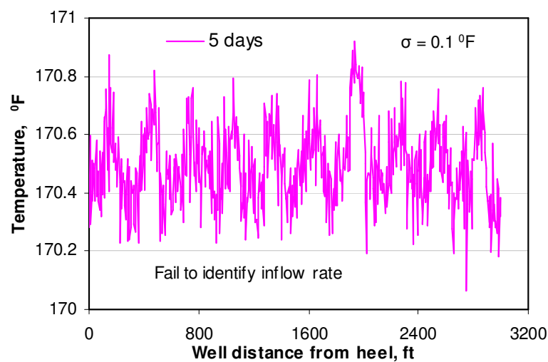
Fig. 5.43 Failure to identify high inflow sections at 5 day, \sigma = 0.1 °F
