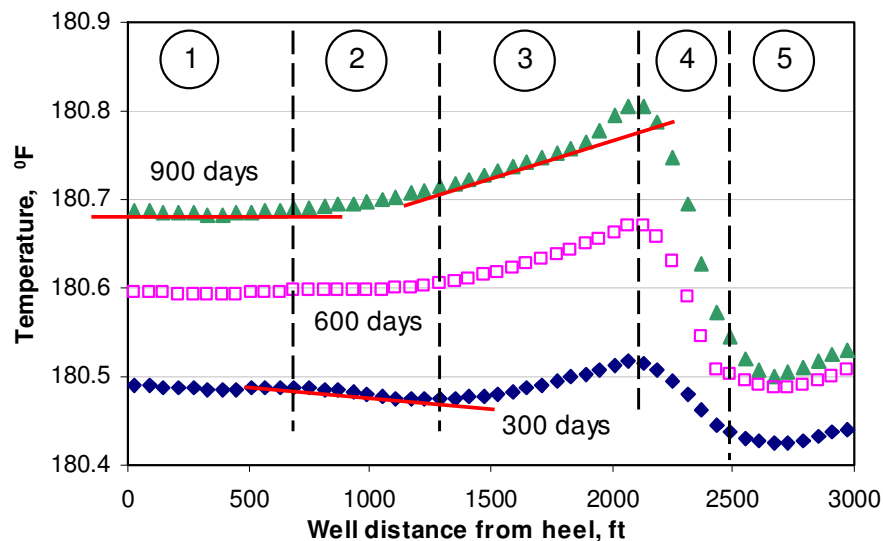
Fig. 4.33 Separate reservoir to sections by temperature data
