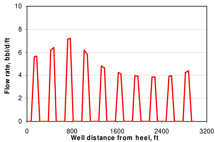
Fig. 5.46 Inflow rate distribution before operating ICV
