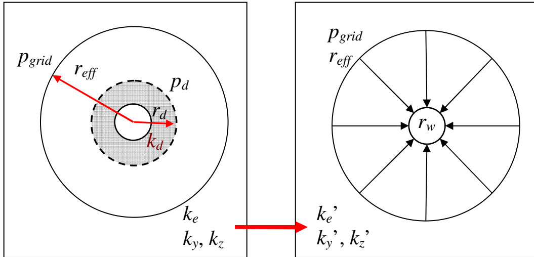
Fig. 2.3 Estimate formation damage effect by effective permeability
