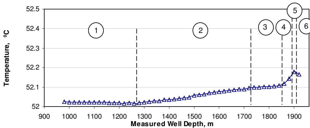
Fig. 5.6 Use measured temperature to separate reservoir for inversion
