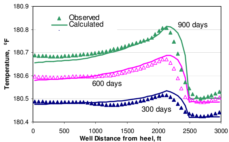
Fig. 4.34 Matched temperature data of water injection example
