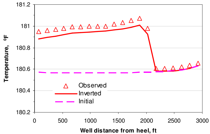
Fig. 4.14 Matched temperature data from L-M method, homogenous initial
