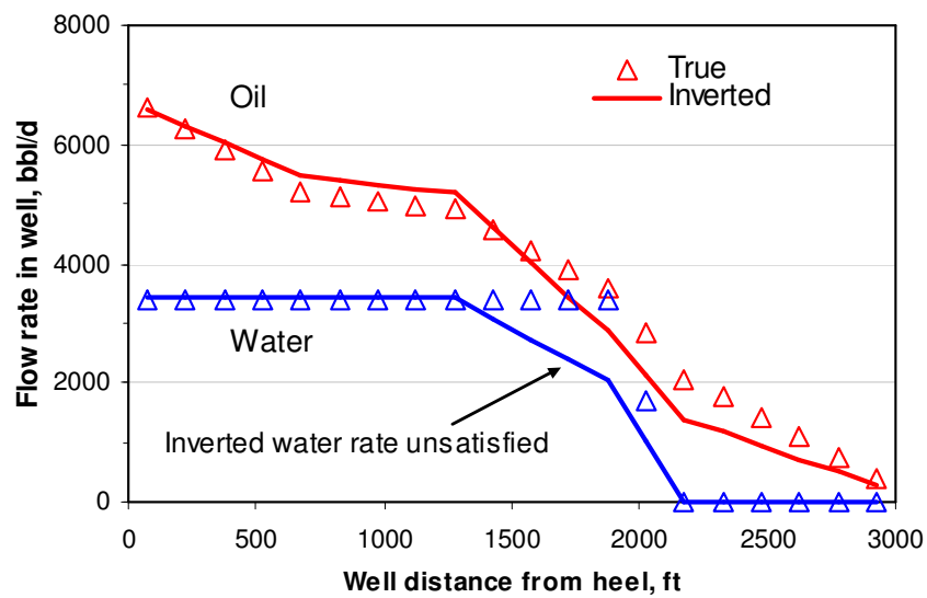
Fig. 4.16 Inverted oil and water flow rate profiles from L-M method, homogenous initial
