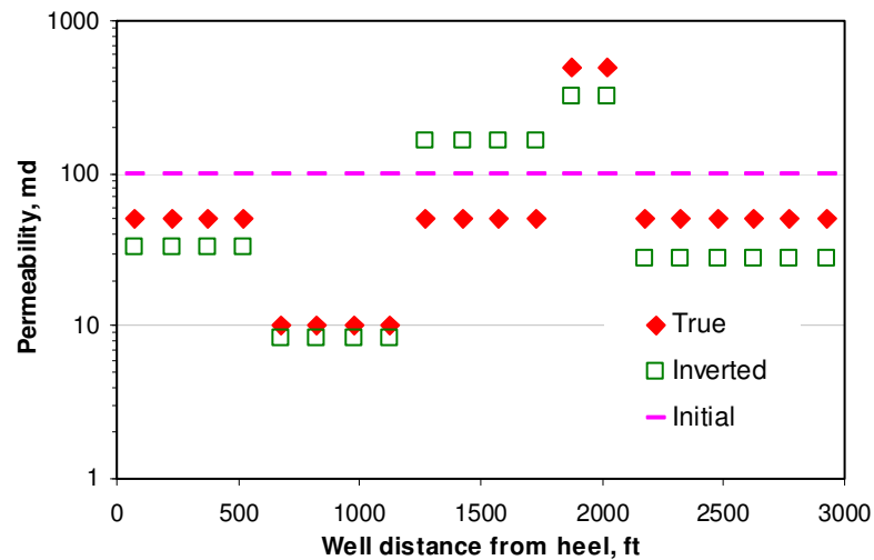
Fig. 4.17 Inverted permeability distribution from L-M method, homogenous initial
