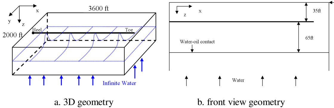
Fig. 4.1 Reservoir geometry information of bottom water driving case
