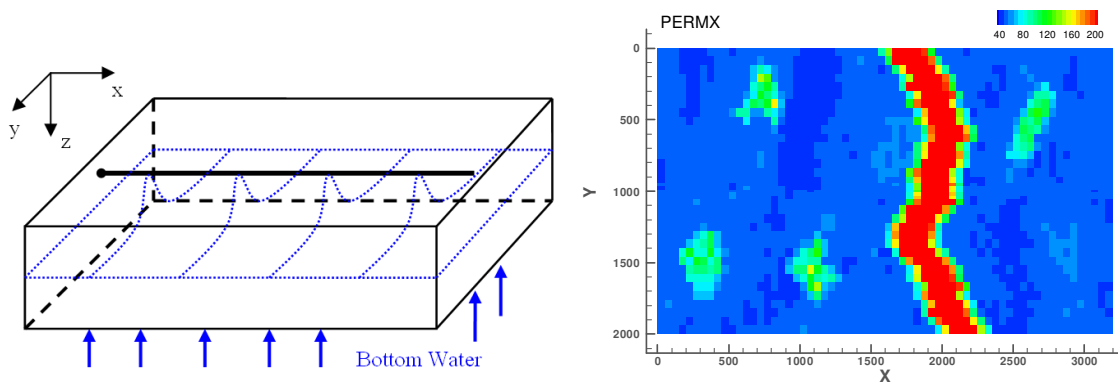
Fig. 5.24 Reservoir geometry and 2D permeability distribution
