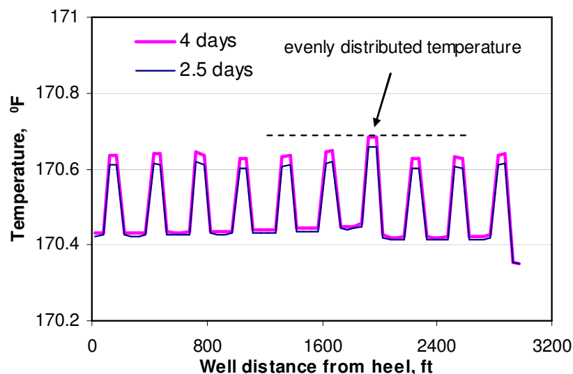
Fig. 5.28 Observe temperature feedback after controlling ICV at high inflow section
