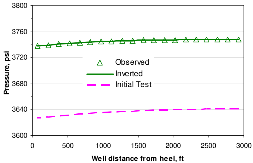
Fig. 3.2 Observed and inverted pressure data at 60 days
