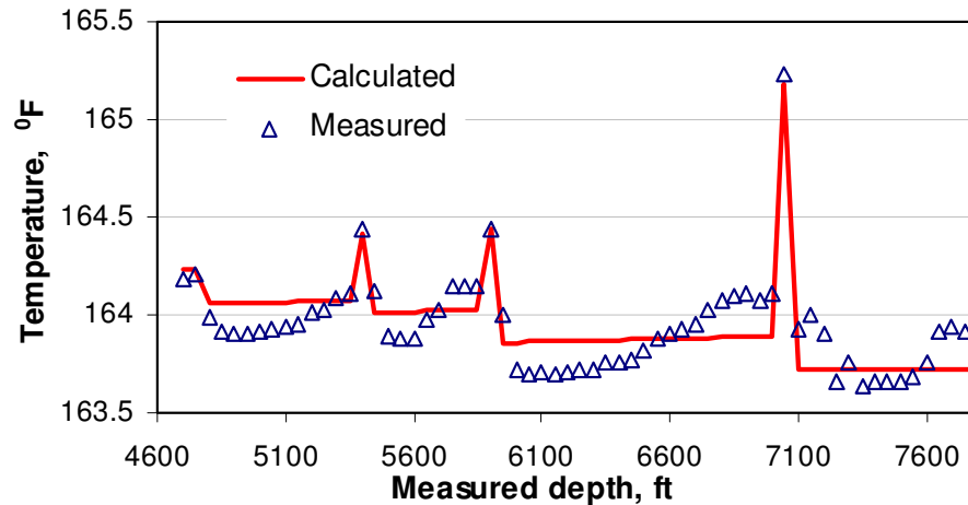
Fig. 5.18 Calculated temperature matches the trend of measured data
