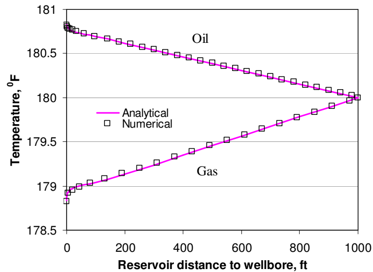
Fig. 2.7 Reservoir temperature distribution
