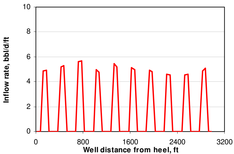
Fig. 5.49 Inflow rate distribution after ICV operation
