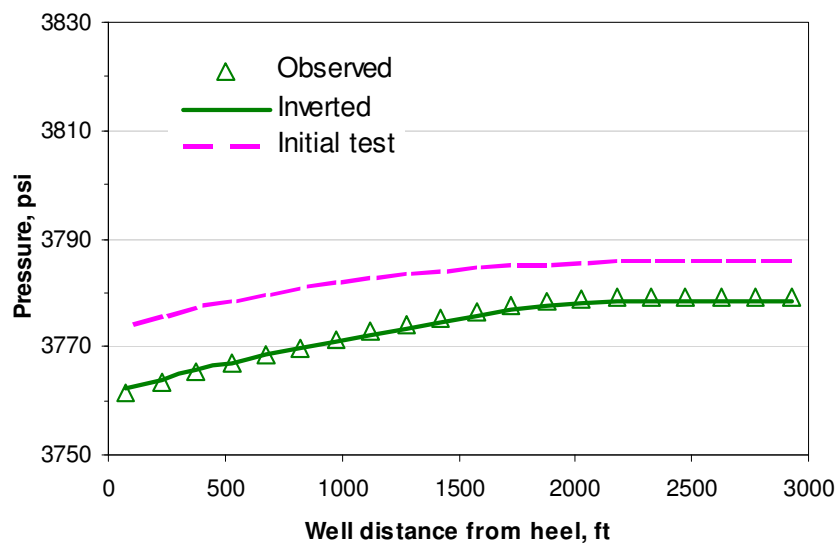
Fig. 4.24 Matched pressure data from MCMC method
