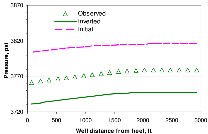
Fig. 4.15 Matched pressure data from L-M method, homogenous initial
