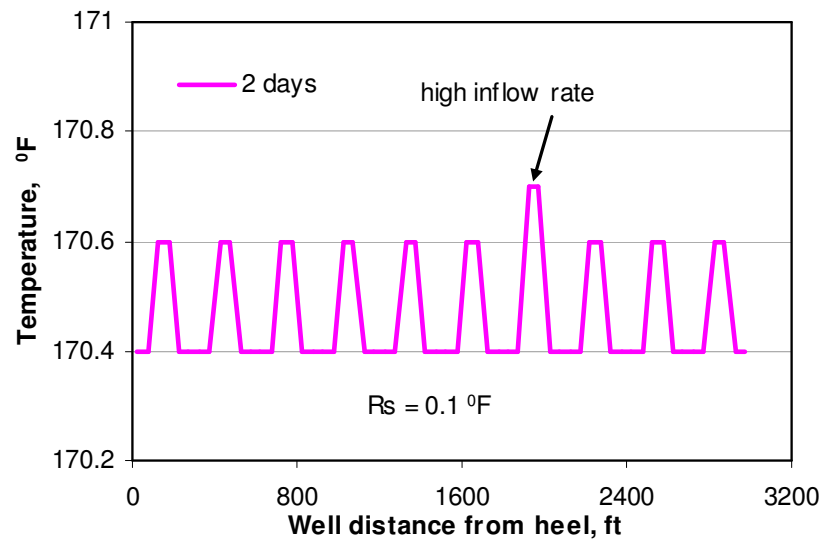
Fig. 5.39 May identify high inflow sections at 2 days, R_s = 0.1 °F
