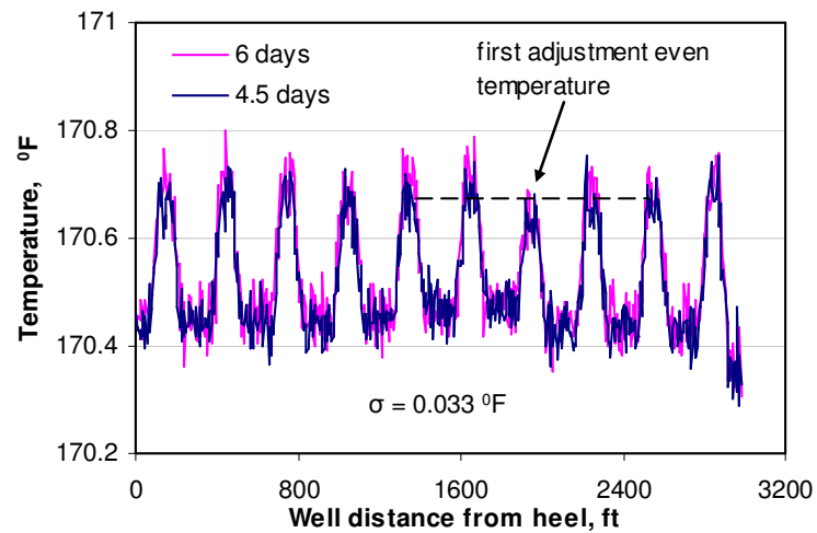
Fig. 5.41 Temperature achieves design, \sigma = 0.033 °F
