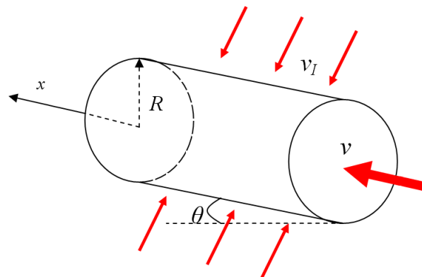
Fig. 2.1 Differential volume element of a wellbore
