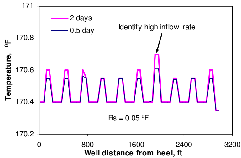
Fig. 5.35 Identify high inflow sections at initial, R_s = 0.05 °F
