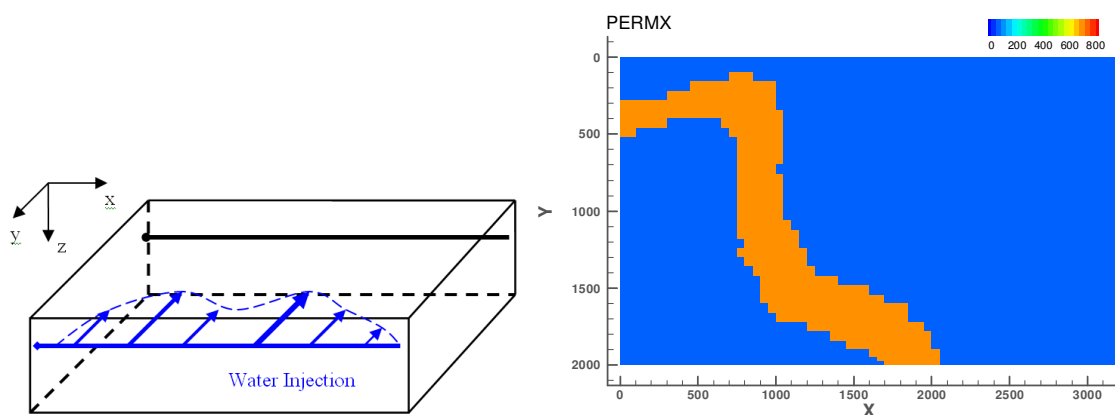
Fig. 5.44 Reservoir geometry and 2D permeability distribution used in example 2
