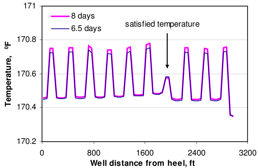
Fig. 5.31 Second ICV operation to meet the desired temperature
