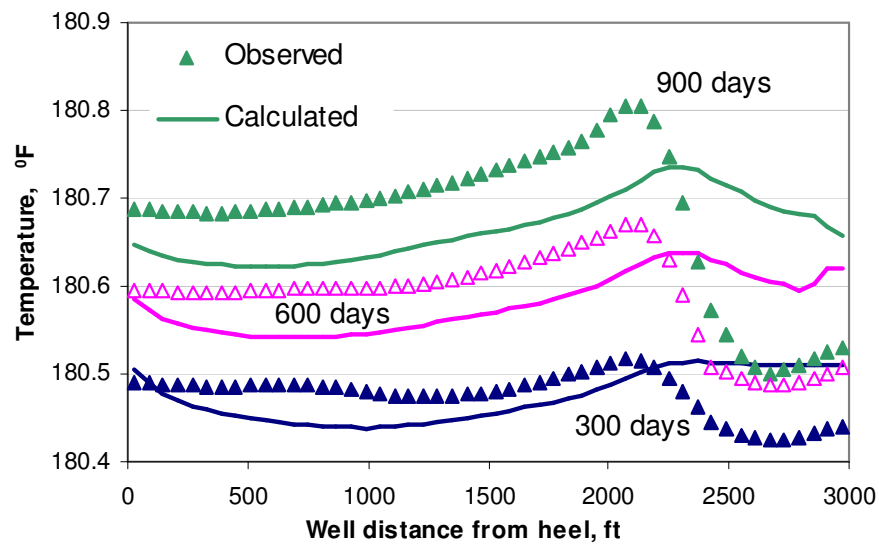
Fig. 5.61 Calculated temperature fails to match observation
