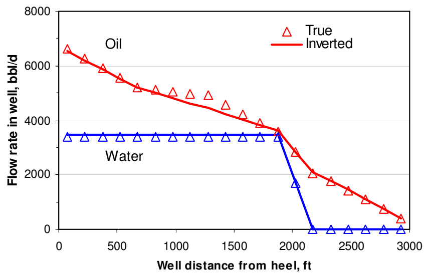
Fig. 4.20 Inverted oil and water flow rate profiles from L-M method, 2-value initial
