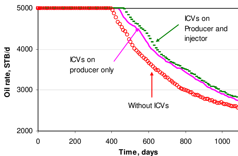
Fig. 5.50 Daily oil rate shows the production improvement
