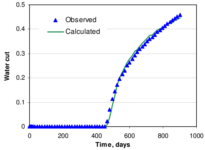
Fig. 5.56 Calculated water-cut history matches observation
