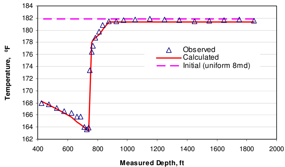
Fig. 5.2 Calculated temperature matches the measured data
