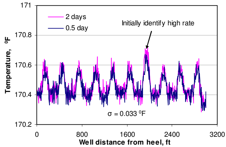
Fig. 5.40 Identify high inflow sections at initial, \sigma = 0.033 °F
