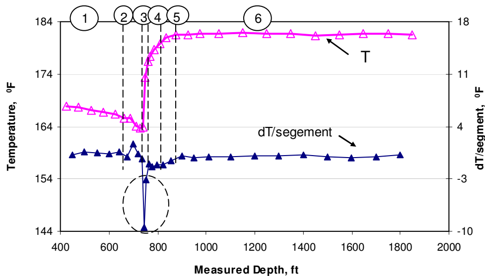
Fig. 5.1 Analysis on measured temperature
