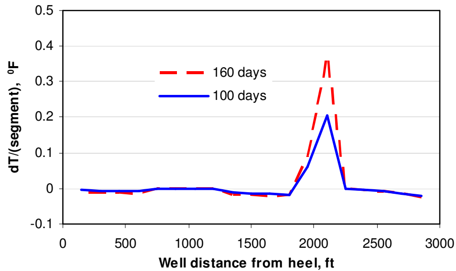
Fig. 4.7 Temperature derivative in wellbore
