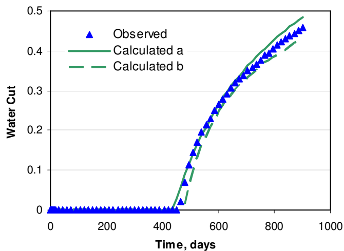
Fig. 5.59 Matching water-cut history
