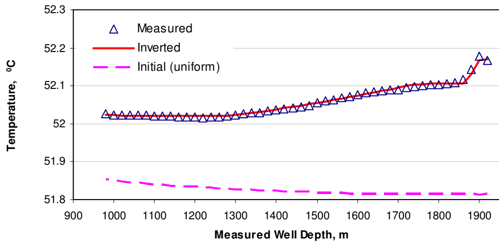
Fig. 5.7 Match measured temperature data of water entry oil well example
