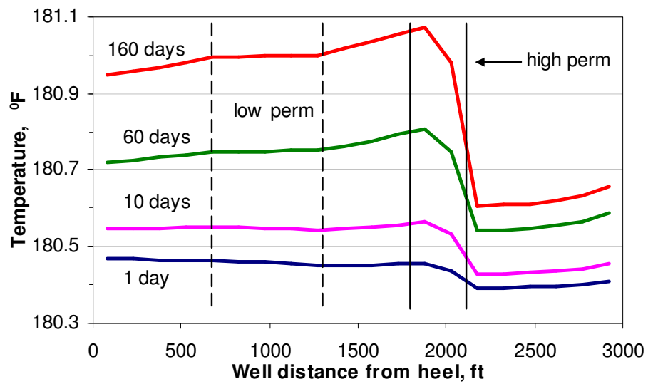
Fig. 4.5 Temperature distribution in wellbore
