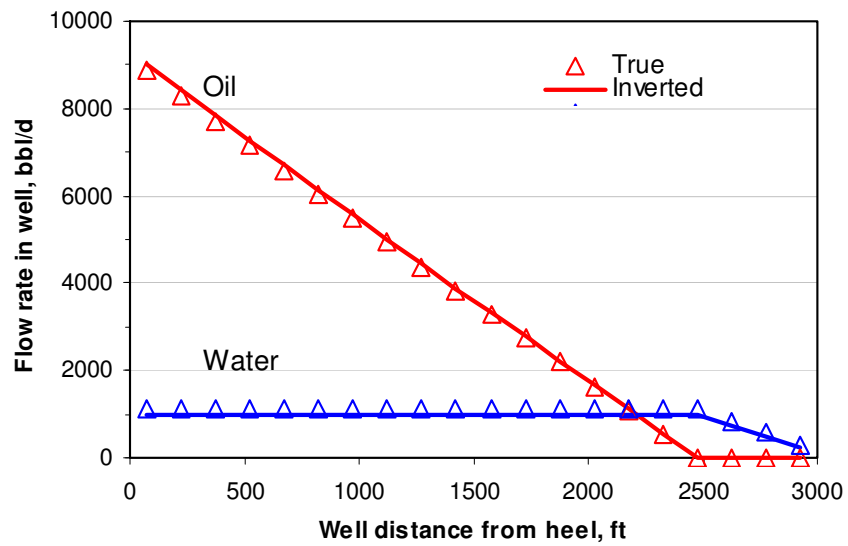
Fig. 3.4 Observed and inverted flow rates of validation case
