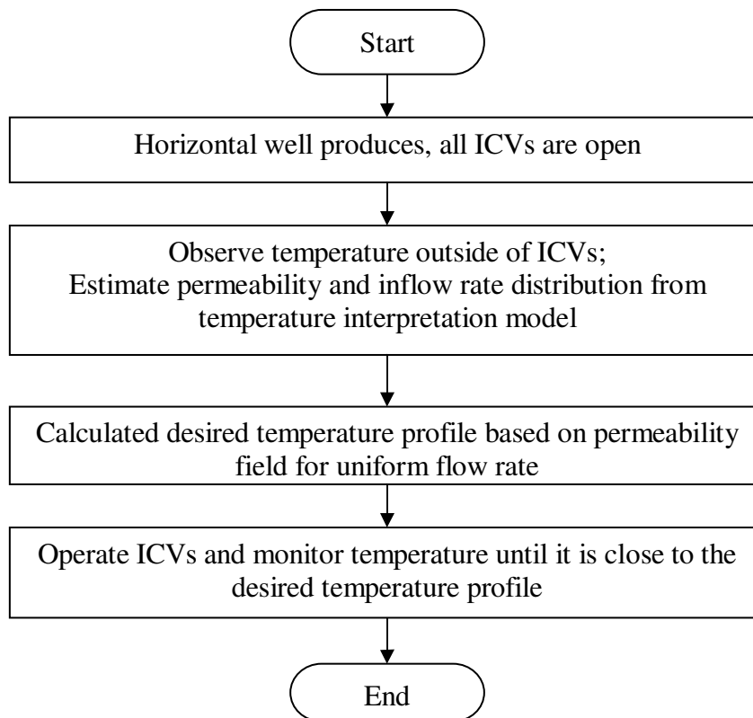
Fig. 5.21 Optimization procedure of operation on ICV from temperature feedback
