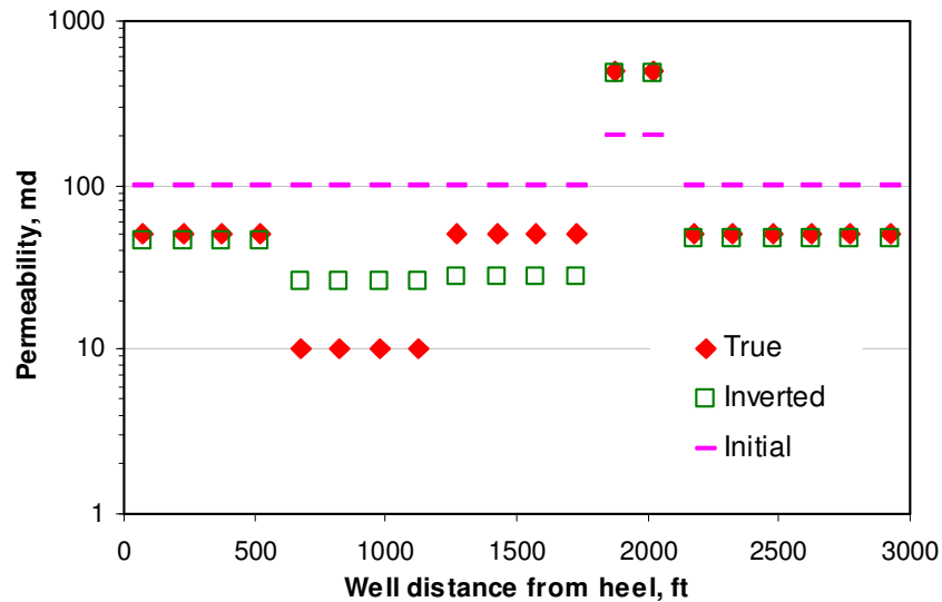
Fig. 4.21 Inverted permeability distribution from L-M method, 2-value initial
