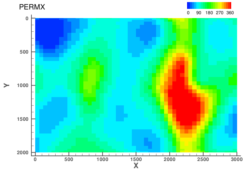
Fig. 4.28 2D permeability distribution
