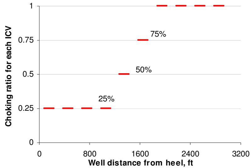
Fig. 5.47 Choking index ratio changes along wellbore
