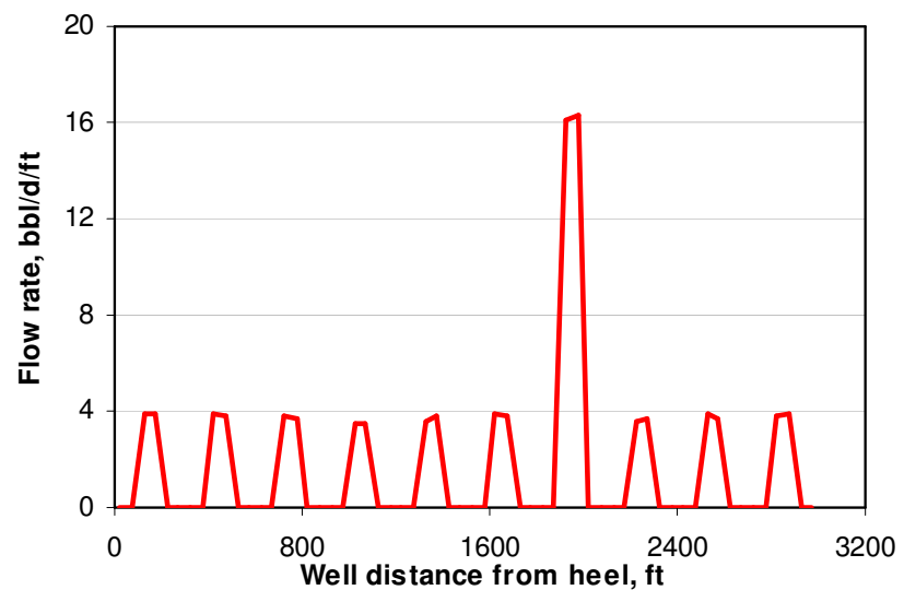
Fig. 5.26 Flow rate profile before operating ICVs
