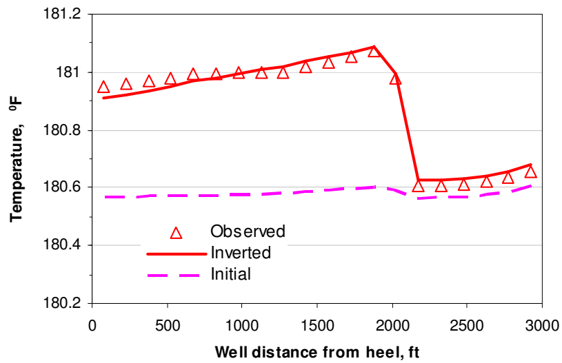
Fig. 4.18 Matched temperature data from L-M method, 2-value initial
