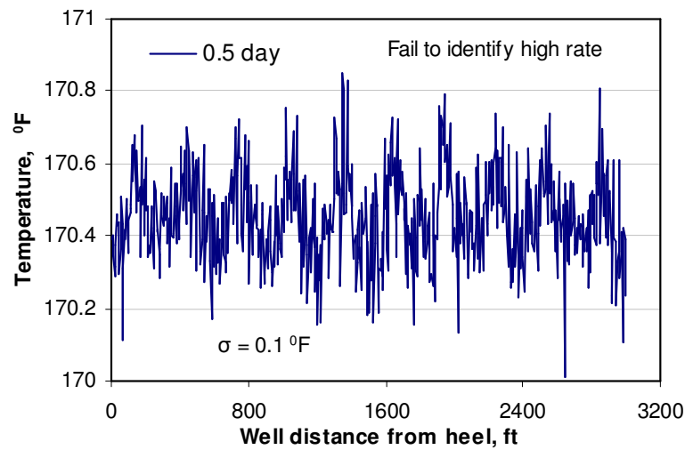
Fig. 5.42 Failure to identify high inflow sections at 0.5 day, \sigma = 0.1 °F
