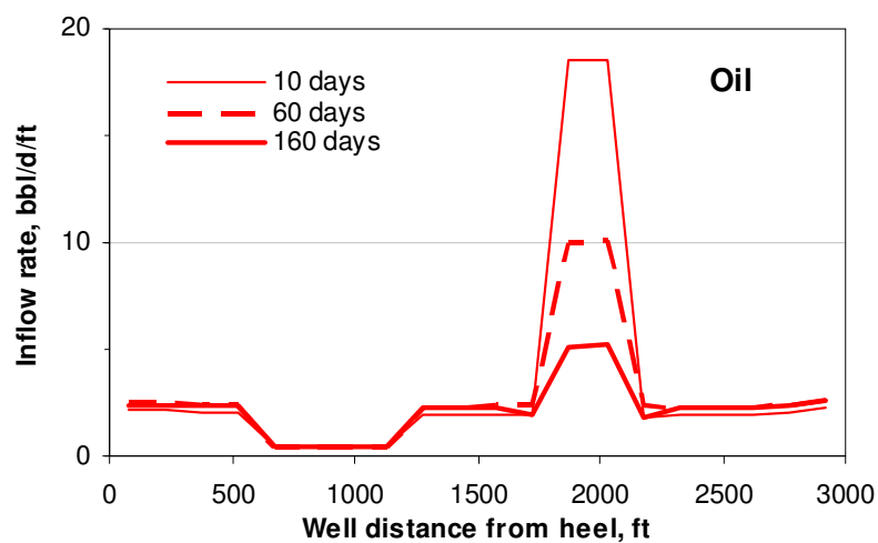
Fig. 4.3 Oil inflow rate distribution
