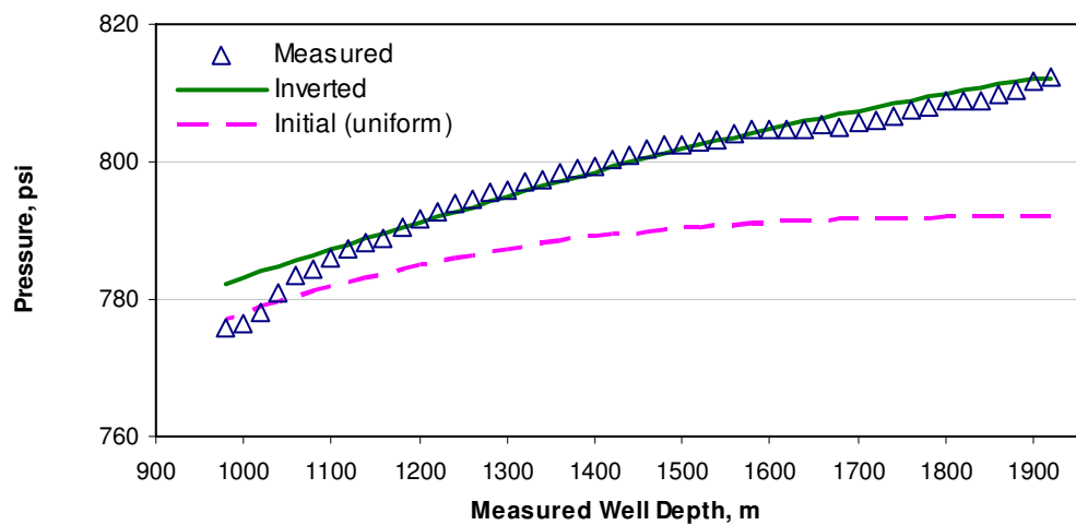
Fig. 5.8 Match measured pressure data of water entry oil well example
