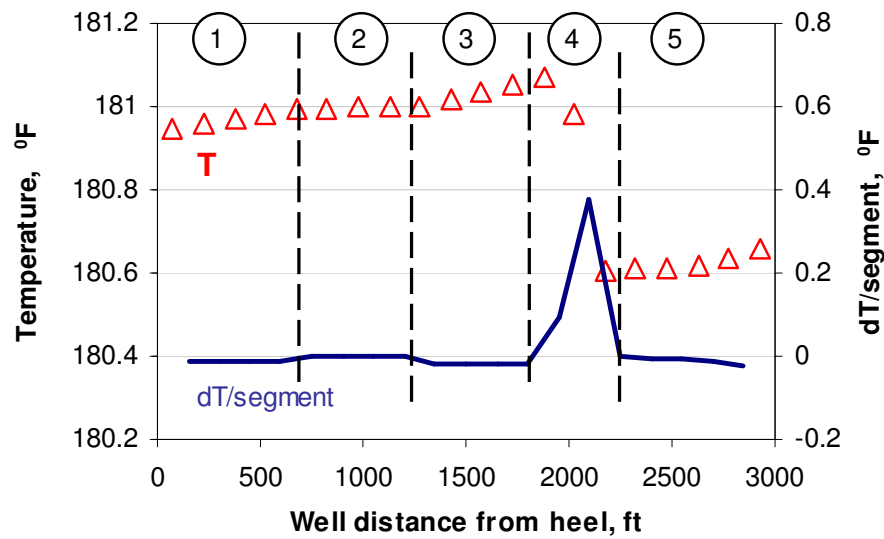
Fig. 4.12 Separate reservoir to sections by temperature data
