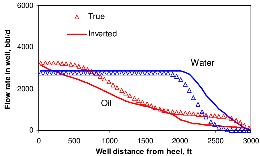
Fig. 5.62 Downhole flow rates may not be predicted correctly by history matching only
