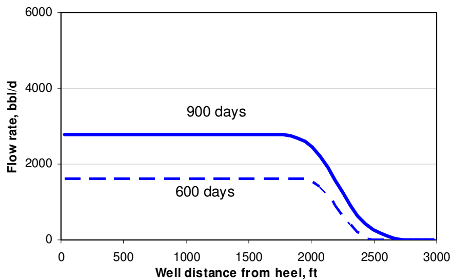
Fig. 4.30 Water flow rate profiles in tubing
