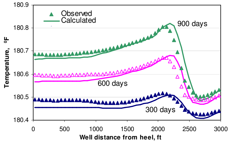
Fig. 5.57 Calculated temperature matches observation
