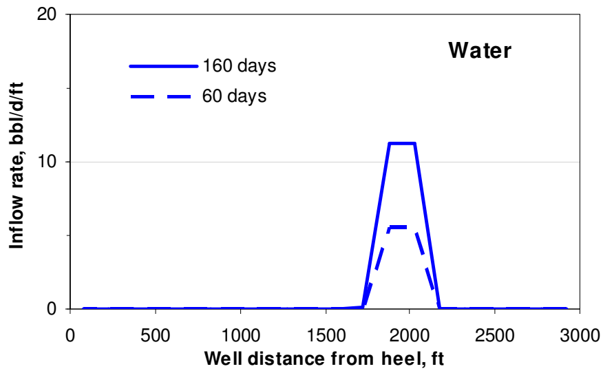
Fig. 4.4 Water inflow rate distribution
