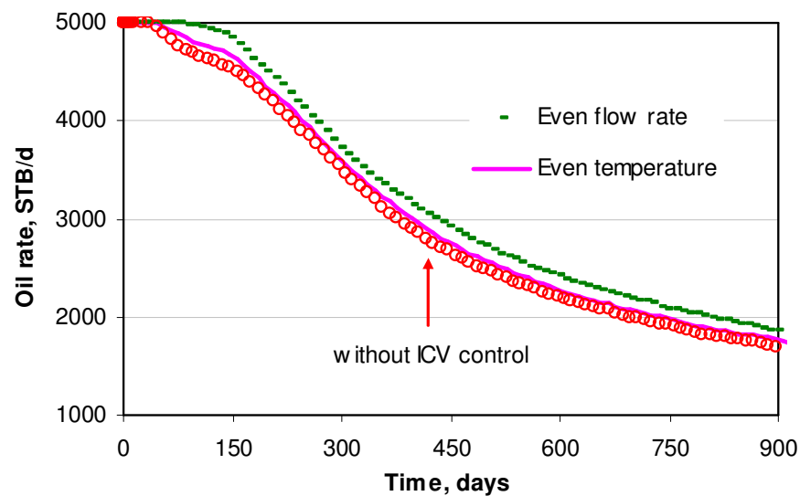
Fig. 5.33 Daily oil rate vs. time at three conditions
