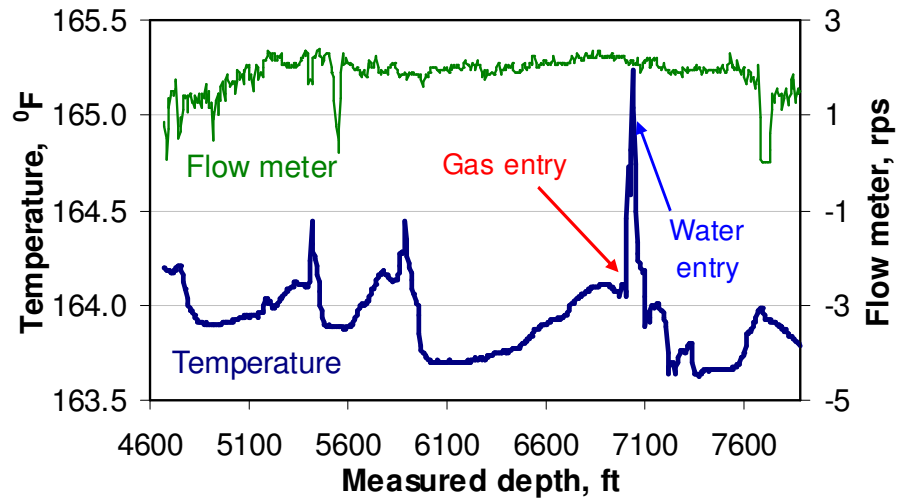
Fig. 5.16 Measured temperature and flow meter data
