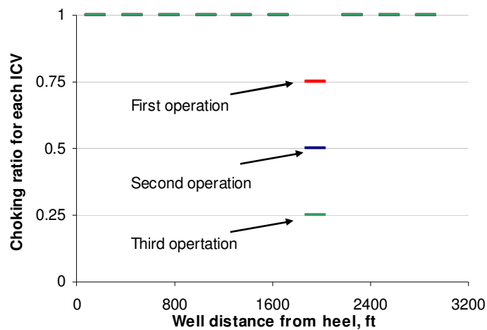
Fig. 5.27 Choking index ratio changes in simulation at different ICV stages
