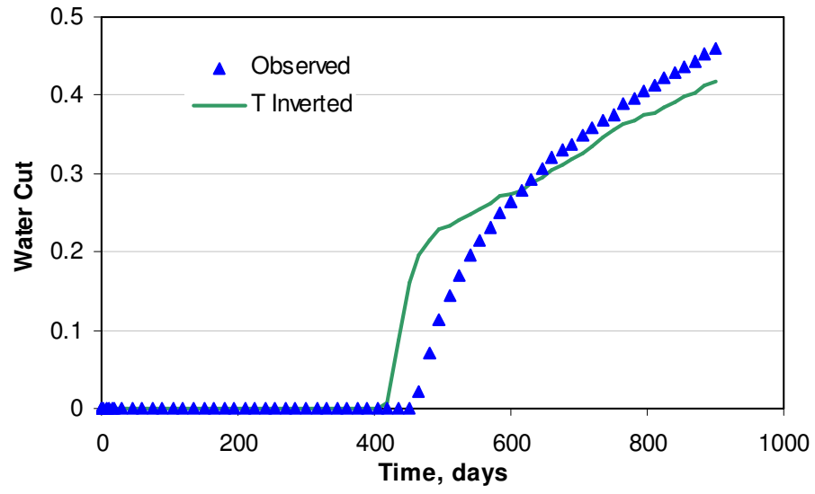
Fig. 4.38 Inverted water cut vs. observation
