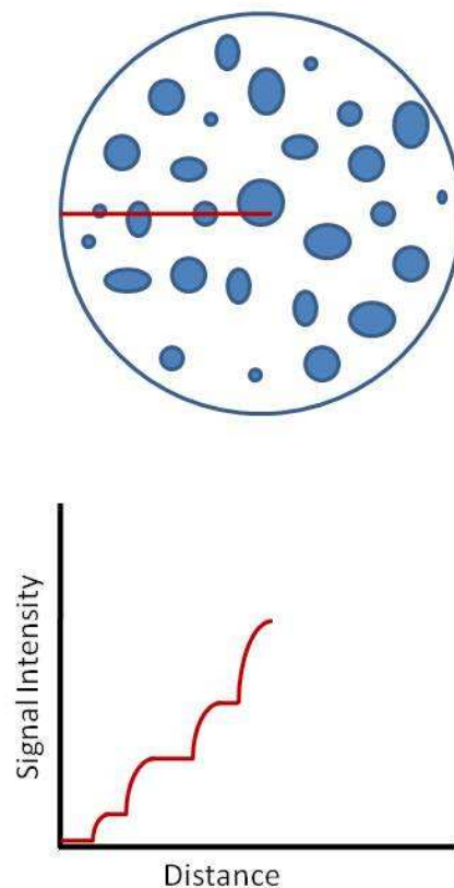
Figure 3.6. Diagram of a sphere showing a potential 1D path of analyte transport and the corresponding signal intensity
