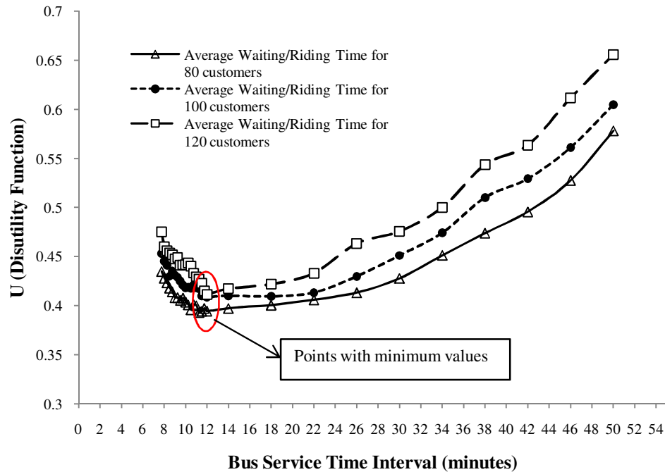
Figure 29: Disutility function variation with the different number of passengers.
