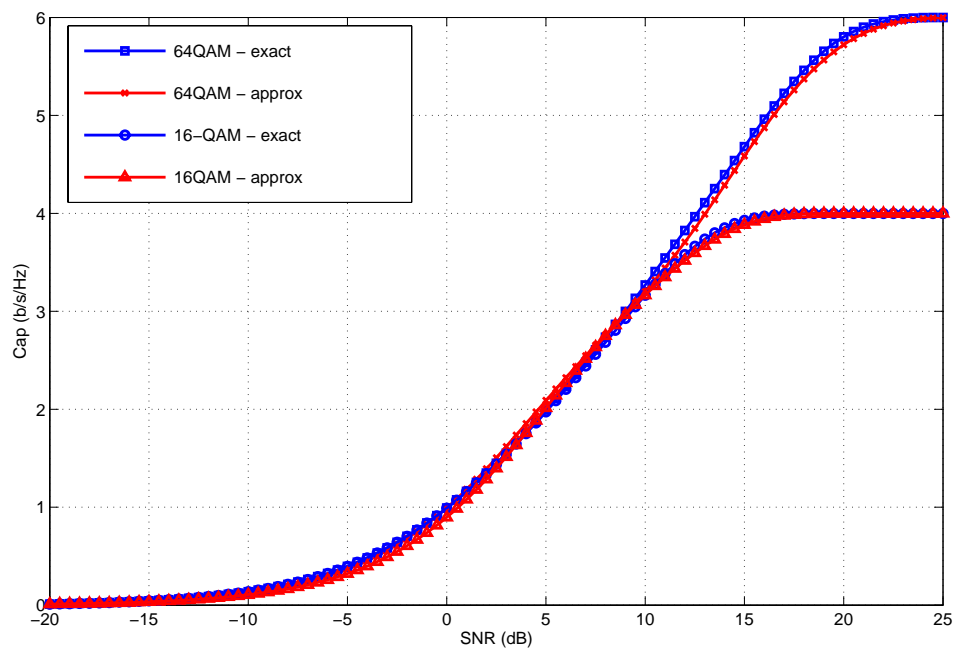
Fig. 30. Exact and tighter capacities for 16-QAM and 64-QAM
