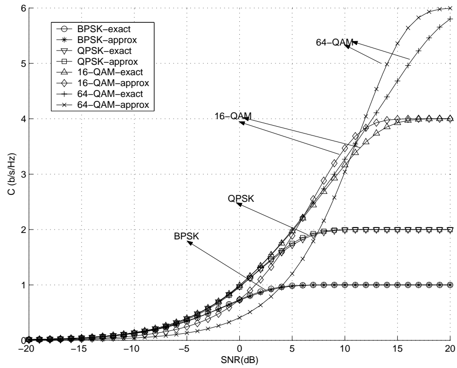
Fig. 29. Exact and appromixate capacities for BPSK, QPSK, 16-QAM and 64-QAM
