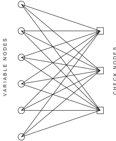
Fig. 2. Bipartite graph of an LDPC code
