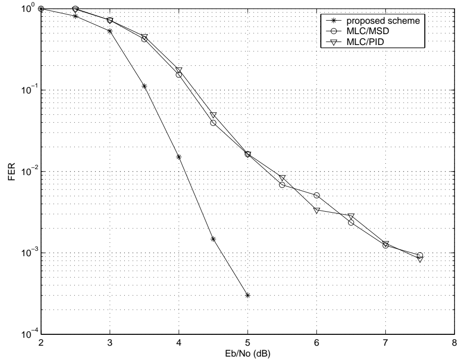
Fig. 8. Comparison of our scheme (FER) to the best MLC/MSD and MLC/PID schemes for gray-mapped 4-PAM R=0.5 (1000,500) LDPC and d_l = 15 for AWGN
