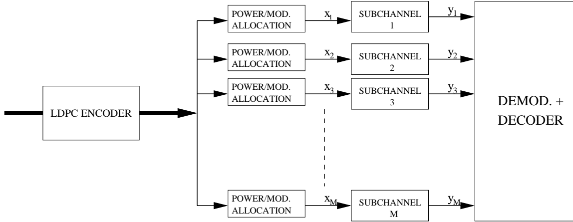
Fig. 28. Adaptive modulation system description
