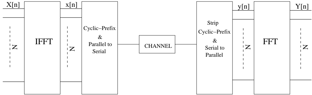
Fig. 1. Block diagram of an OFDM system
