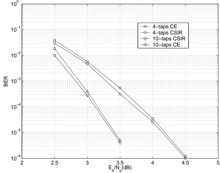
Fig. 25. BER of a rate-0.5 length 32768 IRA code BPSK and OFDM with 1024 sub-carriers and 4, 10 multipaths on an NCSI system with channel estimator and with CSIR
