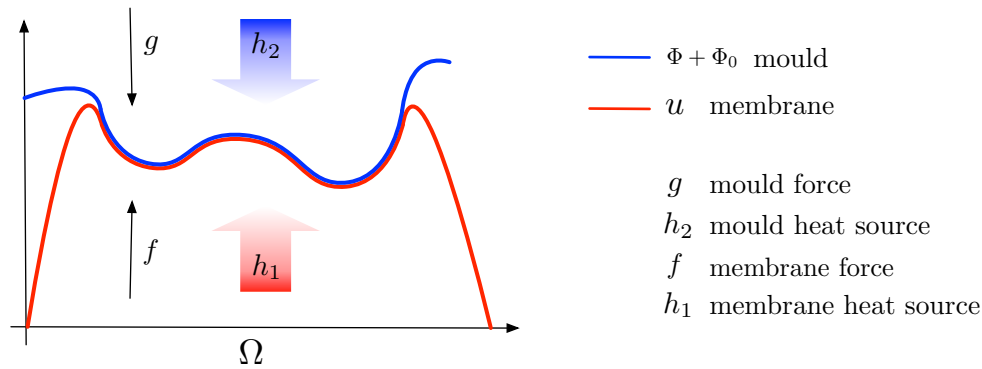
Figure 1: Contact of the membrane and the mould.
