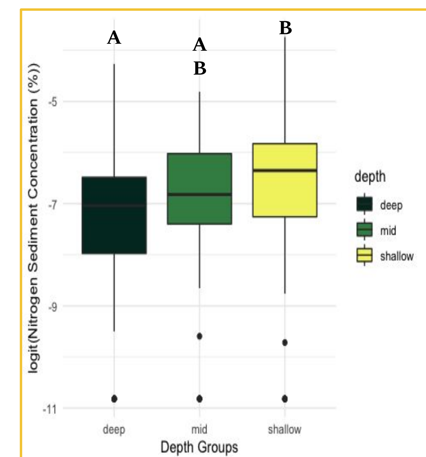
Figure 5a: Boxplot of % carbon concentrations in sediment across the subdivisions of all wetlands. Means are significantly different (ANOVA: p < 0.05 ). Significant differences between means denoted with letters (Tukey: p < 0.05 ). 5b: Boxplot of % nitrogen concentrations in sediment across the subdivisions of all wetlands. Significant differences between means denoted with letters (Tukey: p < 0.05 ).
