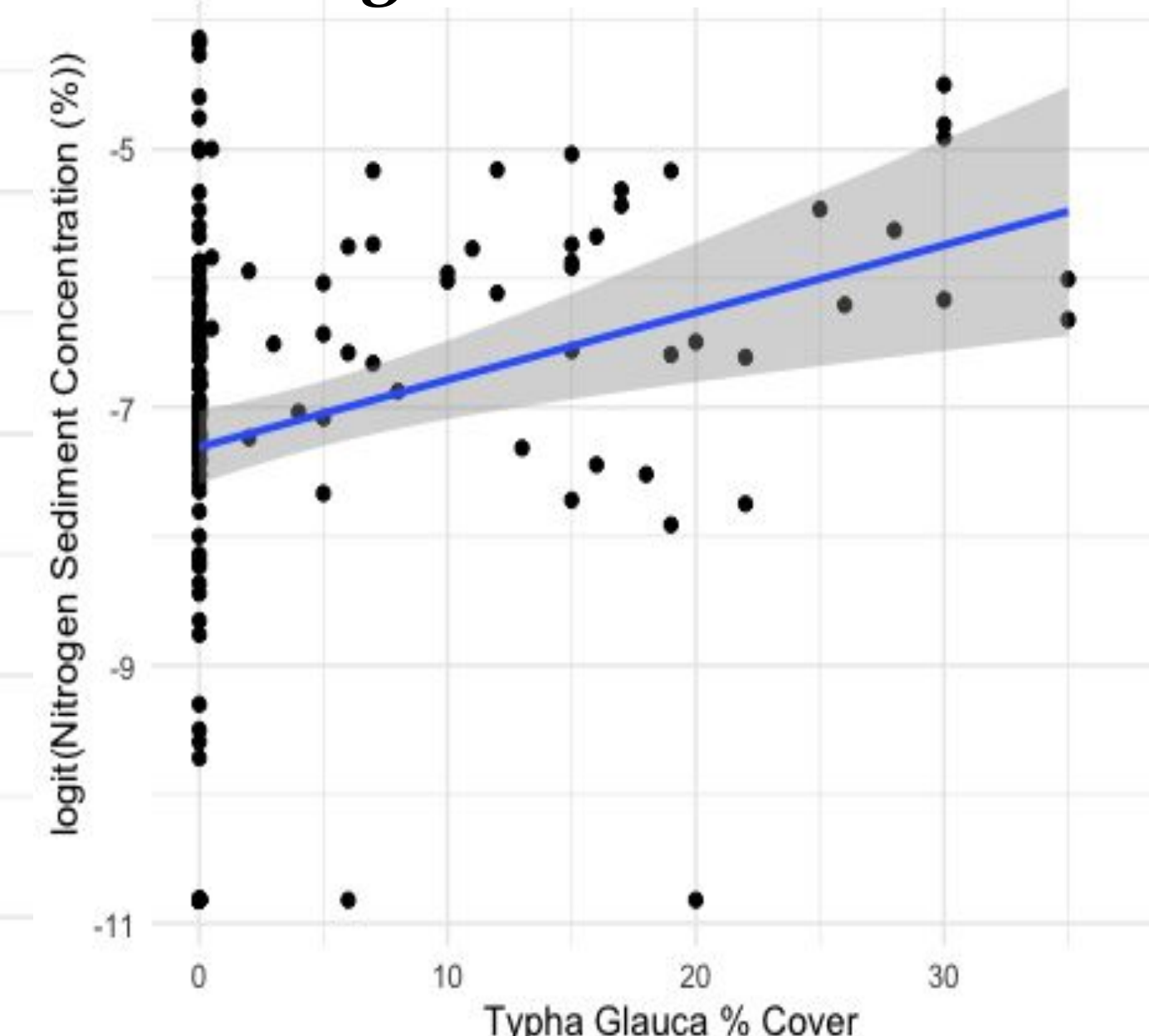
Figure 4a: Linear regression model of C% based on T. glauca % cover ( p < 0.05 , R^2 = 0.08 ). Figure 4b: Linear regression model of N% based on T. glauca % cover ( p < 0.05 , R^2 = 0.06 ).
