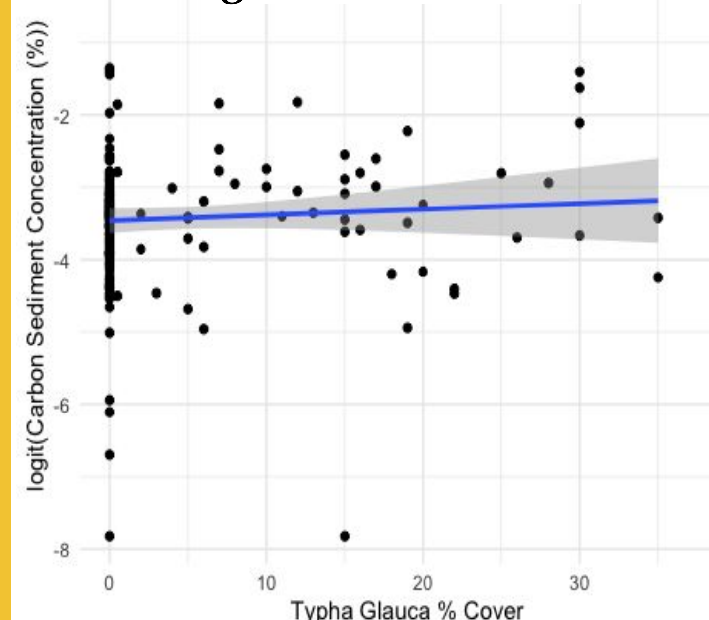
Figure 4a: Linear regression model of C% based on T. glauca % cover ( p < 0.05 , R^2 = 0.08 ). Figure 4b: Linear regression model of N% based on T. glauca % cover ( p < 0.05 , R^2 = 0.06 ).
