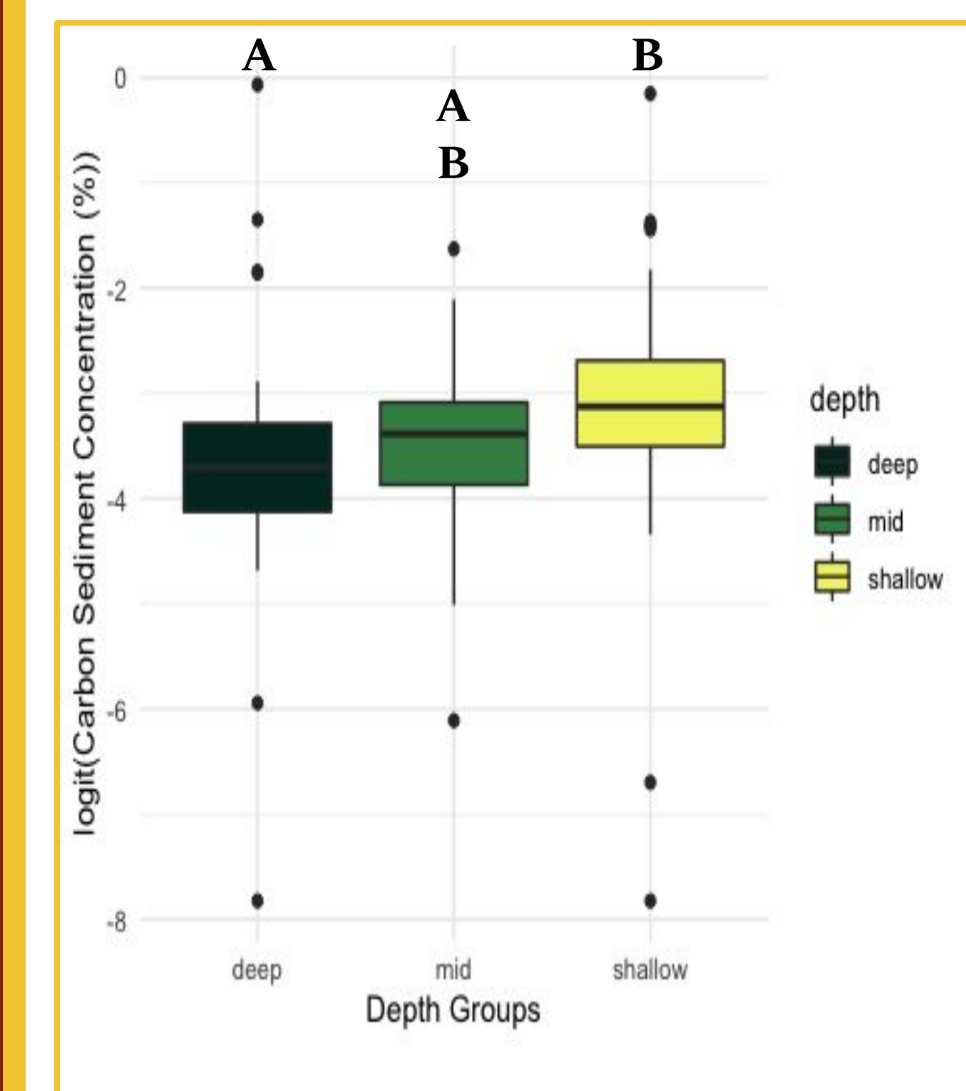
Figure 5a: Boxplot of % carbon concentrations in sediment across the subdivisions of all wetlands. Means are significantly different (ANOVA: p < 0.05 ). Significant differences between means denoted with letters (Tukey: p < 0.05 ). 5b: Boxplot of % nitrogen concentrations in sediment across the subdivisions of all wetlands. Significant differences between means denoted with letters (Tukey: p < 0.05 ).
