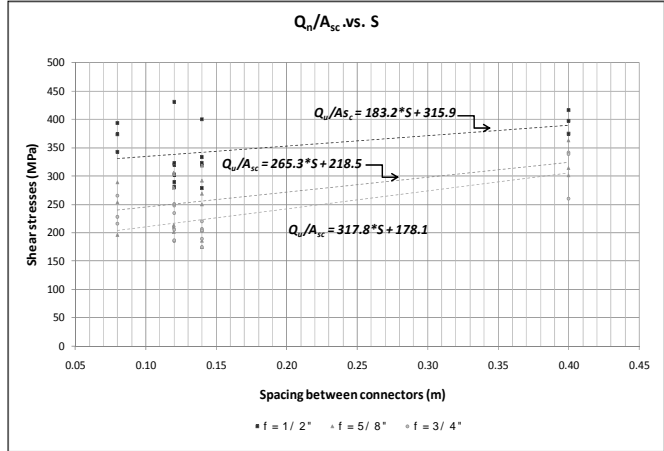
Figure 6. Q_u/A_{sc} cf S
