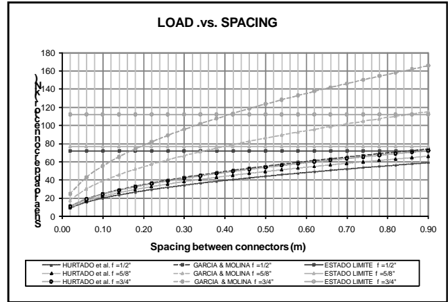
Figure 1. Comparative curves from formulations by Hurtado et al., and García & Molina.
