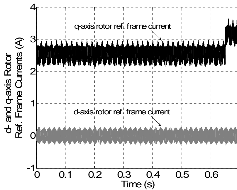
Fig. 5.11. Steady-state and transient behavior of the simulated q - and d -axis rotor reference frame currents when i_{ds}^{ref} = 0 under 0.5 N·m load torque.
