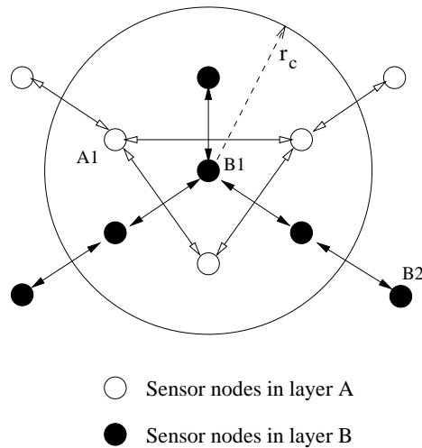
Fig. 22. Concept of Layer Communication
