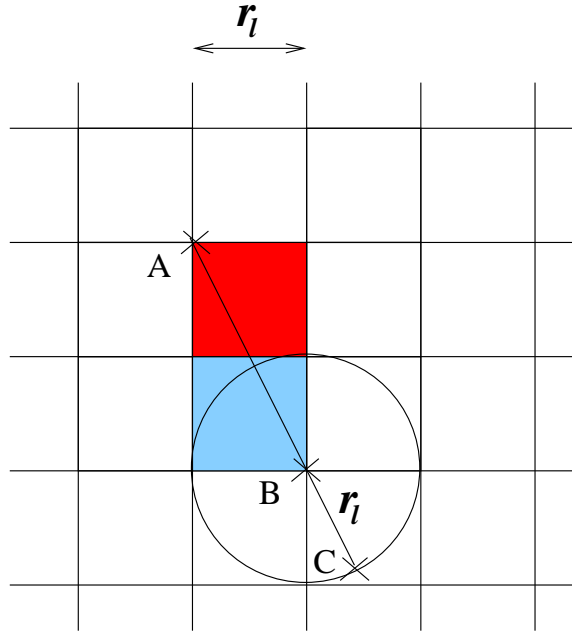
Fig. 12. Maximum Distance of Two Closest Working Nodes
