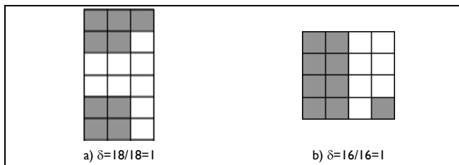
Figure 1. Evaluation of index \delta in activities involving breakage
