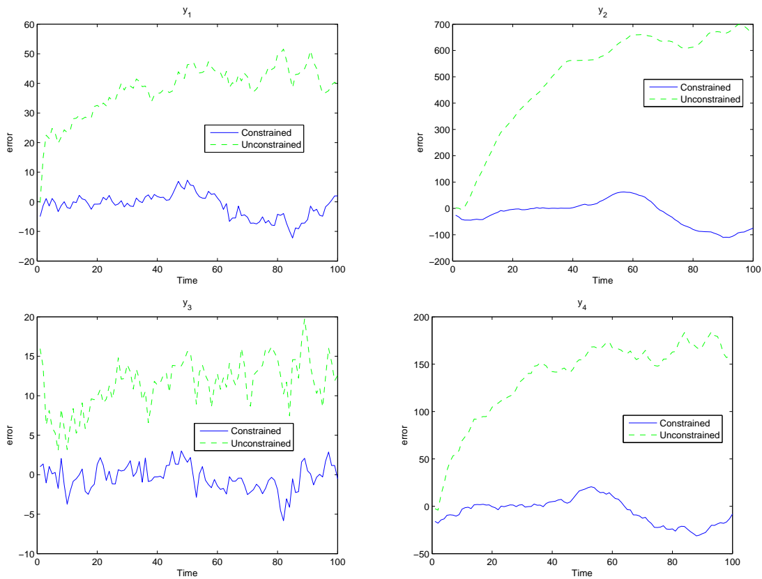
Fig. 5.: These are the errors in the predicted outputs of y_1 and y_2 , using conventional EM (dashed) and constrained EM (solid), for the synthetic data. The errors are the differences between the predictions of the estimated model and the observed values. We can see that conventional EM produces models that have large prediction errors and thus poor predictive power.
