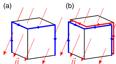
Figure 5. a) Schematic picture of an “extrinsic” second-order topological insulator consisting of a 3D topological insulator placed in a magnetic field in a generic direction, as proposed by Sittte et al. [28] Each surface has a finite flux and there are chiral modes along hinges that touch two faces with opposite sign of the magnetic flux. b) The gapless hinge modes may be removed by decorating some of the crystal faces with a two-dimensional anomalous quantized Hall insulator.
