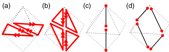
Figure 13. a) Construction of second-order boundary states for a crystal with \mathcal{M}_z and \mathcal{R}_{2,z} symmetries by placing 2D topological superconductors on the two 2-cells in the mirror plane. b) Placing 2D superconductors on the four 2-cells perpendicular to the mirror plane is not allowed, because the copropagating chiral Majorana modes at the interior boundaries between cells can not be gapped out. c) Third-order boundary states with well-defined \mathcal{R}_{2,z} parity can be obtained by placing 1D superconductors at the two 1-cells along the rotation axis. d) Extrinsic third-order boundary states, consisting of pairs of corner states with different \mathcal{R}_{2,z} parity, arise from 1D topological phases at the four boundary 1-cells outside the mirror plane.
