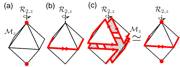
Figure 7. A topological 3D superconductor with mirror and twofold rotation symmetry admits a) Majorana corner modes at the rotation axis or b) a pair of copropagating Majorana hinge modes at the mirror plane. The difference between these two boundary signatures is a matter of crystal termination: c) The higher-order boundary modes in a crystal that has corner states as well as hinge modes are extrinsic.
