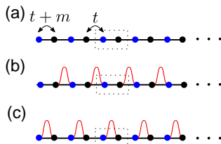
Figure 2. a) Without particle–hole symmetry, the model (1) describes a 1D lattice with a two-atom unit cell and nearest-neighbor hopping amplitudes that alternate between t and t + m . b) In the “topological phase” -2t < m < 0 Wannier functions are localized between unit cells, whereas c) they are localized in the center of the unit cells if m < -2t or m > 0 . The two patterns cannot be smoothly deformed into each other in the presence of inversion symmetry.
