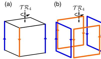
Figure 4. a) Configuration of chiral hinge modes of a 3D crystal with \mathcal{T}\mathcal{R}_4 symmetry. b) Configurations of chiral hinge modes that can be obtained by “decorating” the boundary have an even number of chiral modes at each hinge.
