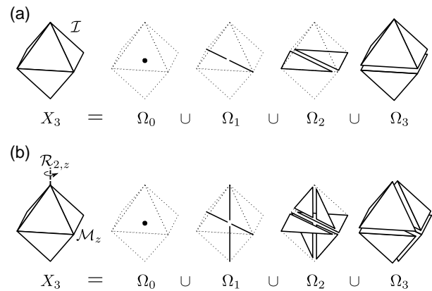
Figure 10. G -symmetric cellular decompositions of the octahedron for the crystalline symmetry group a) G generated by inversion \mathcal{I} and for b) G = C_{2h} , generated by mirror \mathcal{M}_z and twofold rotation symmetry \mathcal{R}_{2,z} .
