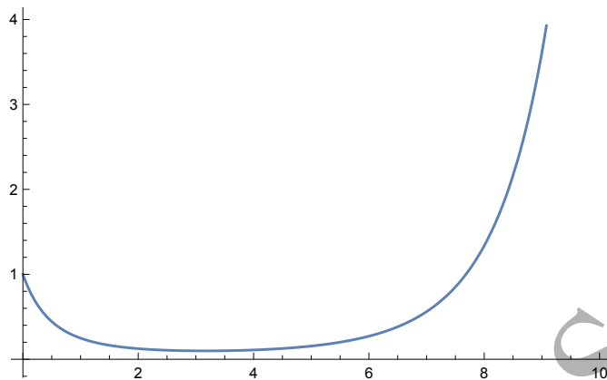
Figure 2. Amplitude f_q in (37) from (38) as a function of q . See discussion in text.
