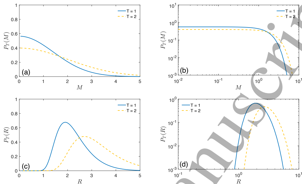
Figure 1. Probability density functions of the extremal behaviour of standard Brownian motion. Panels (a,b) show the Gaussian law (2) for the maximum M on linear and log-log scales. Panels (c,d) show the probability density (3) for the range. In all panels we depict the functions for the observation times T = 1 and T = 2 . We chose D_0 = 1 .
