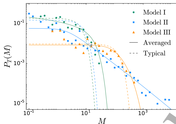
Figure 6. Comparison of the probability density functions P_T(M) (solid curves) and the estimate P_T^{(\text{typ})}(M) from (85) of the typical behaviour (dashed curves) for the three random diffusivity models. Symbols represent the empirically renormalised histograms obtained from Monte Carlo simulations with 10^2 runs (the time step of 10^{-2} ). We set D_0 = 1 , T = 100 , a = 1 , and D_B = 1 .
