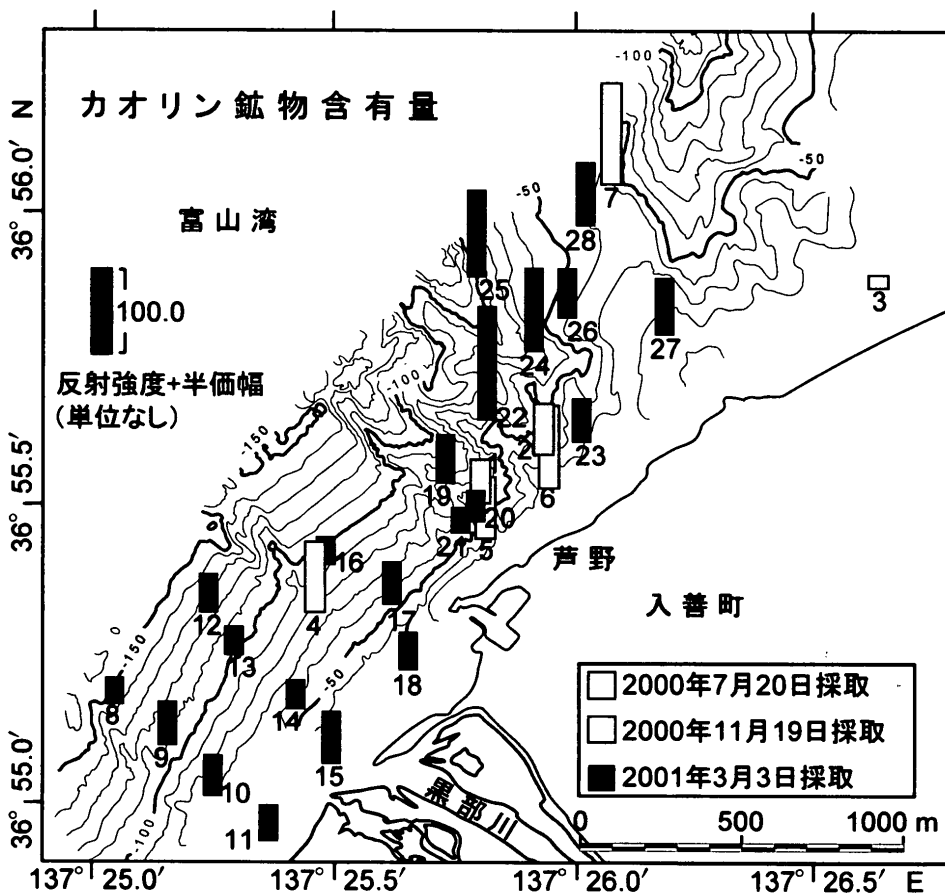
Fig. 12. Distribution map of kaolin group minerals intensity in the sediments in Toyama Bay, by using XRD method. Intensity of kaolin group minerals (001) was calculated by the same method as Fig. 9.
