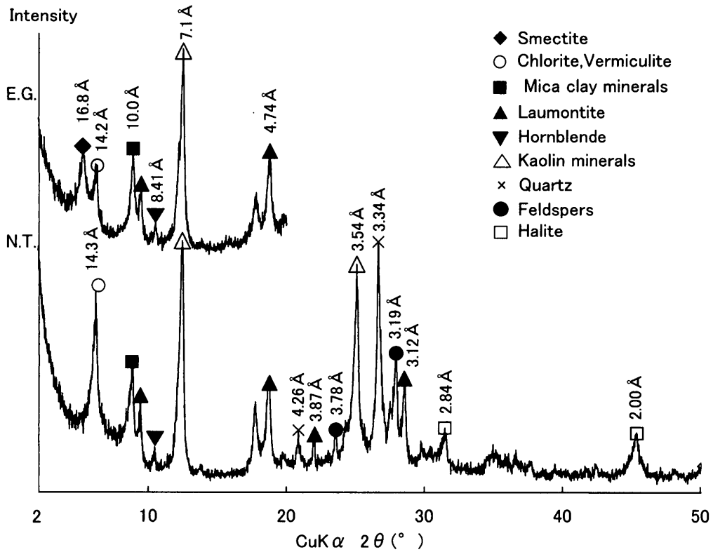
Fig. 8. X-ray powder diffraction (XRD) patterns of the sediments (<2 \mu m fraction) of the sample No. 22.
