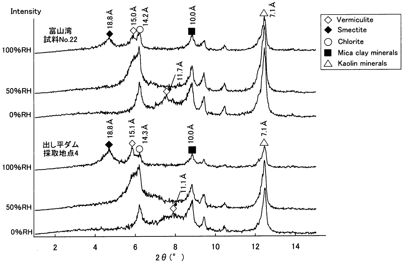
Fig. 13. X-ray powder diffractions (XRD) patterns of the sediments collected from Toyama Bay (Sample No. 22).
