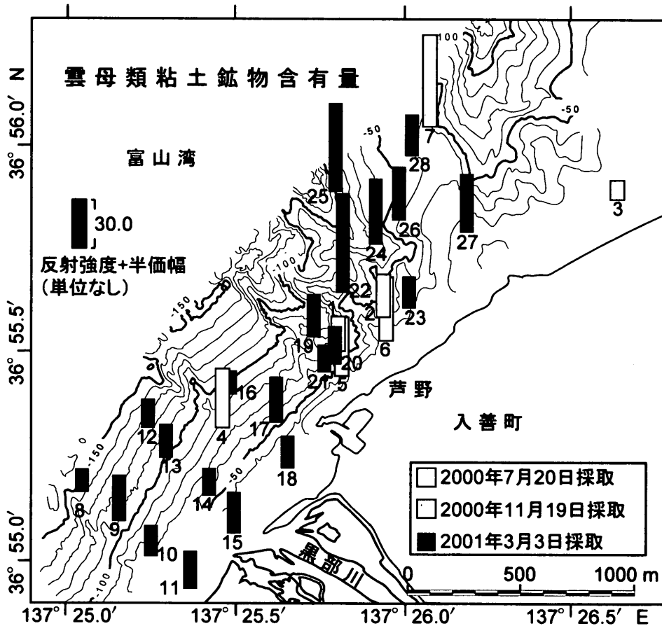
Fig. 11. Distribution map of mica group clay minerals intensity in the sediments in Toyama Bay, by using XRD method. Intensity of 10 Å (001) was calculated by the same method as Fig. 9.
