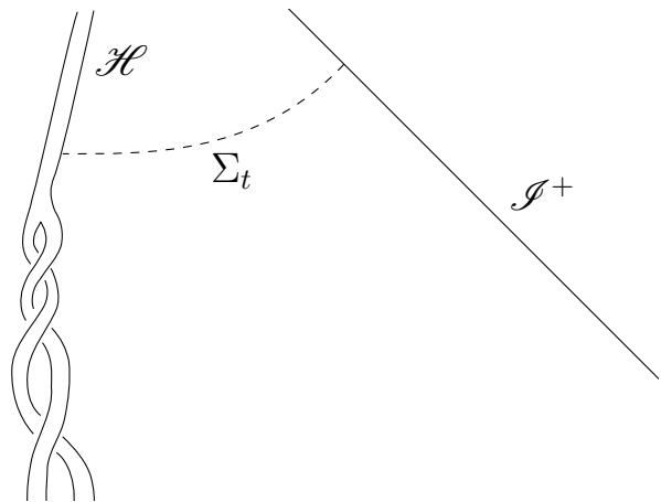
FIG. 1. A diagram of a BBH spacetime, showing the inner boundary formed by the horizon \mathcal{H} and the outer boundary formed by future null infinity \mathcal{I}^+ . Integrating Eq. (22) over the spacelike hypersurface \Sigma_t justifies the comparison of the horizon quantities and asymptotic quantities.
