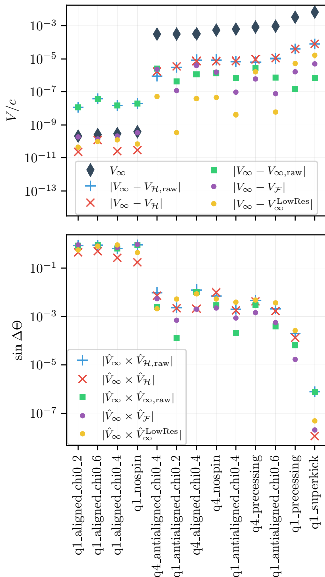
FIG. 3. A comparison of the CoM-corrected asymptotic recoil velocity \vec{V}_\infty with the CoM-corrected apparent horizon recoil velocity \vec{V}_H and the same recoil velocity measurements without the CoM correction, \vec{V}_{\infty,\text{raw}} and \vec{V}_{H,\text{raw}} . A comparison with the recoil velocity \vec{V}_F as computed for surrogate remnant models is also shown. The upper plot shows the absolute difference in magnitude. For reference, the value of V_\infty has been plotted as well. The lower plot shows the misalignment \sin \Delta\Theta , where \Delta\Theta is the angle between the one of the recoil velocity vectors and \vec{V}_\infty . For most systems, errors in the methods used to compute the recoil velocity dominate over the numerical resolution.
