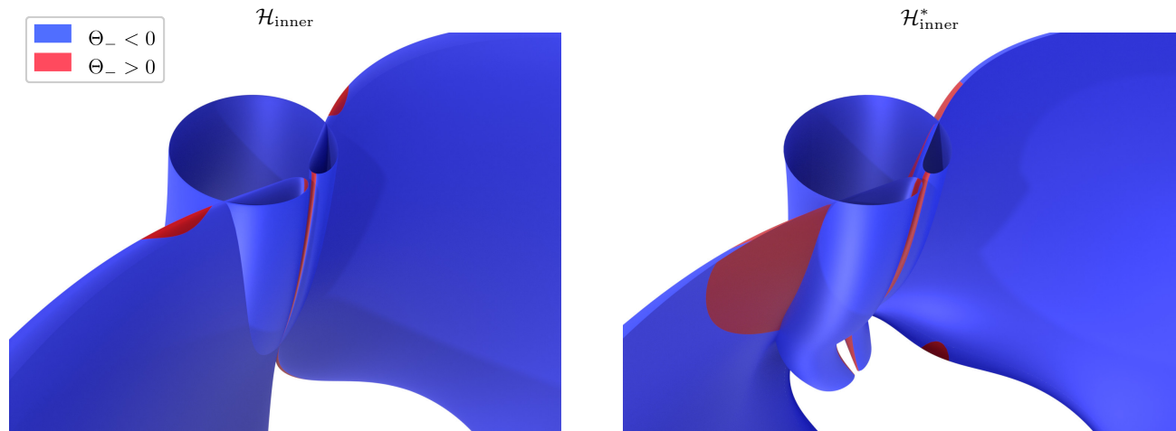
FIG. 20. Close-up of the top ends of the MOTTs shown in FIG. 19. The two world tubes smoothly join at this top end and the portions with \Theta_- < 0 connect across this merger.
