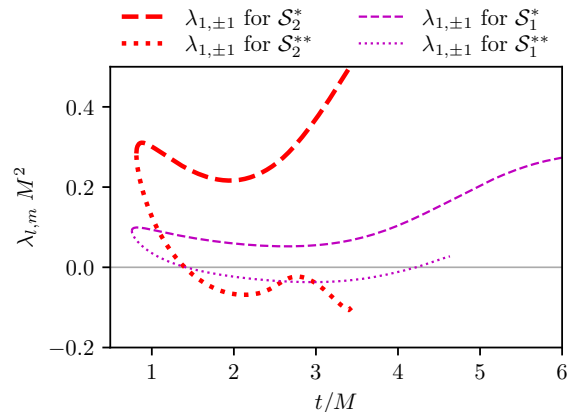
FIG. 17. Examples of eigenvalues with m \neq 0 crossing zero on the smoothly evolving portions of \mathcal{S}_2^{**} (thick dotted line) and \mathcal{S}_1^{**} (thin dotted line). The smoothly connecting respective curves for \mathcal{S}_2^* and \mathcal{S}_1^* are added here for reference. Note that both \mathcal{S}_2^{**} and \mathcal{S}_1^{**} have a principal eigenvalue \lambda_0 < 0 and \lambda_{1,0} < 0 , which are not shown.
