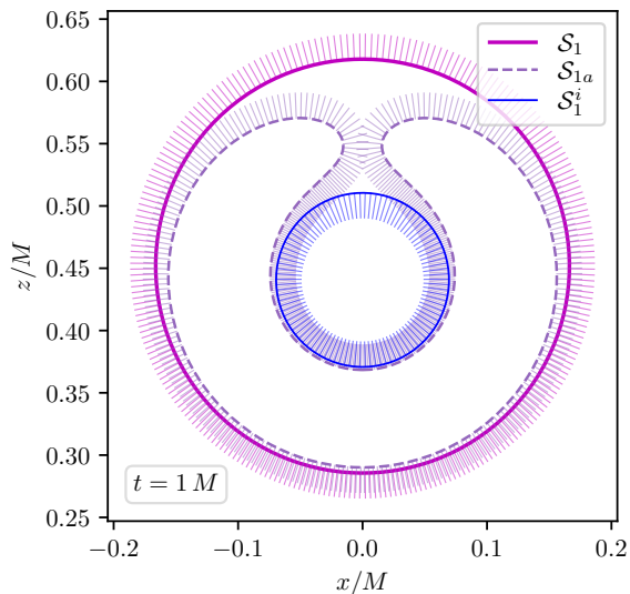
FIG. 12. Spatial outward normal directions on \mathcal{S}_1 and one of the interior MOTSs \mathcal{S}_{1a} as well as the inward normal direction on the MITS \mathcal{S}_1^i .
