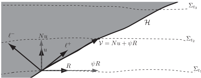
FIG. 2. Definition of the evolution vector \mathcal{V} along a MOTT \mathcal{H} . \mathcal{V} can be split into a component \psi R orthogonal to \mathcal{S} = \mathcal{H} \cap \Sigma_{t_1} within \Sigma_{t_1} and one orthogonal to \Sigma_{t_1} , i.e. Nu , which is also orthogonal to \mathcal{S} .
