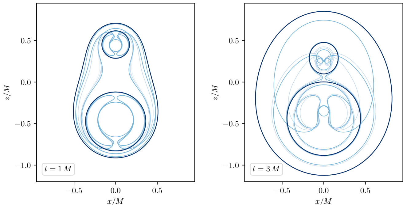
FIG. 16. MOTSs at two different times of the simulation. The line thickness and color reflects N_-^0 , i.e. the number of negative stability eigenvalues of the m = 0 mode. The three dark lines in both panels are \mathcal{S}_{\text{outer}} (common), \mathcal{S}_1 (upper) and \mathcal{S}_2 (lower). Lighter colors show MOTSs with larger N_-^0 . Note that none of the MOTSs extends beyond \mathcal{S}_{\text{outer}} .
