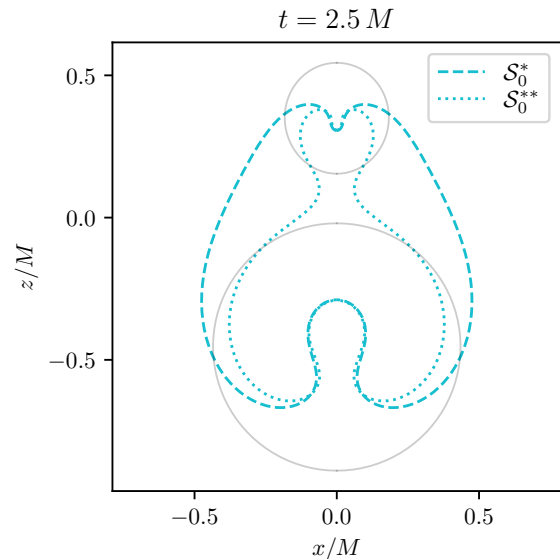
FIG. 7. Examples of the MOTSs \mathcal{S}_0^* and \mathcal{S}_0^{**} at simulation time t = 2.5M . The light grey curves show \mathcal{S}_1 and \mathcal{S}_2 for reference.
