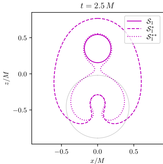
FIG. 6. Examples of the MOTSs \mathcal{S}_1 , \mathcal{S}_1^* , and \mathcal{S}_1^{**} at simulation time t = 2.5M . The light grey curve shows \mathcal{S}_2 for reference.
