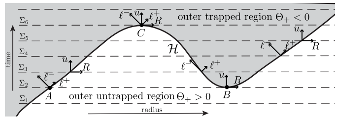
FIG. 1. Spherically symmetric evolution of a MOTT \mathcal{H} (thin solid line). It is perfectly possible for \mathcal{H} to weave back and forth through the time foliation. See, for example, [20, 21] for exact solutions exhibiting this behaviour.
