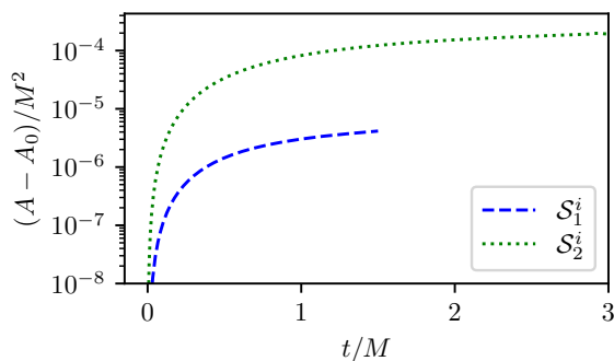
FIG. 13. Evolution of the area of the MITSs \mathcal{S}_1^i and \mathcal{S}_2^i . We plot the difference A - A_0 on a logarithmic scale to emphasize the area change. Here A_0 is the area of the MITS at t = 0 where it coincides with the area of \mathcal{S}_1 and \mathcal{S}_2 , respectively.
