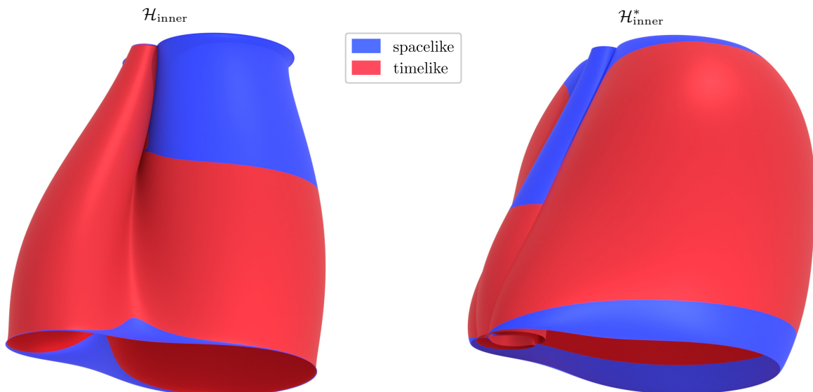
FIG. 18. Signature of \mathcal{H}_{\text{inner}} (left panel) and \mathcal{H}_{\text{inner}}^* (right panel). In these tube plots, time goes upwards and z -values increase to the left. These two MOTTs smoothly connect at their top ends but not at the bottom as they connect with different world tubes there. The bottom end of the right panel corresponds to the bottom-left panel of FIG. 4.
