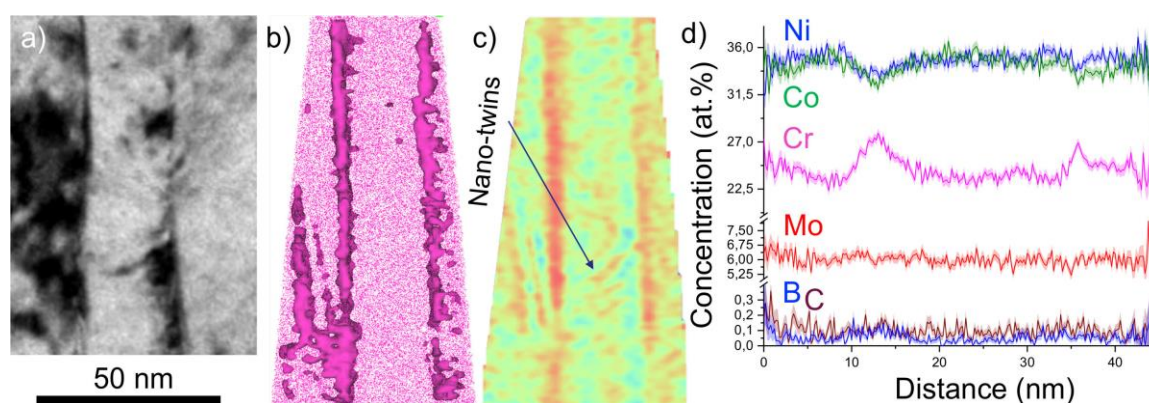
Figure 1. (a) Bright-field TEM micrograph showing a representative micro-twin, (b) 3D reconstruction of the Cr atoms along with 12.55 \text{ \#/nm}^3 Cr isodensity surfaces representing the fault planes of a sample aged at 500^\circ\text{C} for 30 min, (c) 2D Cr concentration map showing the presence of nano-twins within the micro-twin, and (d) Concentration profile across the fault planes showing. Error bars are shown as lines filled with color and correspond to the 2\sigma counting error.
