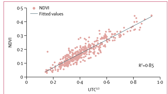
Figure 3: Scatterplot of 2014 NDVI scores versus tree canopy cover values NDVI=Normalized Difference Vegetation Index. UTC=percent of pixels within each census tract that were tree canopy.
